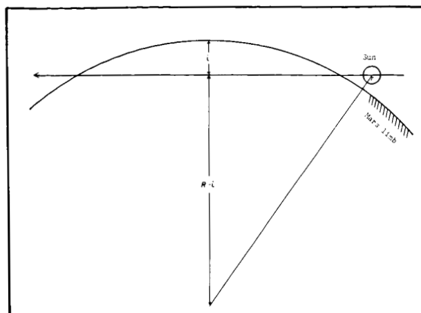
Figure 4. The solar eclipse by Mars as seen from Phobos.
