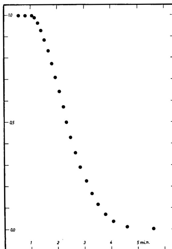
Figure 5. Computed light curve of Phobos for i = r when effects of Martian atmosphere are neglected.
