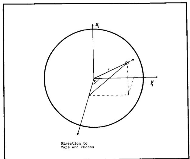
Figure 3. Geometrical relations pertaining to the brightness of solar segments.
