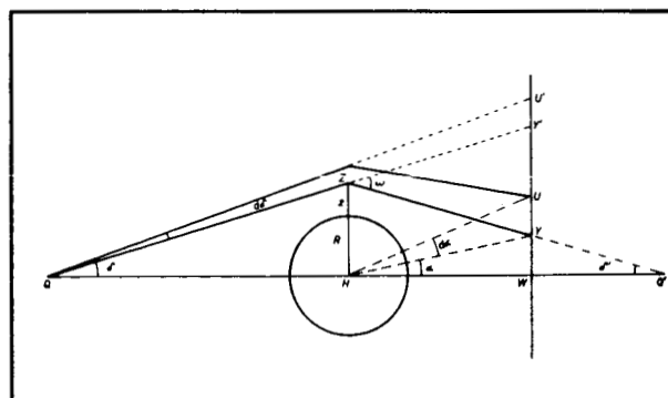
Figure 8. Geometrical relations for the calculation of the loss of light caused by the refraction of the sunlight as it passes through the Martian atmosphere.
