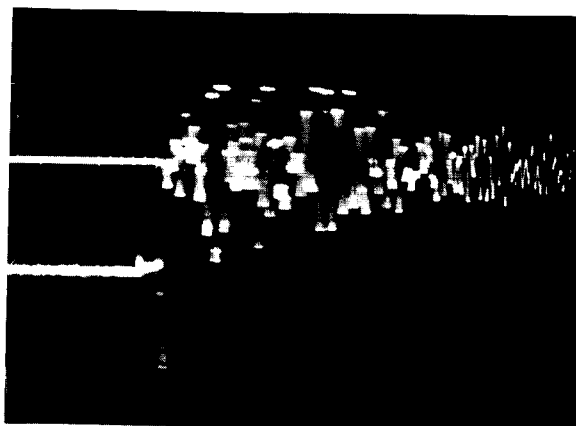
FIGURE 2-14 IMPACT TEST NO. 5 (Channels #1, 2, 3) 2 February, 1966 - Shot #1 PROJECTILE: LEXAN SLUG (2.8 mg)
