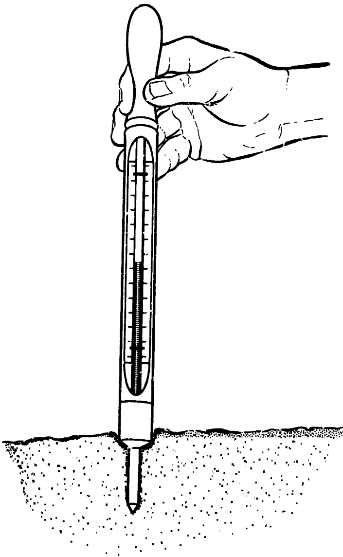
Fig. A-5. Brass-tipped soil thermometer constructed for in situ soil temperature measurements
