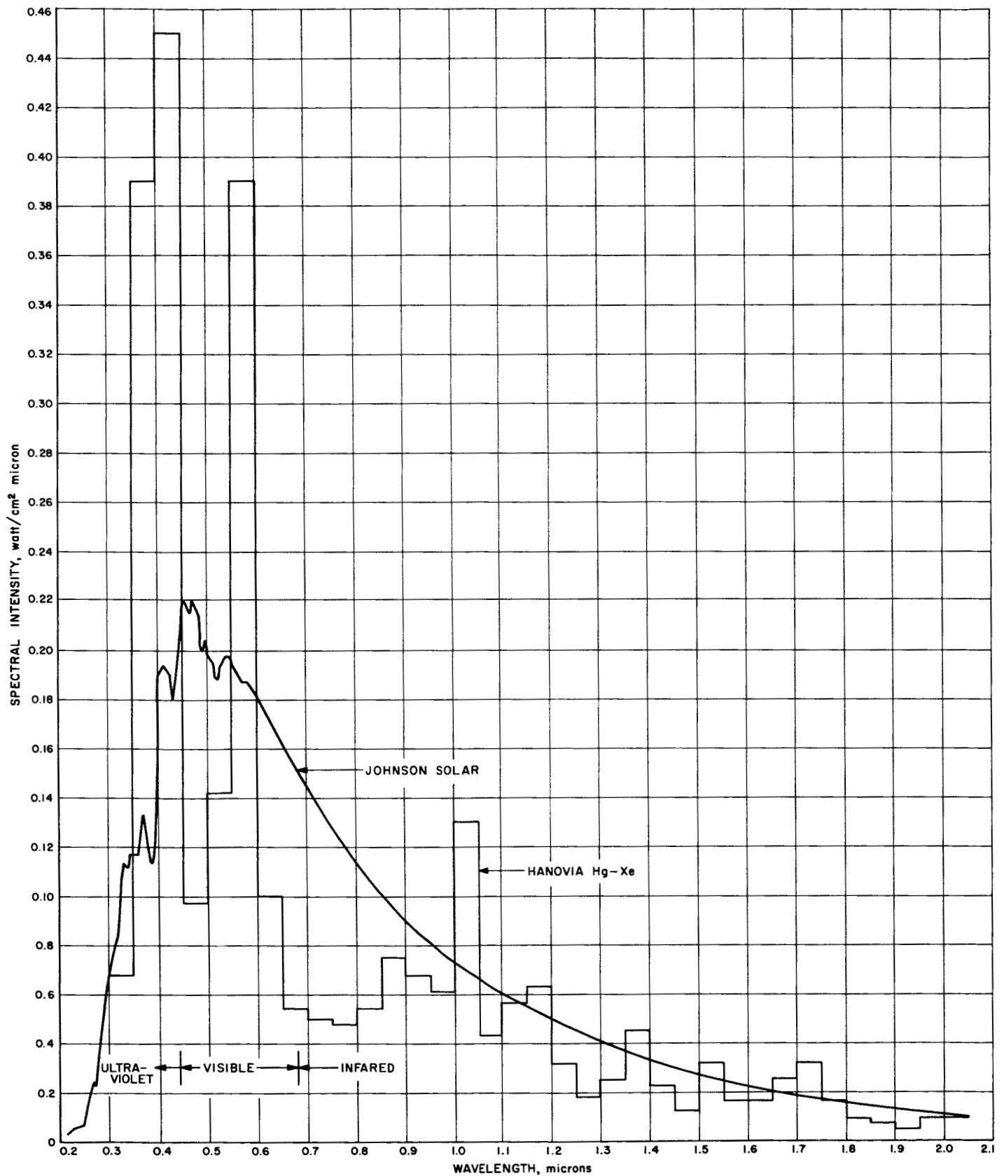
Fig. 3. Solar constant
