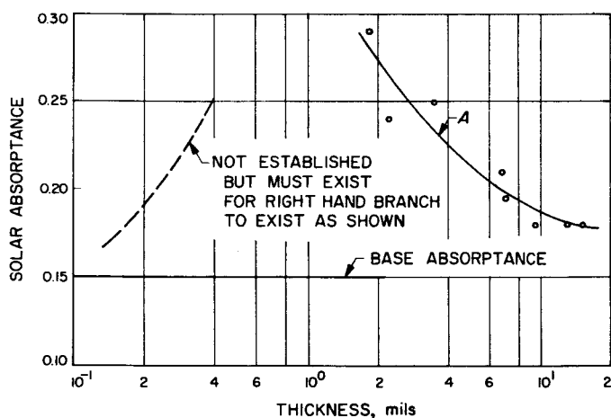
Fig. 10. Solar absorptance vs thickness (white paint)
