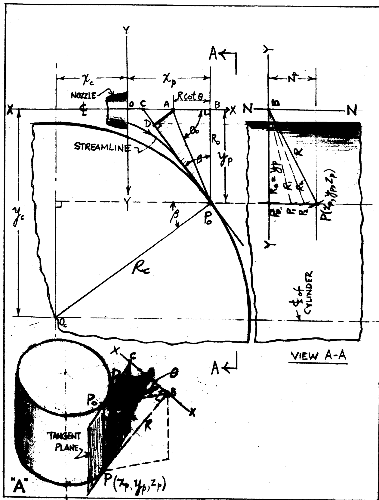
Fig. 5 Geometry of Impingement of Plume Streamline on Convex Cylinder at Right Angles to Plume Axis
