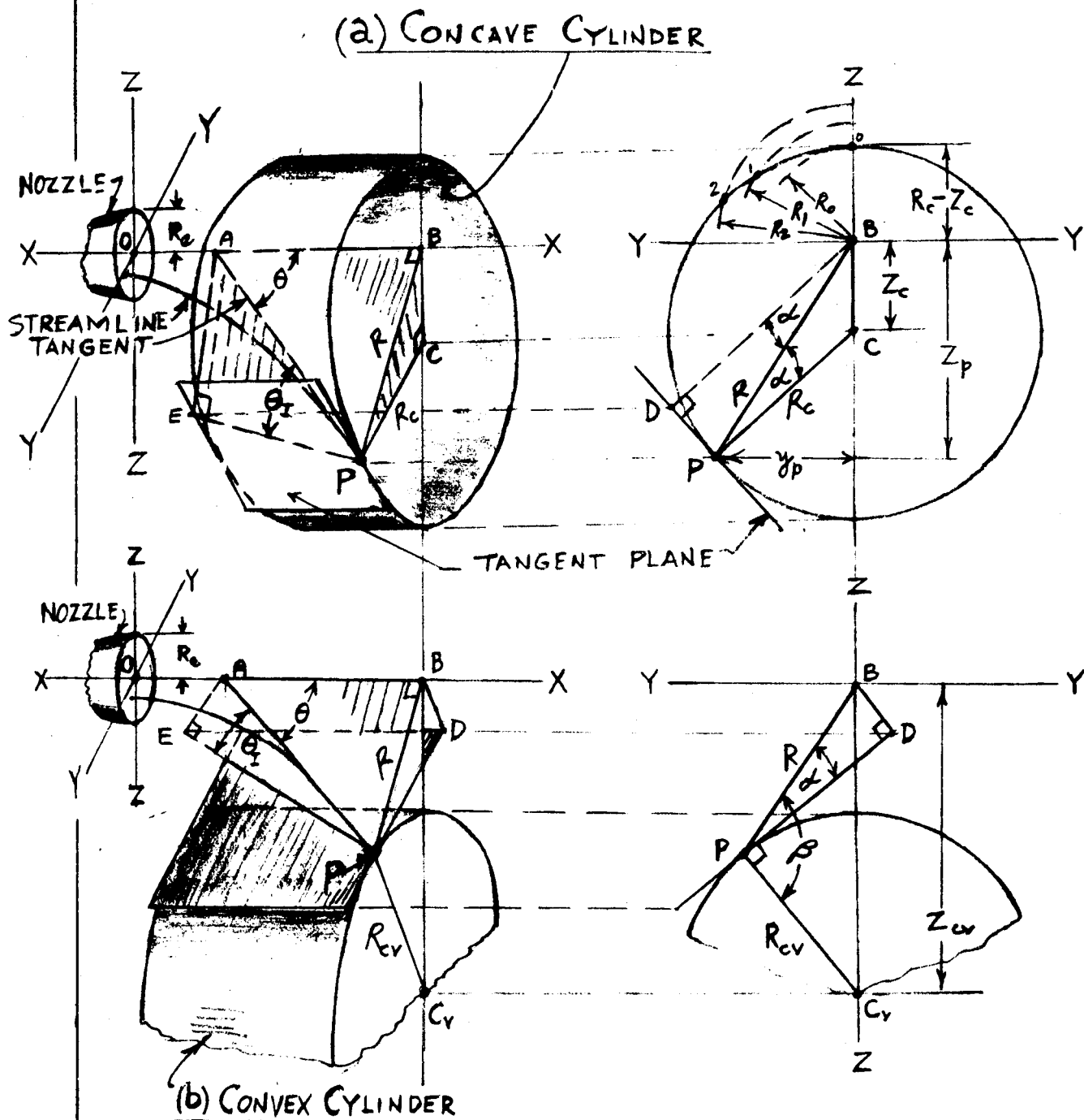
Fig.3 Geometry of Impingement of Plume Streamline on Concave and Convex Cylinders Parallel to Plume
