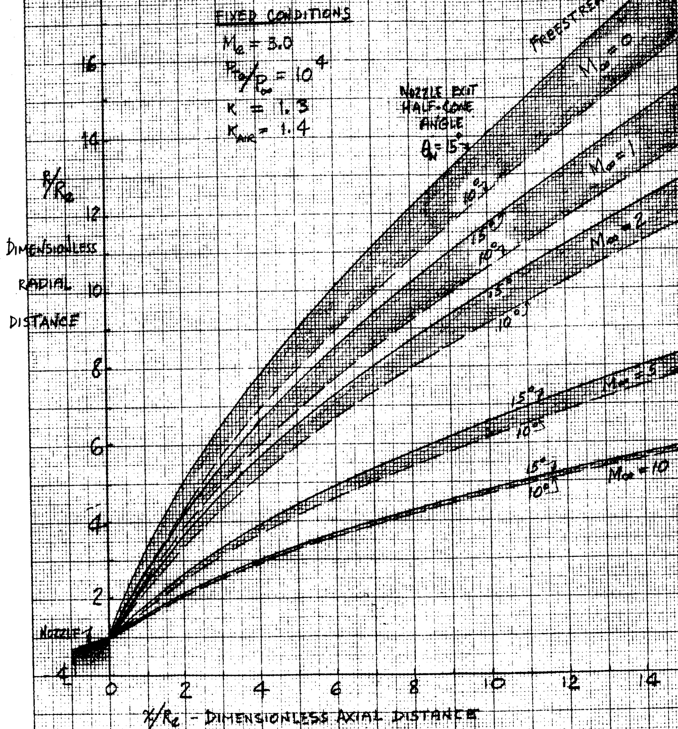
Fig. 2 Effect of Freestream Mach No. and Nozzle Exit Angle on Jet Plume Boundary
