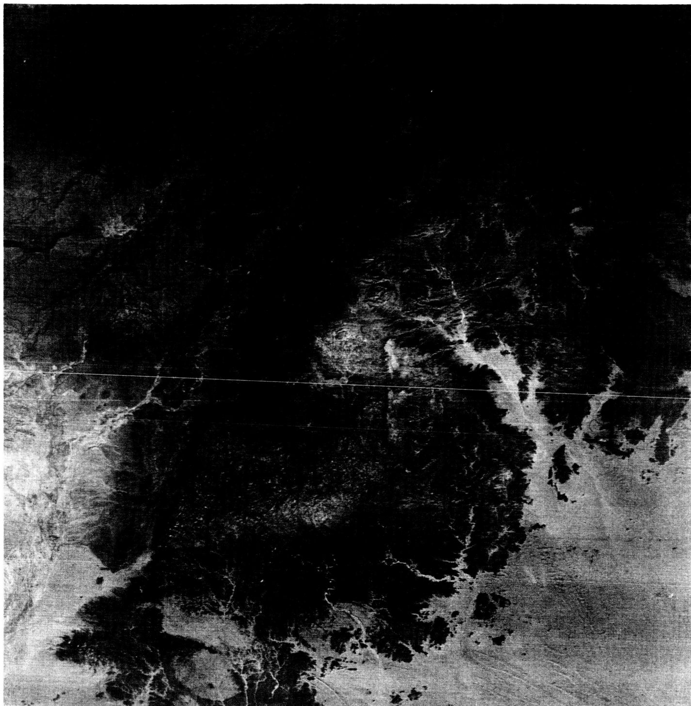
Fig. 7 Mountains in southwestern part of Arabian Peninsula; Empty Quarter at lower right. Chiefly Precambrian crystalline rocks, considerably jointed and faulted.
