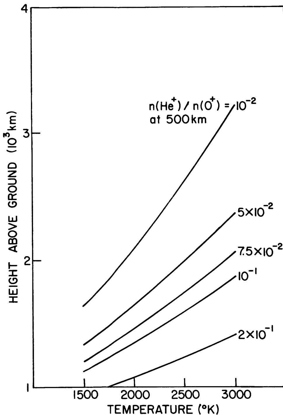
FIG. 5. TRANSITION LEVELS BETWEEN \text{He}^+ AND \text{O}^+ FOR DIFFERENT COMPOSITIONS AT THE BASE LEVEL (500 KM).
