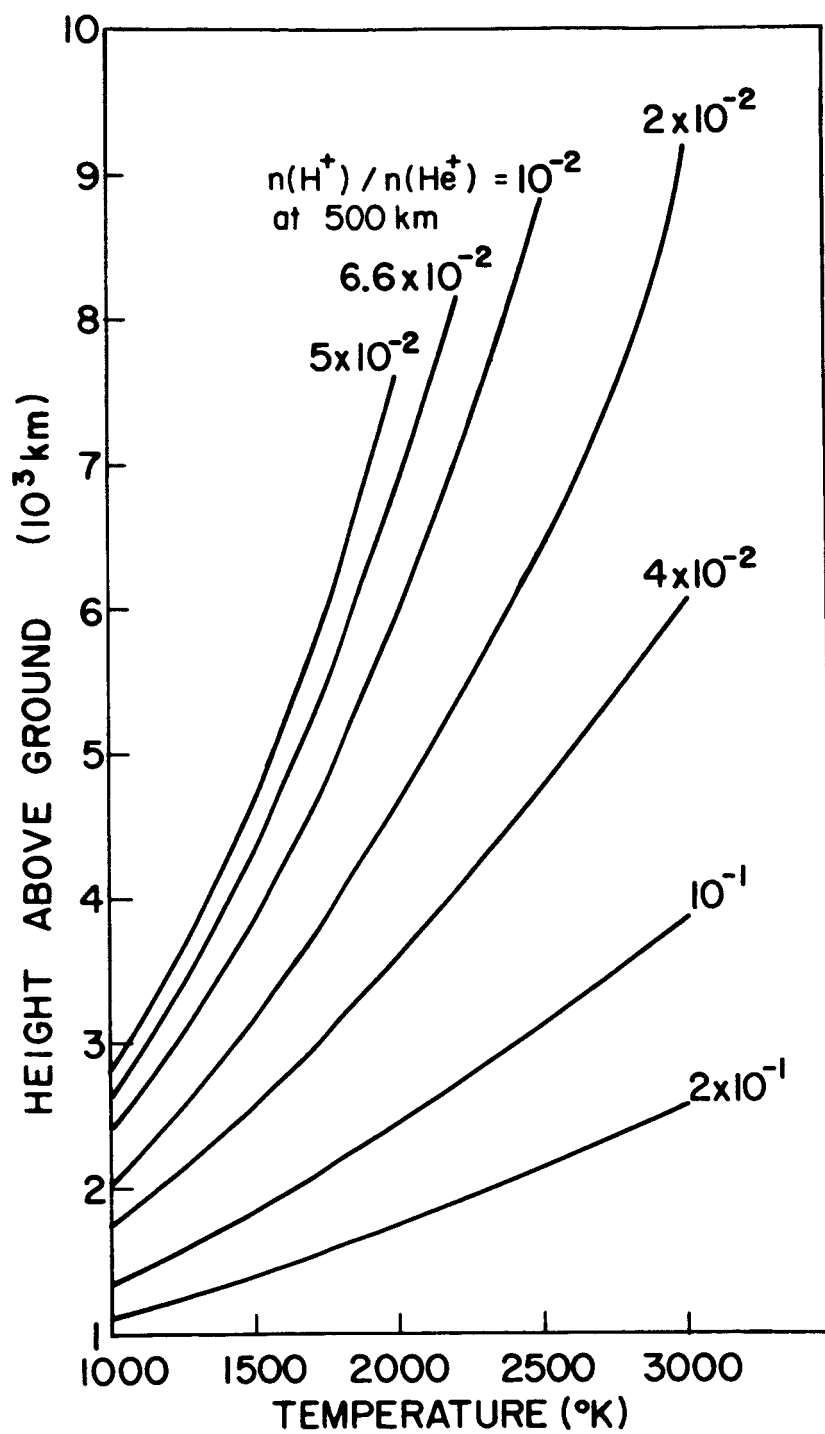
FIG. 6. TRANSITION LEVELS BETWEEN H^+ AND He^+ FOR DIFFERENT COMPOSITIONS AT BASE LEVEL (500 KM).
