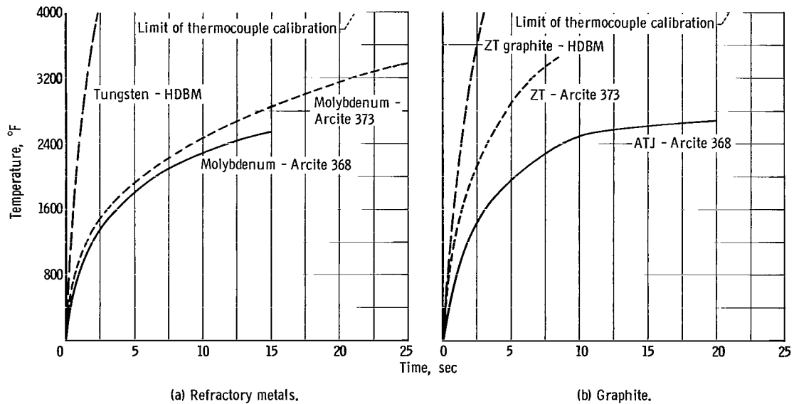
Figure 7. - Nozzle-insert temperature-time curves. Thermocouple junction, 0.05 inch from nozzle throat surface.
