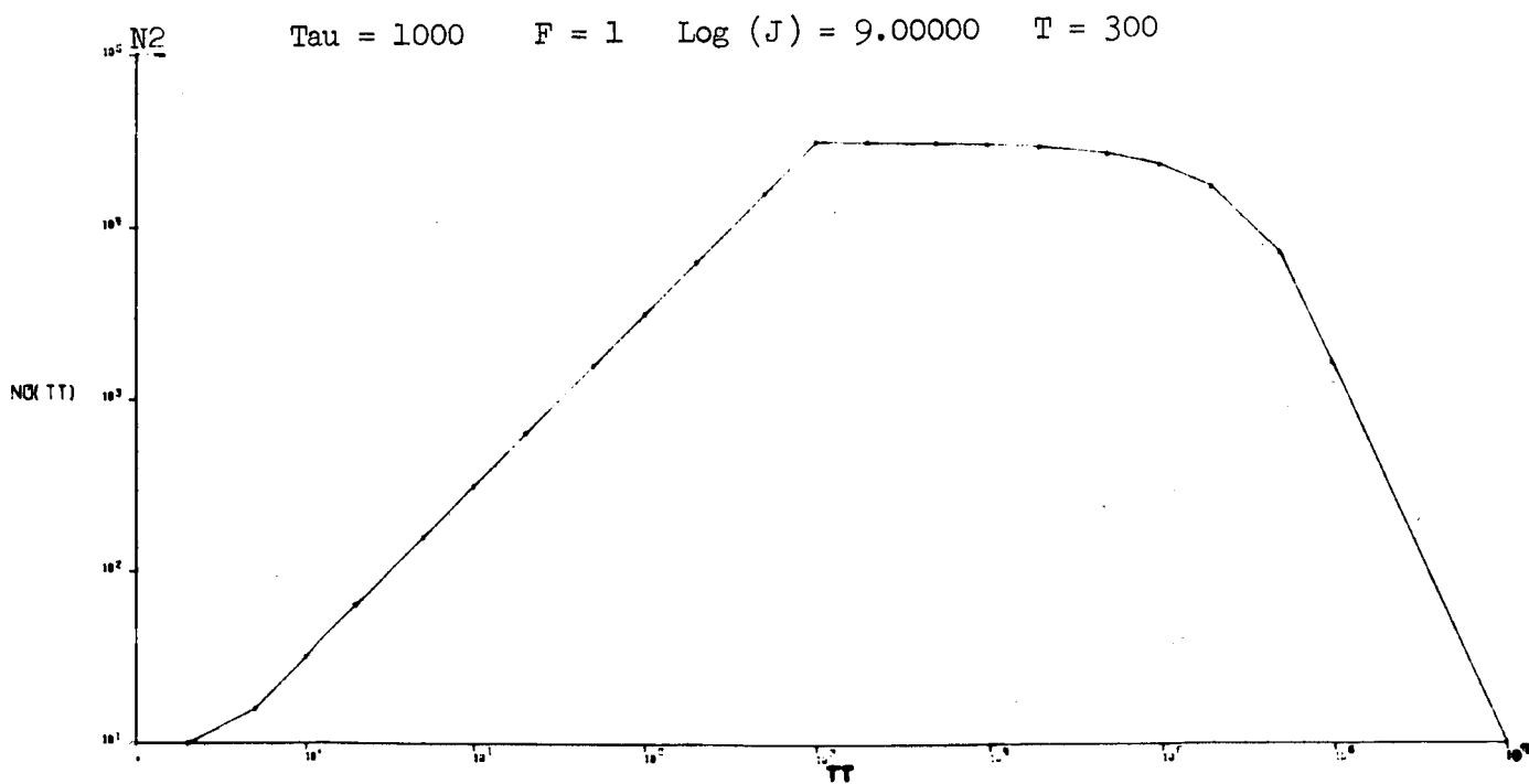
Fig. 15 Model I - N_2 Variation of LEM Exhaust Contamination With Time (Number of Particles/cm 3 versus Time in Seconds)
