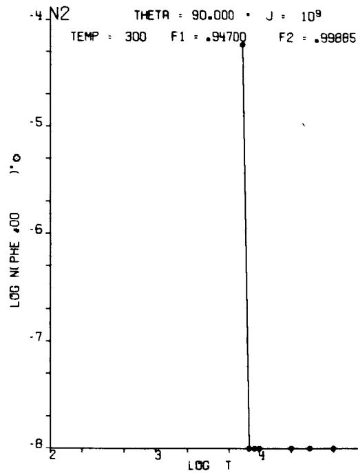
Fig. 52 Model II - N 2 Variation of LEM Exhaust Contamination with Time at 2700 km from LEM Touchdown F_1 = 0.947 , F_2 = 0.99885
