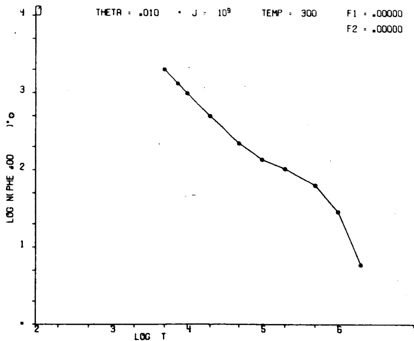
Fig. 49 Model II - O Variation of LEM Exhaust Contamination with Time at 300 Meters from LEM Touchdown F_1 = 0 , F_2 = 0
