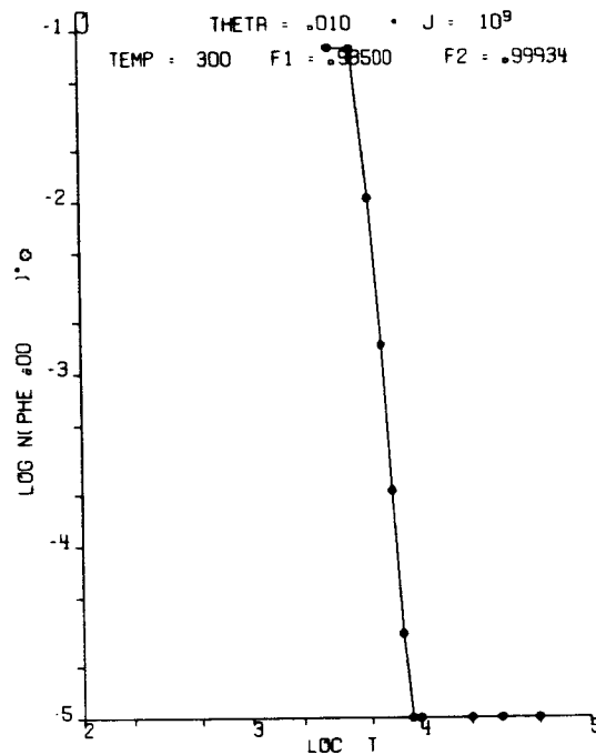
Fig. 48 Model II - O Variation of LEM Exhaust Contamination with Time at 300 Meters from LEM Touchdown F_1 = 0.985 , F_2 = 0.99934
