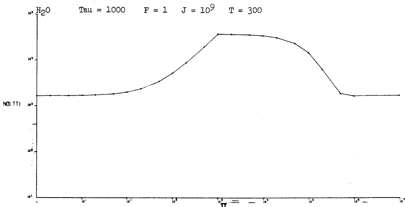
Fig. 14 Model I - H_2O Variation of LEM Exhaust Contamination With Time (Number of Particles/cm 3 versus Time in Seconds)
