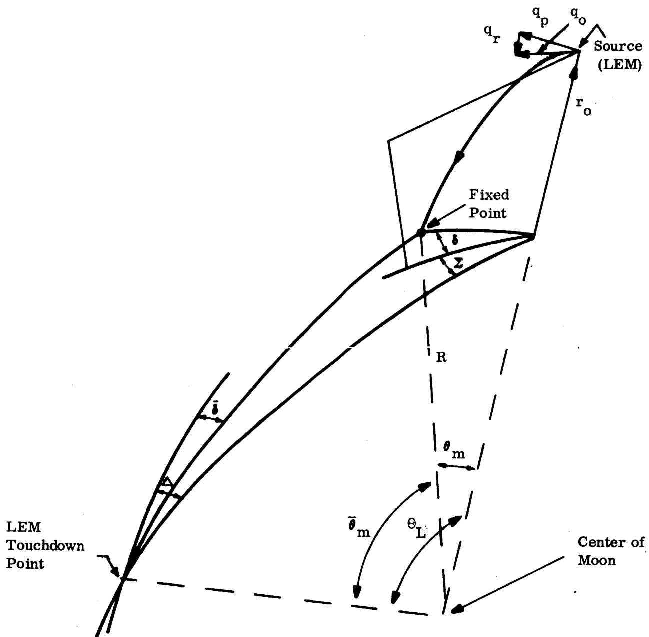
Fig. 4 Coordinate Systems
