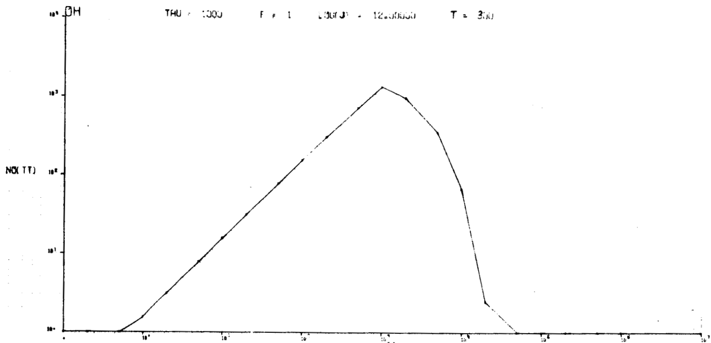
Fig. 30 Model I - OH Variation of LEM Exhaust Contamination With Time (Number of Particles/cm 3 versus Time in Seconds)
