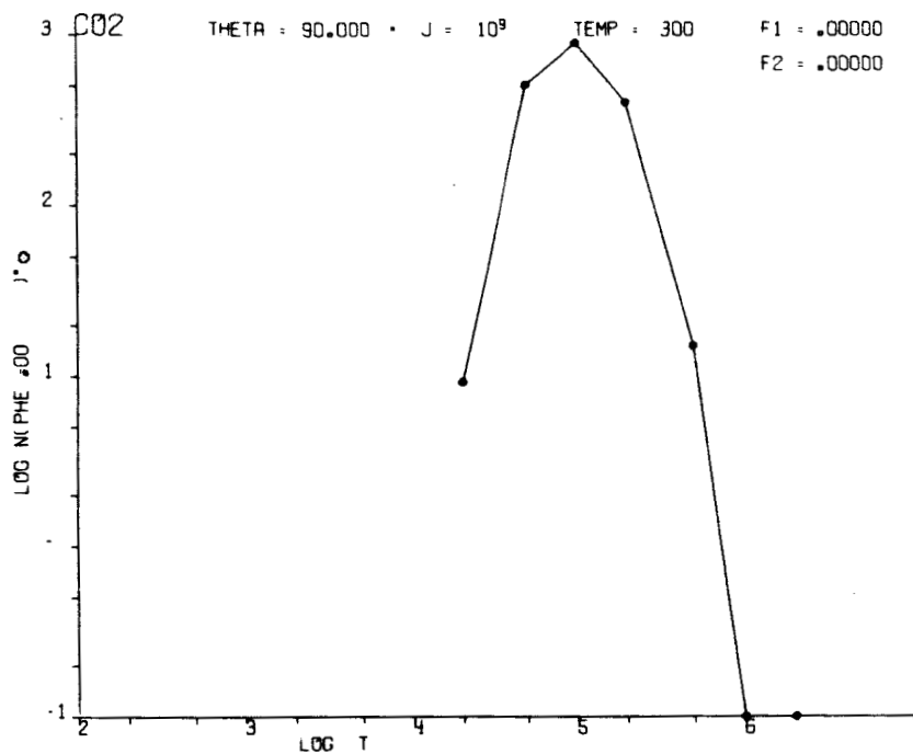
Fig. 56 Model II - CO 2 Variation of LEM Exhaust Contamination with Time at 2700 km from LEM Touchdown F 1 = 0, F 2 = 0
