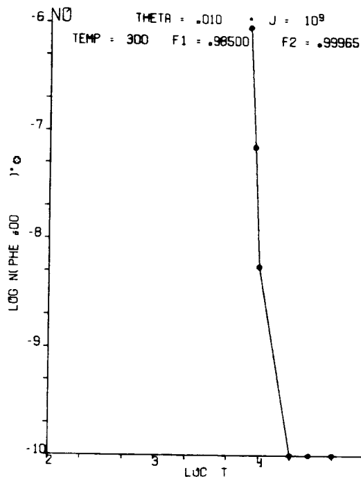
Fig. 44 Model II - NO Variation of LEM Exhaust Contamination with Time at 300 Meters from LEM Touchdown F_1 = 0.985 , F_2 = 0.99965
