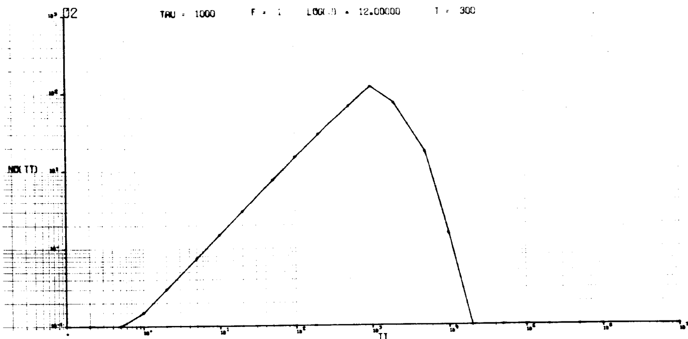
Fig. 32 Model I - O 2 Variation of LEM Exhaust Contamination With Time (Number of Particles/cm 3 versus Time in Seconds)
