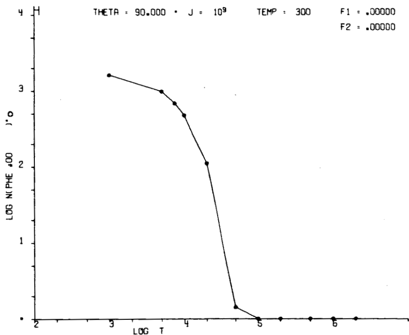
Fig. 57 Model II - H Variation of LEM Exhaust Contamination with Time at 2700 km from LEM Touchdown F 1 = 0, F 2 = 0
