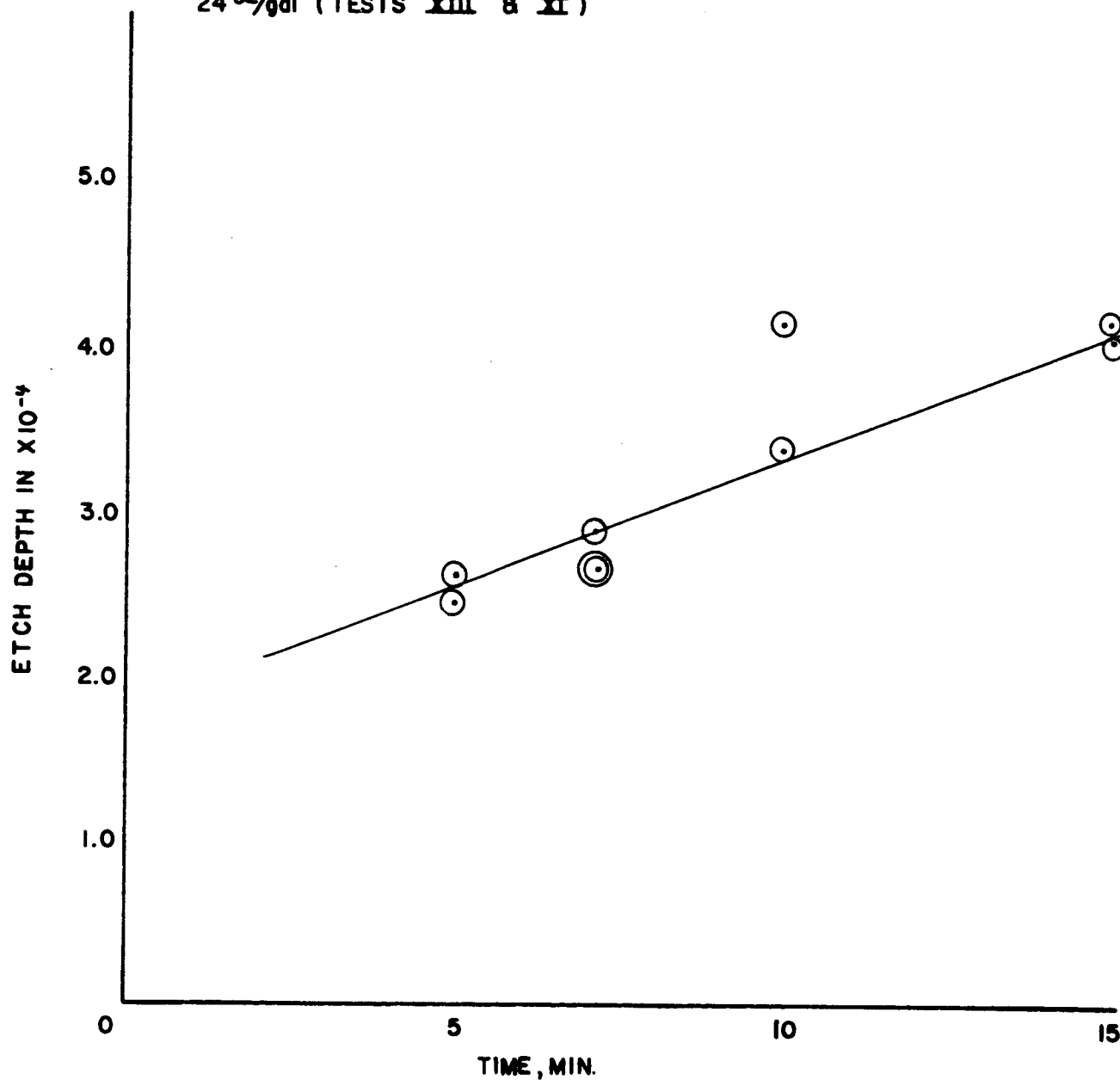
ETCH DEPTH VS TIME FOR MANUALLY APPLIED TURCO 13-B AT 24 oz/gal (TESTS XIII & XI)
