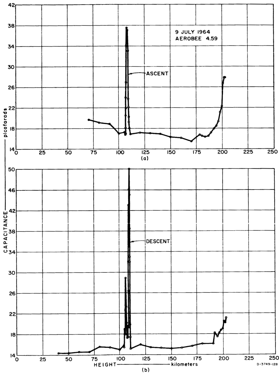
FIG. 19. IMPEDANCE PROBE CAPACITANCE DATA, 1.54 KC. (Courtesy of L. E. Orsak, L. H. Rorden, G. B. Carpenter and B. P. Ficklin, Stanford Research Institute, Final Rept., Contract NASr-49(01), Jan 1965.)
