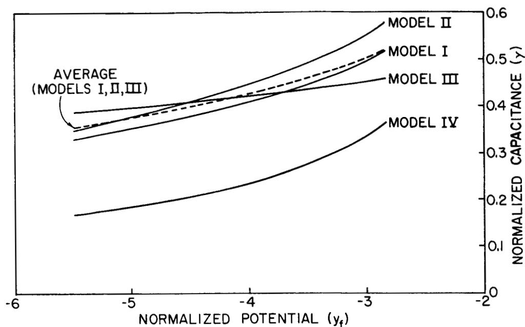
FIG. 7. NORMALIZED SHEATH CAPACITANCE FOR DIFFERENT MODELS, PLANAR GEOMETRY.
