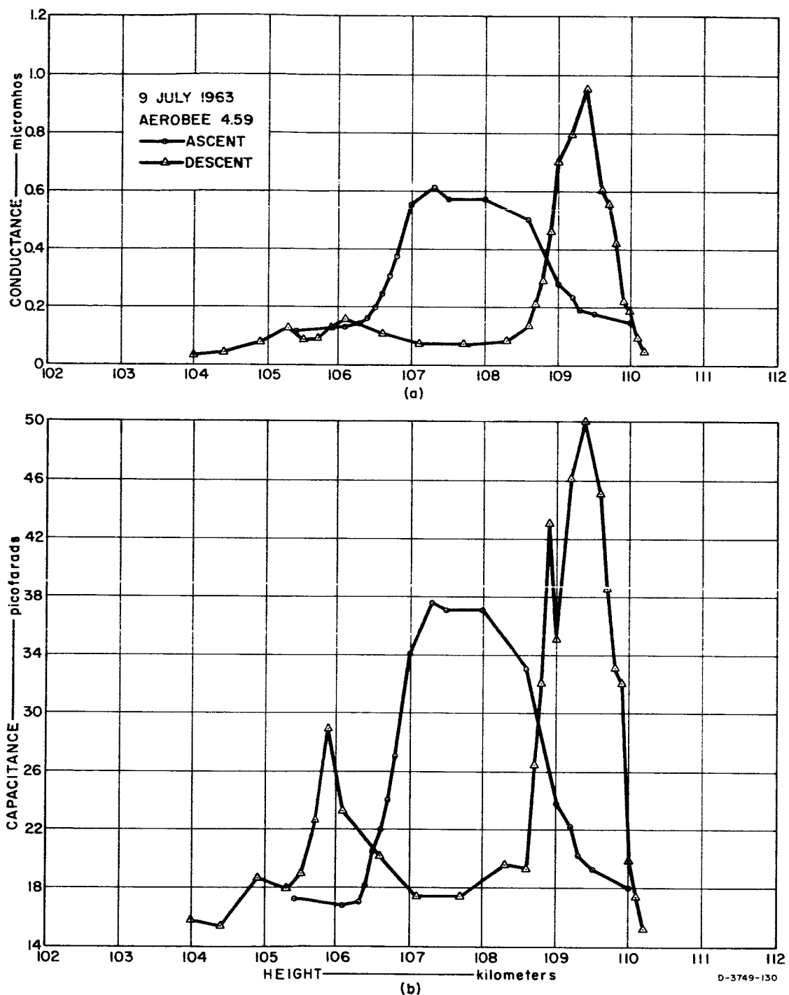
FIG. 21. IMPEDANCE PROBE CONDUCTANCE AND CAPACITANCE IN THE SPORADIC E LAYER. (Courtesy of L. E. Orsak, L. H. Rorden, G. B. Carpenter and B. P. Ficklin, Stanford Research Institute, Final Rept., Contract NASr-49(01), Jan 1965.)
