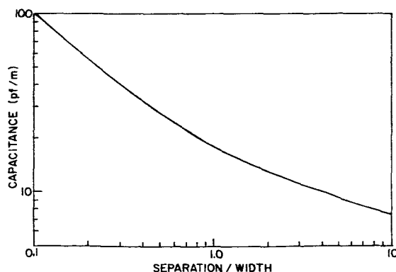
FIG. 24. CAPACITANCE OF TWO LONG PARALLEL STRIPS IN FREE SPACE.
