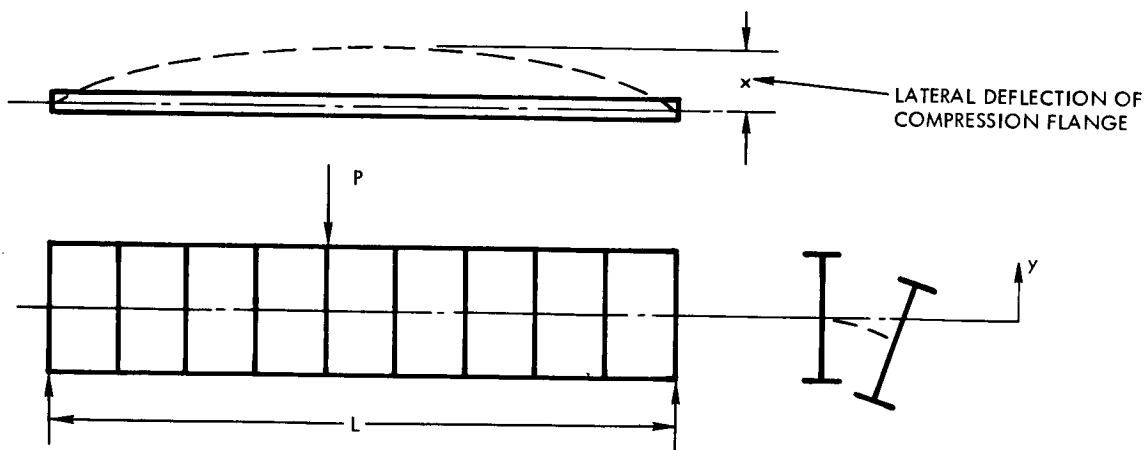
Figure 70. Determination of the Allowable Flexural Compressive Stress
