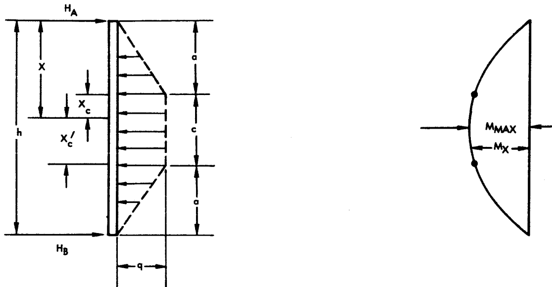
Figure 33. Upright Reaction
