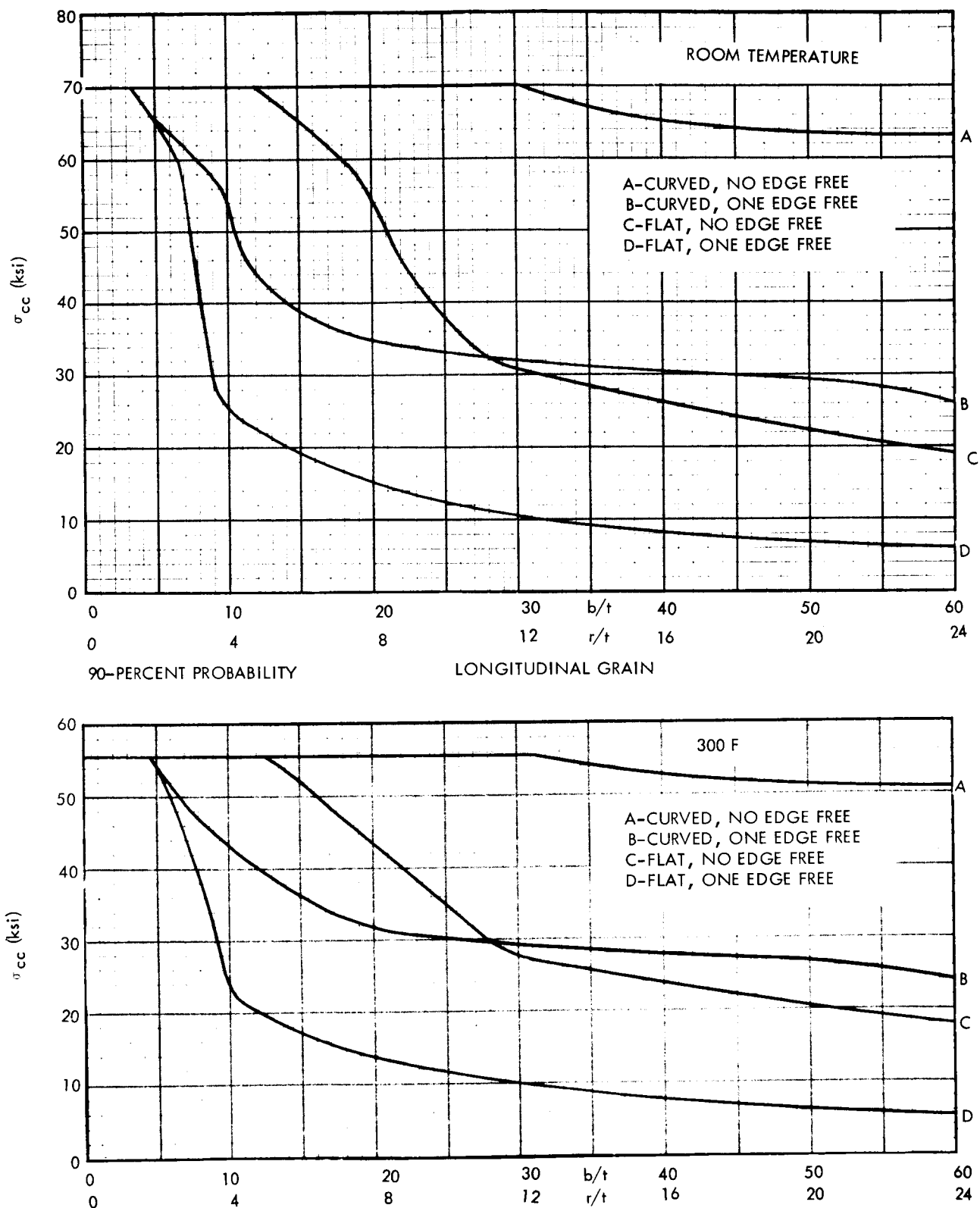
Figure 20. Ultimate Element Crippling Curves for Bare 7075-T6 Aluminum Alloy Sheet (Room Temperature, 300 F)
