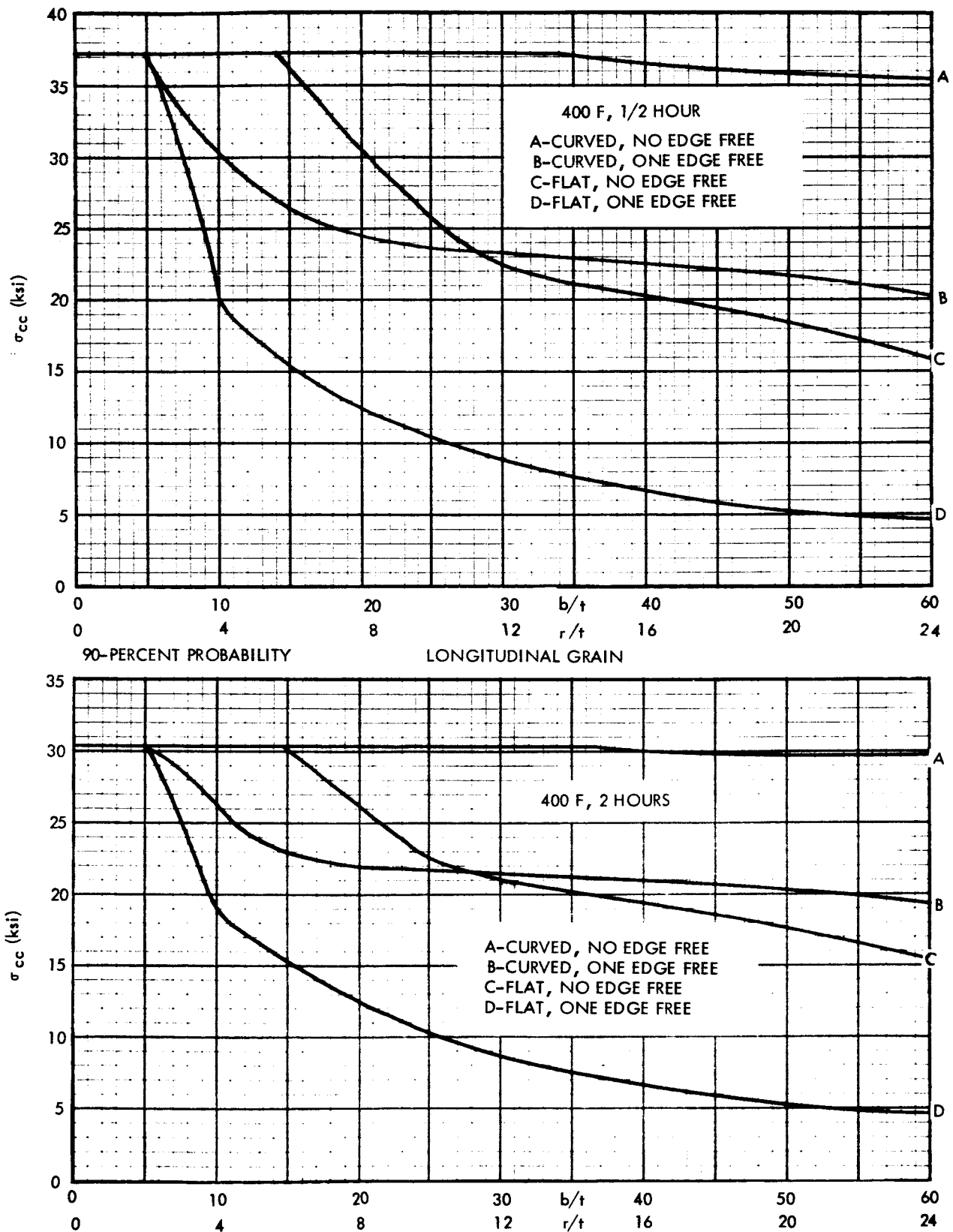
Figure 21. Ultimate Element Crippling Curves for Bare 7075-T6 Aluminum Alloy Sheet (400 F)
