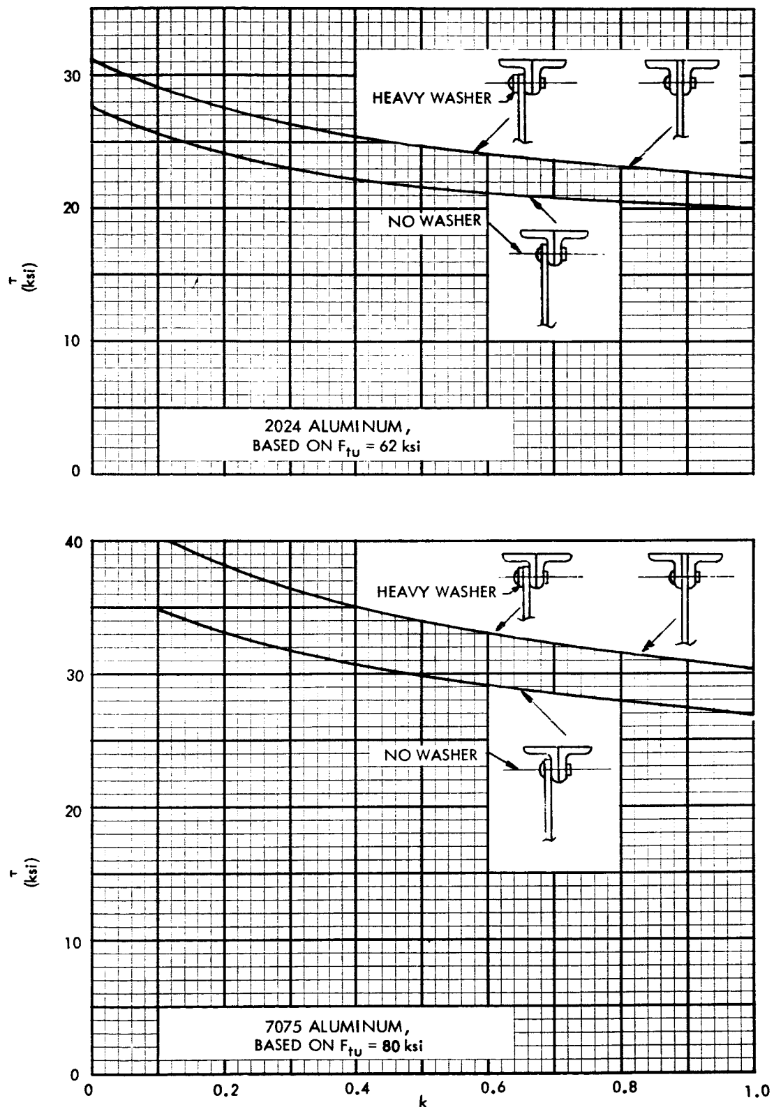
Figure 16. Allowable Web Stresses for 2024 and 7075 Aluminum at Room Temperature
