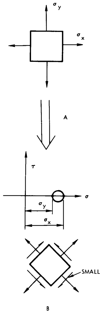
Figure 40. Stresses Due to Lateral Loading
