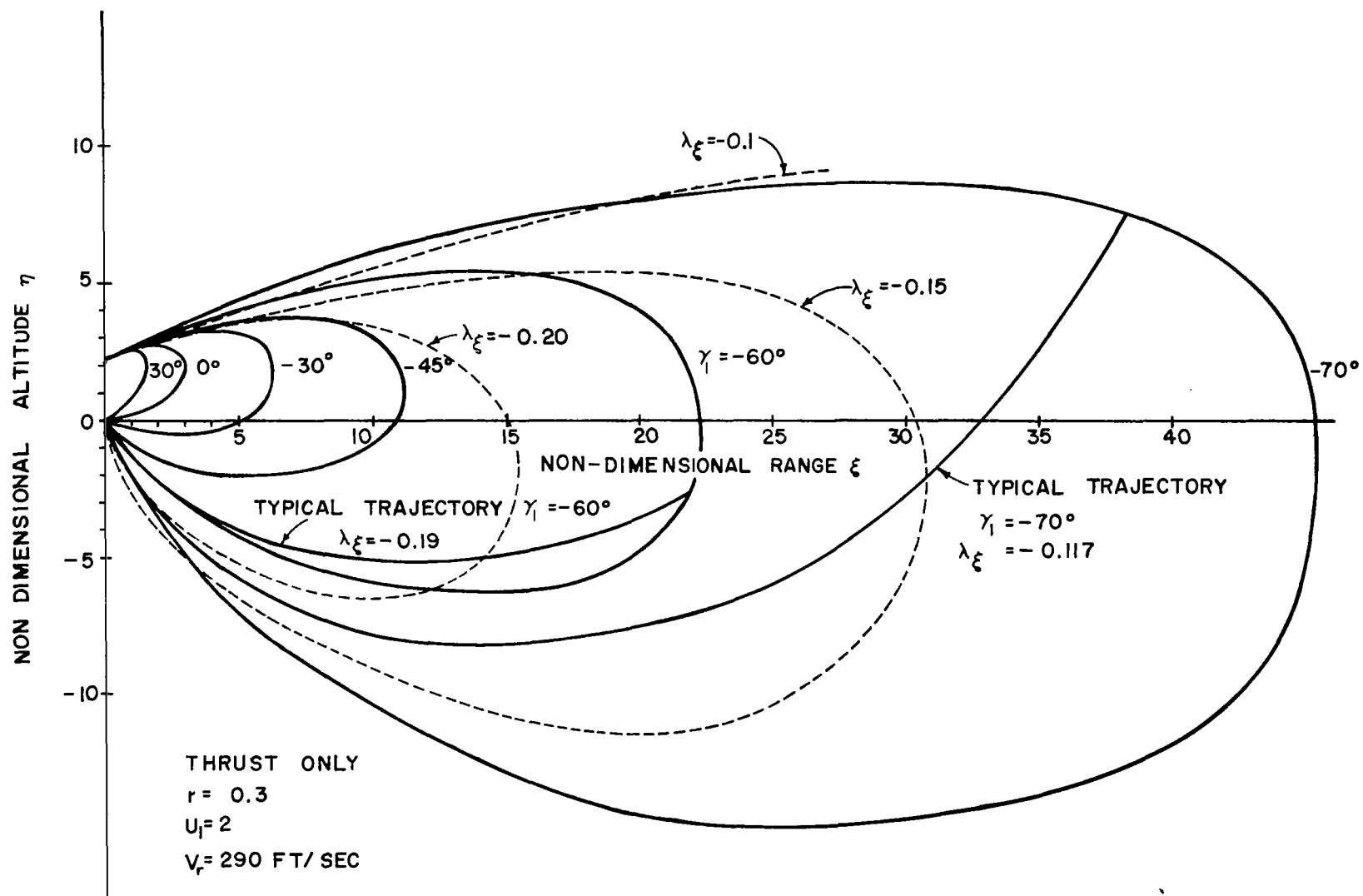
FIGURE 2— LOCUS OF OPTIMAL ENDPOINTS (THRUST ONLY)
