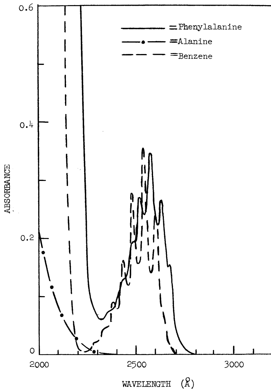
FIG. 1--Structure of longest wavelength UV absorption band of DL-phenylalanine and benzene in dilute aqueous solution ( 1.75 \times 10^{-3} M) . The absorption of an equimolar solution of DL-alanine is included for comparison. Spectra were measured on a Cary model 14M recording spectrophotometer using 1 cm fused silica cuvettes.
