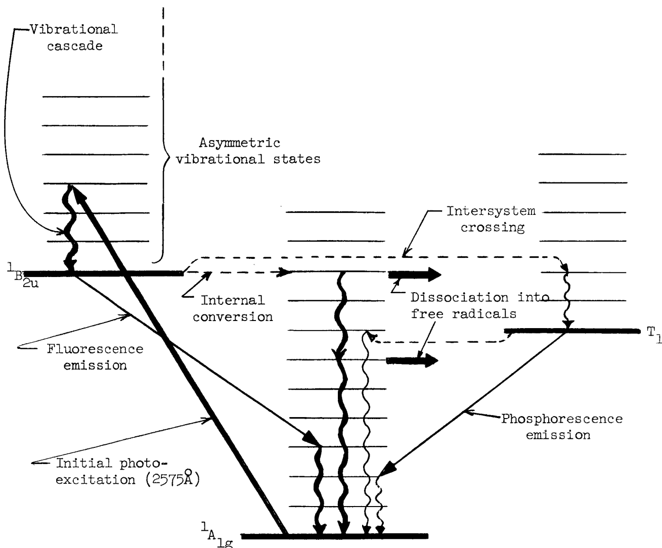
FIG. C.1.--Pathways of de-excitation of the lowest lying ( 1B_{2u} ) singlet excited state of DL-phenylalanine. The above energy level diagram is a modified version of the general scheme of Hammond and Turro (1963). The levels designated 1A_{1g} and T_1 are the ground and lowest lying triplet states, 1g respectively. The series of levels above each electronic state represent vibrational states. Rotational levels have been omitted for the sake of clarity.
