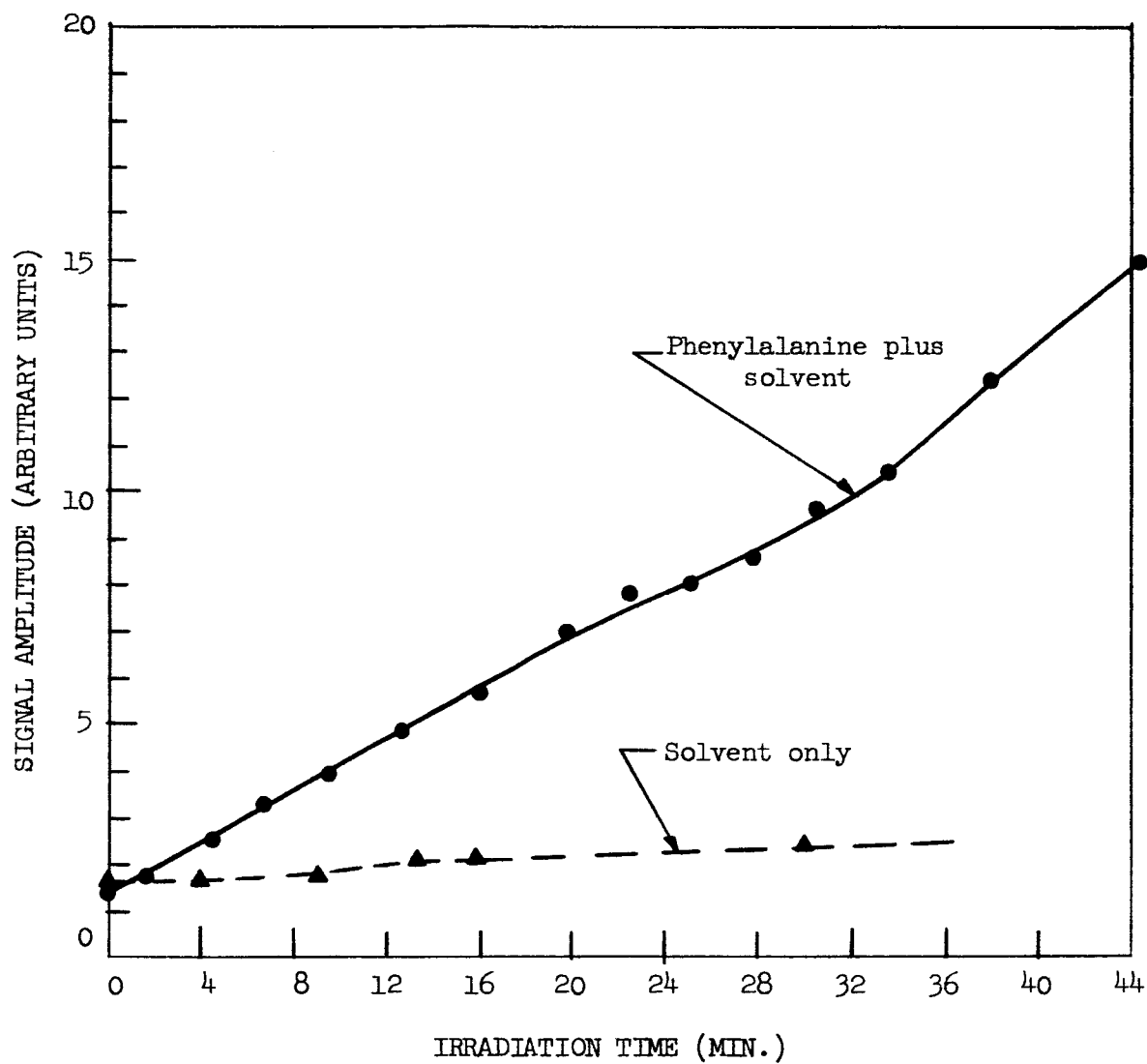
FIG. 19--Rate of increase in amplitude of the phenylalanine low temperature e.s.r. signal during UV-irradiation. Experimental conditions are given in the legend to Fig. 17.
