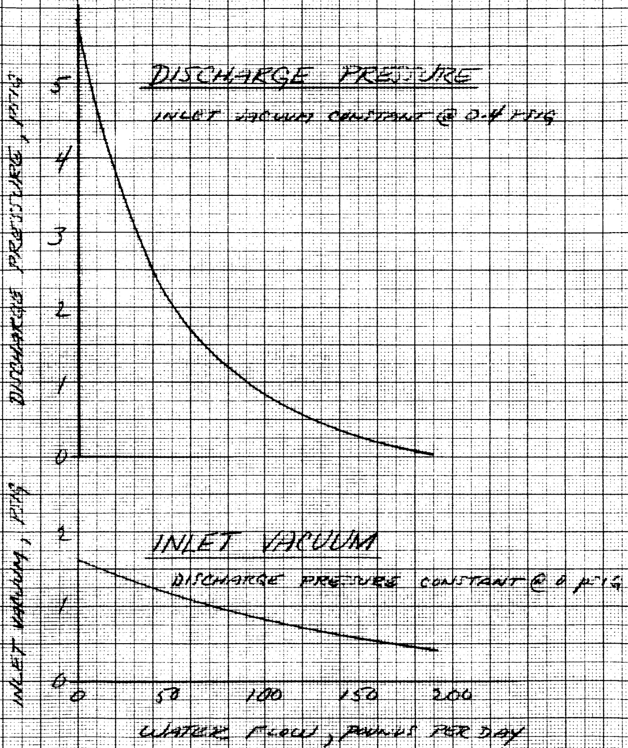
Figure 6. TFW Pump Capacity
