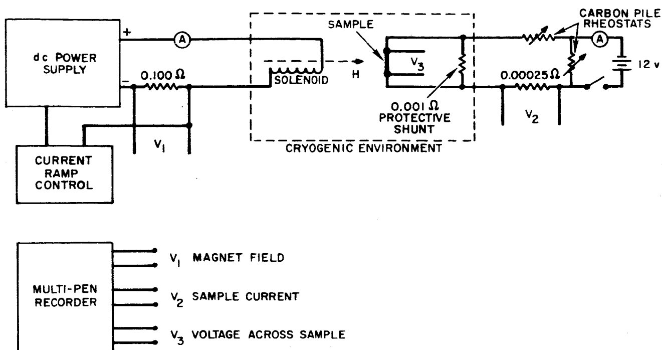
Figure 1. Experimental Circuitry
