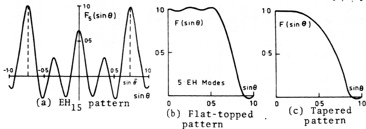
Fig. 3 Pattern syntheses with hybrid modes
