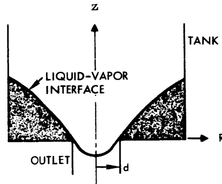
FIGURE 2. — Free Surface Configuration at Vapor Ingestion
