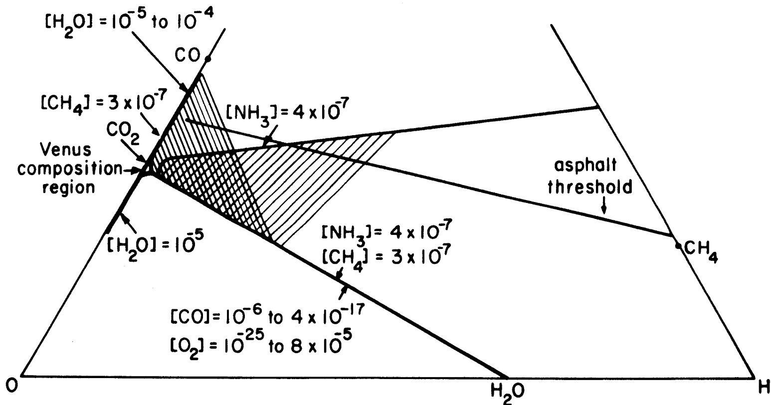
Fig. 1.--C-H-O ternary diagram for the Cytherean atmosphere. The shaded regions are excluded at thermodynamic equilibrium by the observational upper limits on [CH 4 ] and [NH 3 ]. For clarity the shading has not been extended through the entire excluded region. The adopted values of [H 2 O] and the observed upper limits on [CO] and [O 2 ] are denoted by lines.
