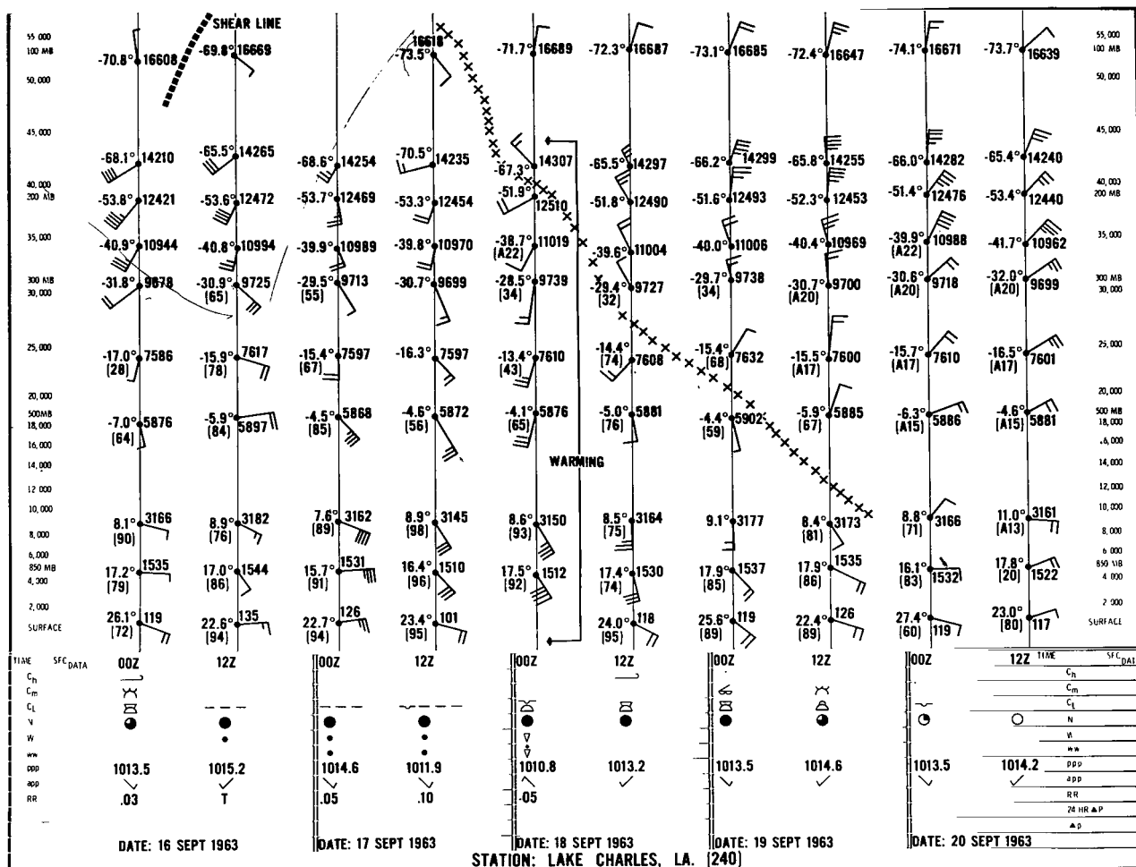
Figure 17-A time cross-section for Lake Charles, Louisiana during the period 16-20 September 1963. The symbol (XXXX) indicates the edge of the ridge line aloft as Hurricane Cindy moved over Lake Charles. The passage of an upper level shear line (—) is indicated on 16 September 1963.
