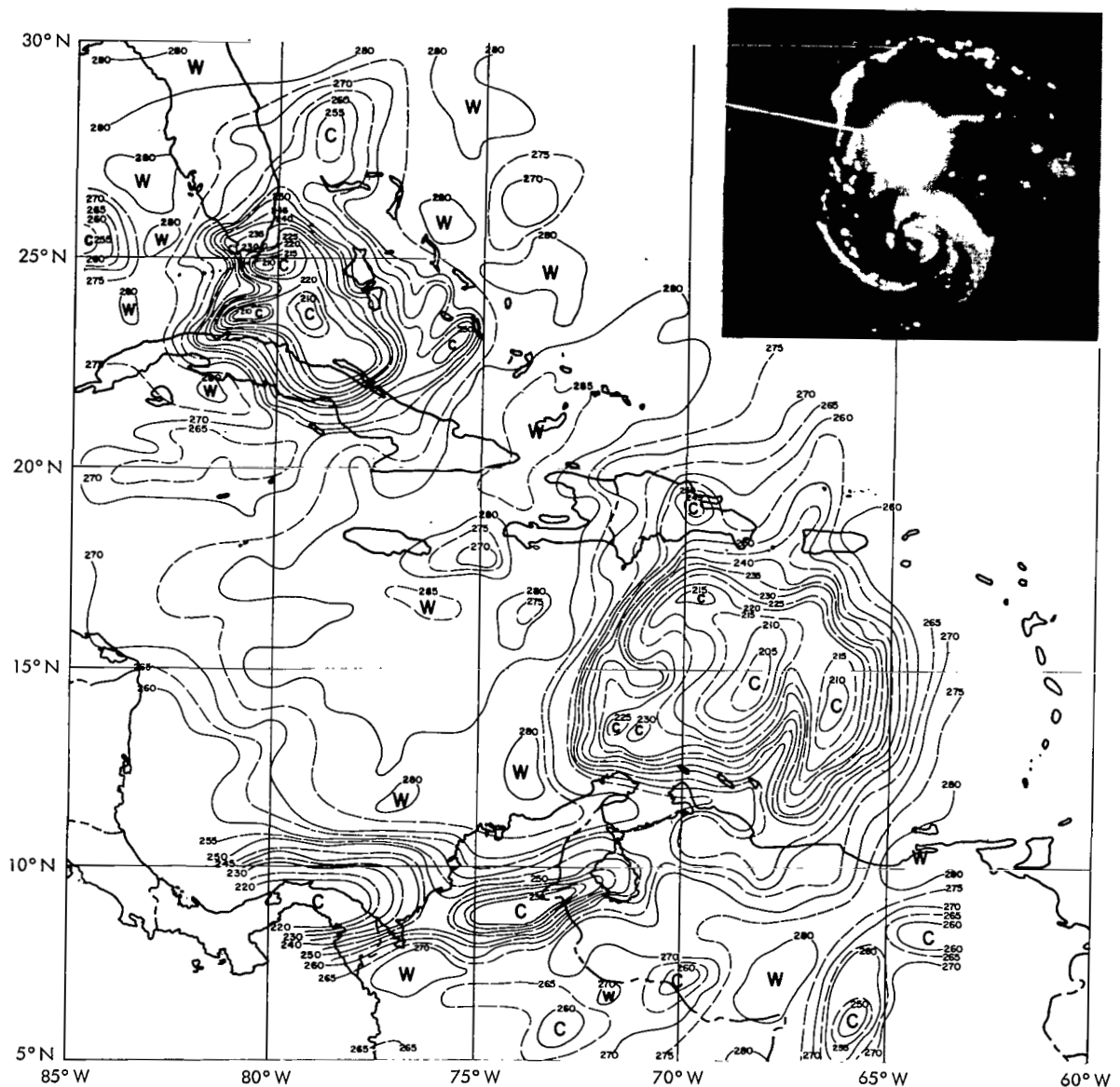
Figure 27—Channel 2 radiation analysis indicating Hurricane Flora, 1004-1012 Z, 2 October 1963, orbit 1553. The isolines show T_{BB} values in ^{\circ}\text{K} (uncorrected for instrumental degradation), U.S. Navy reconnaissance aircraft radar photograph indicating Hurricane Flora, 1100 Z approximately, 2 October 1963, 250 mile range.
