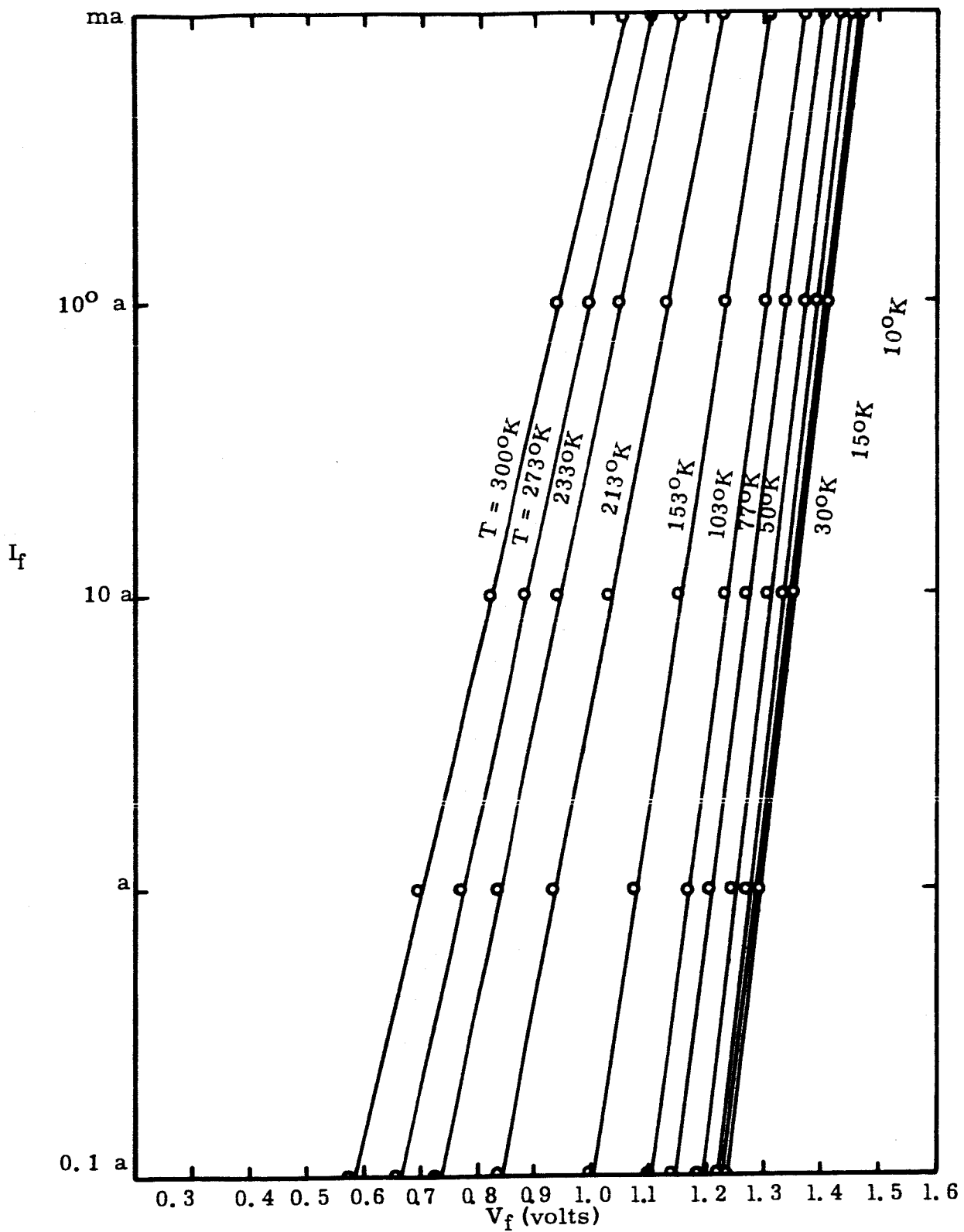
Forward Current Versus Forward Voltage as a Function of Temperature for Typical GaAs Temperature Sensor Diode #48
