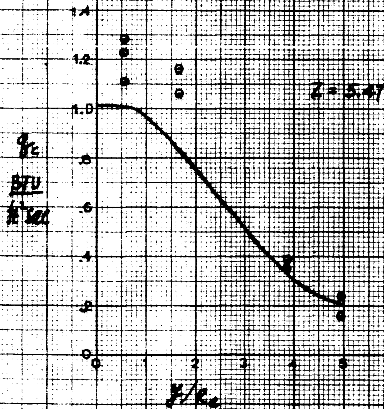
FIG. 12 Theoretical and Experimental Heating Rates (Oblique Shock Region) in Two Transverse Planes
