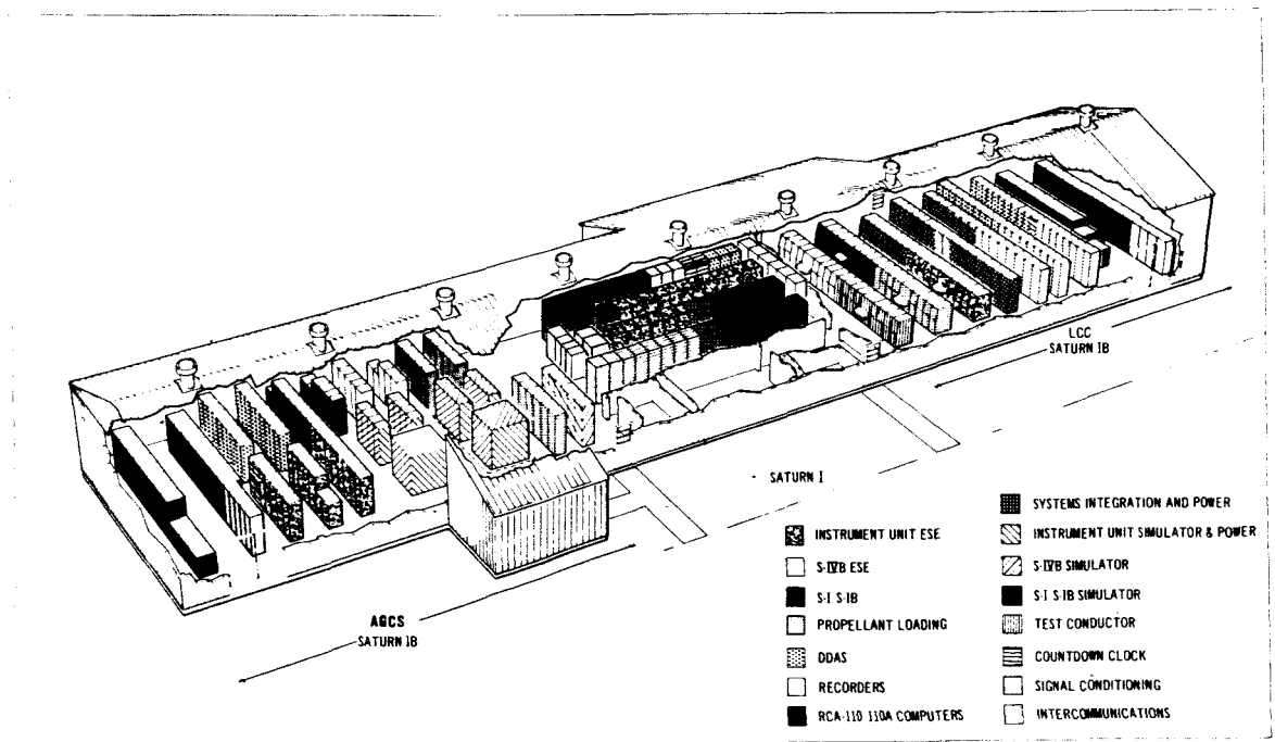
FIGURE 1. SATURN I/IB SYSTEMS DEVELOPMENT BREADBOARD FACILITY
