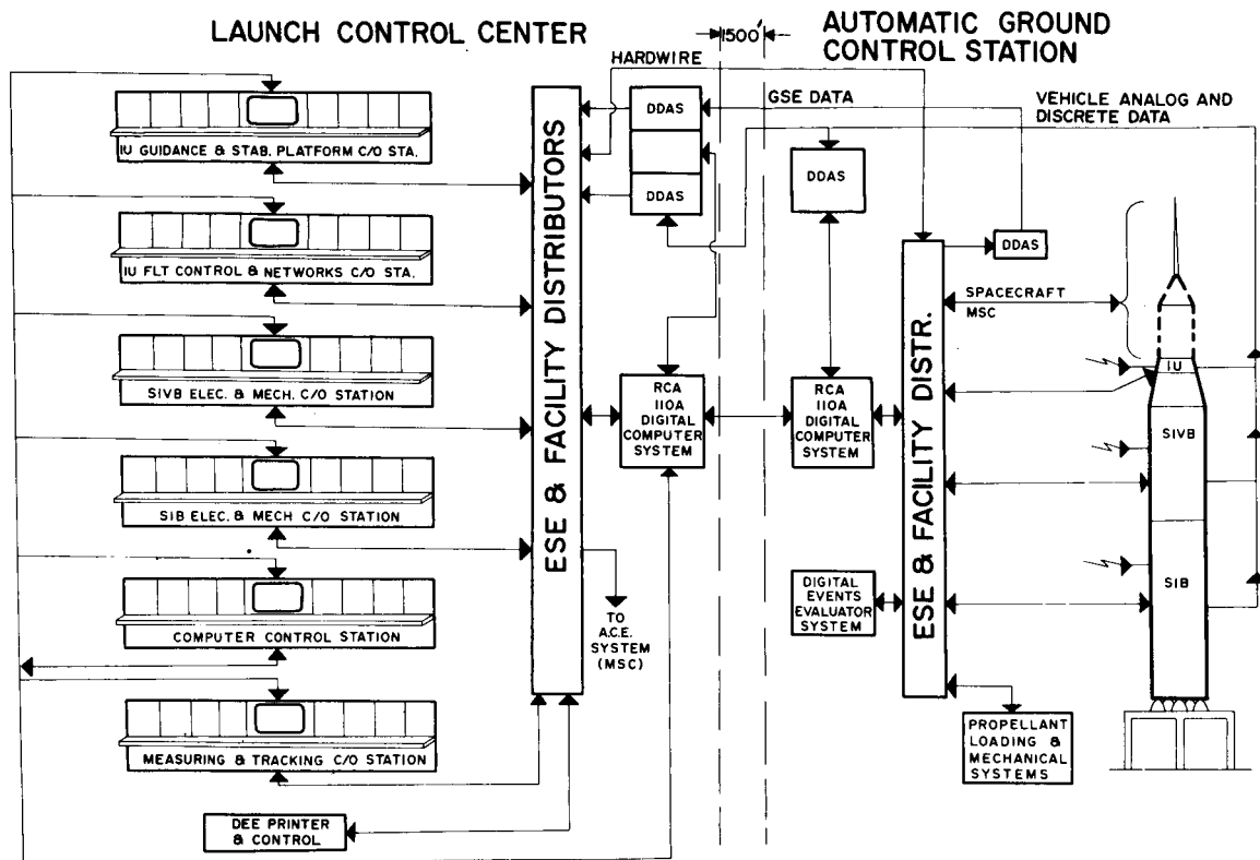
FIGURE 2. SATURN IB LAUNCH SYSTEM SIGNAL FLOW DIAGRAM
