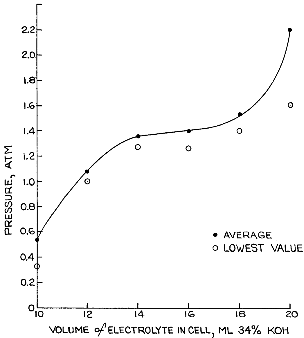
MI900 FIG. 2 PRESSURE CHANGES WITH ELECTROLYTE VOLUME DURING OVERCHARGE of SEALED NICKEL-CADMIUM CELLS
