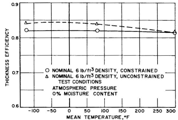
Fig. 14. Thickness efficiency vs mean temperature; moisture content, 0%
