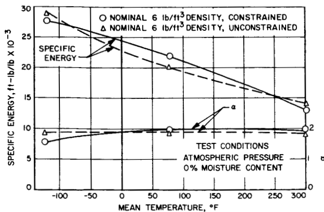
Fig. 12. Specific energy vs mean temperature; \alpha vs mean temperature; moisture content, 0%
