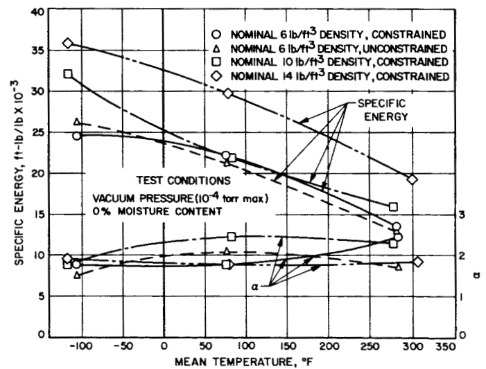
Fig. 15. Specific energy and \alpha vs mean temperature; vacuum pressure ( 10^{-4} torr max)
