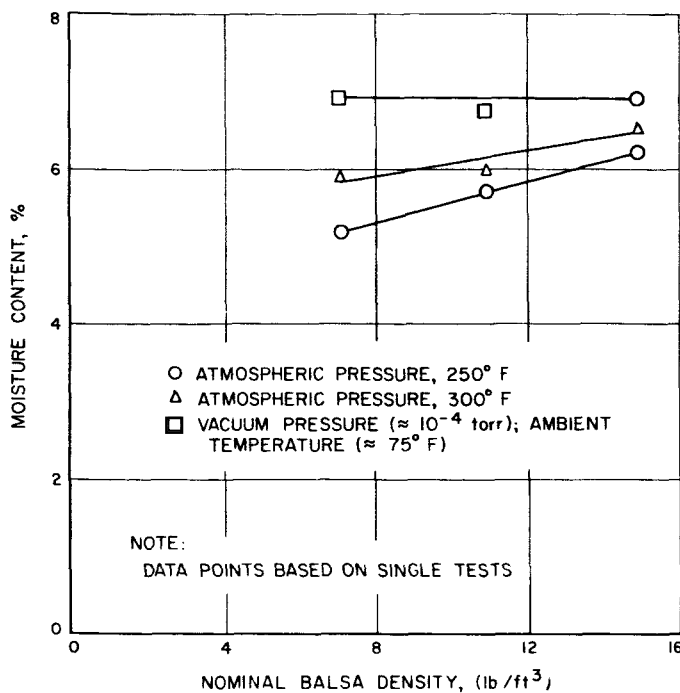
Fig. 3. Moisture content vs density
