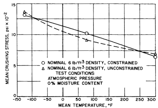
Fig. 13. Mean crushing stress vs mean temperature; moisture content, 0%
