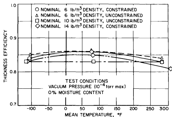
Fig. 17. Thickness efficiency vs mean temperature; vacuum pressure ( 10^{-4} torr max)
