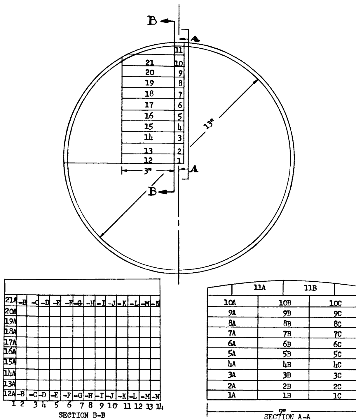
Figure 1 Specimen Locations of Standard 7075-T6 and Special Product 7079-T6 Hand Forgings
