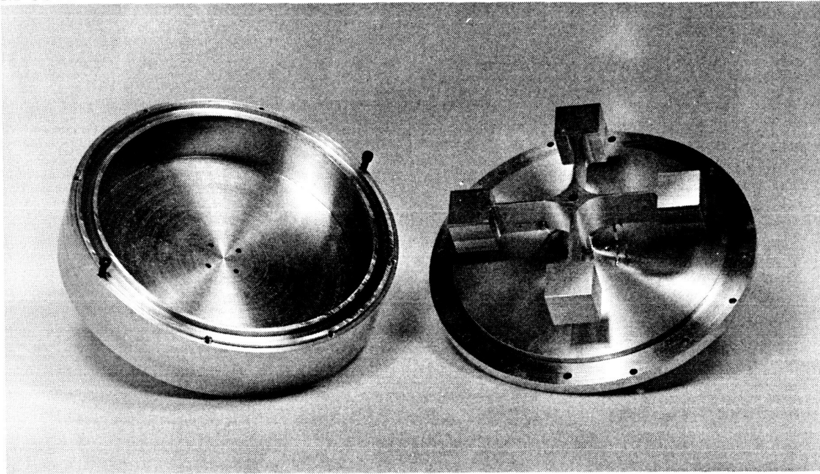
Fig. 9. Cruciform gravitational mass sensor.
