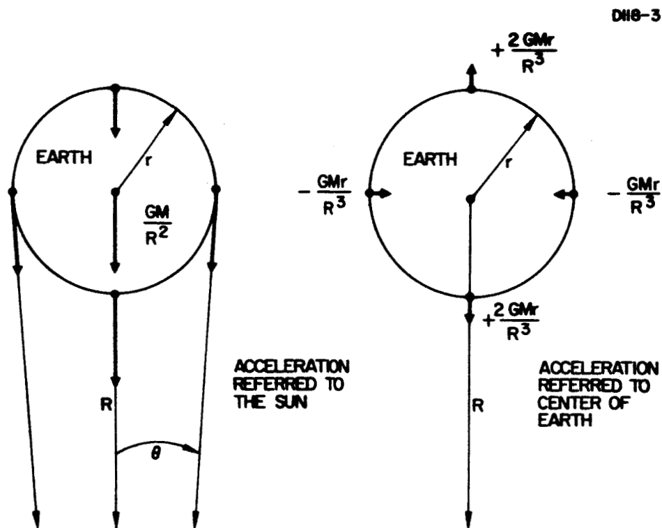
Fig. 4. Radial and azimuthal contributions to the earth's tides.
