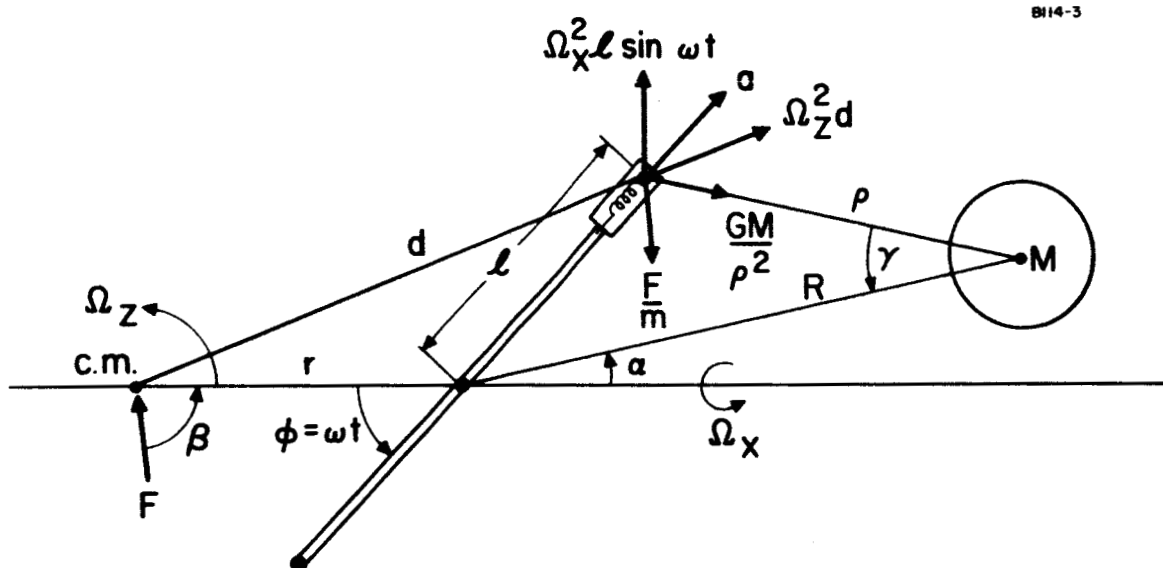
Fig. 8. Effect of gravitational and inertial fields on rotating sensor.
