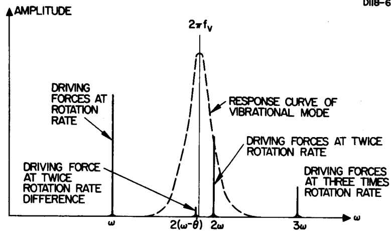
Fig. 6. Response of vibrational mode to driving forces from various sources.
