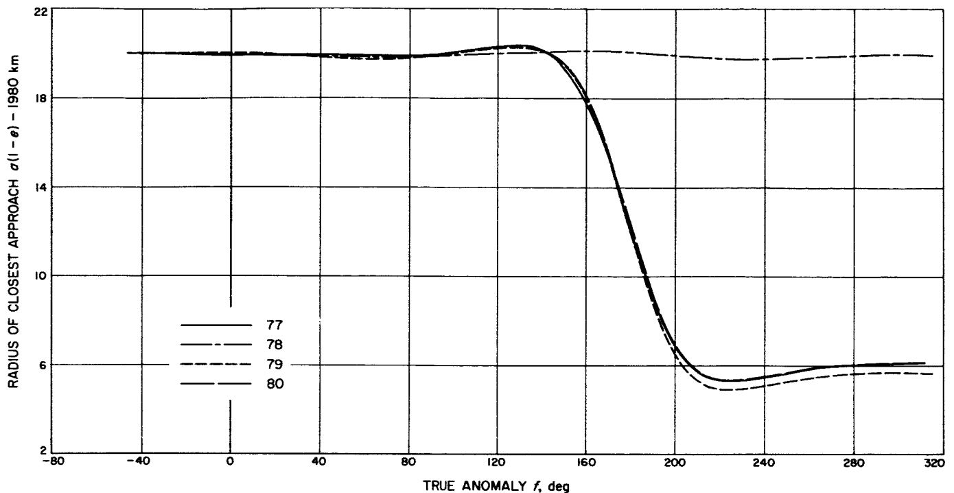
Fig. 6. Radius of closest approach
