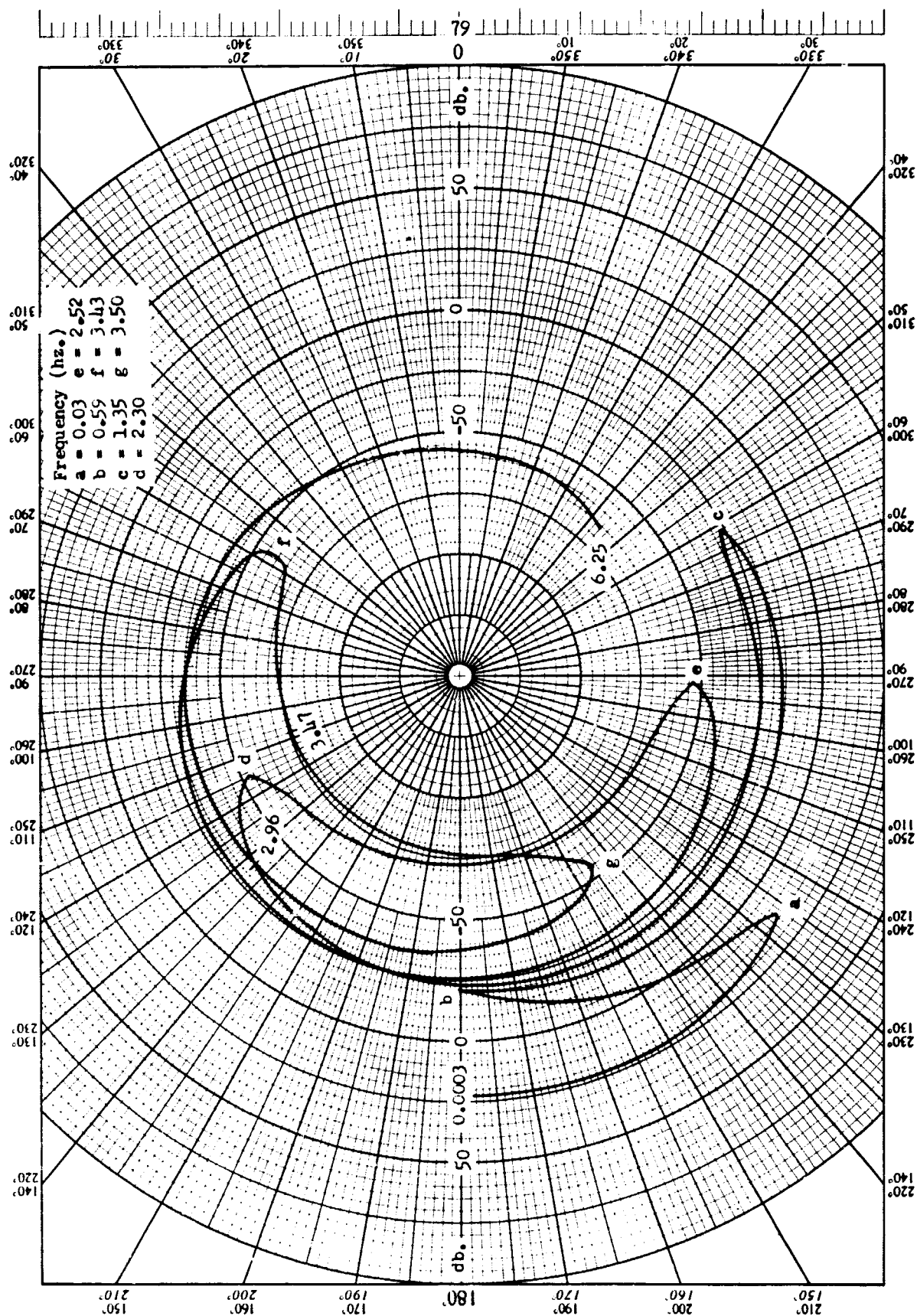
Fig. 36-Nyquist diagram broken in \phi channel of system shown in Fig. 23, T = 0.08
