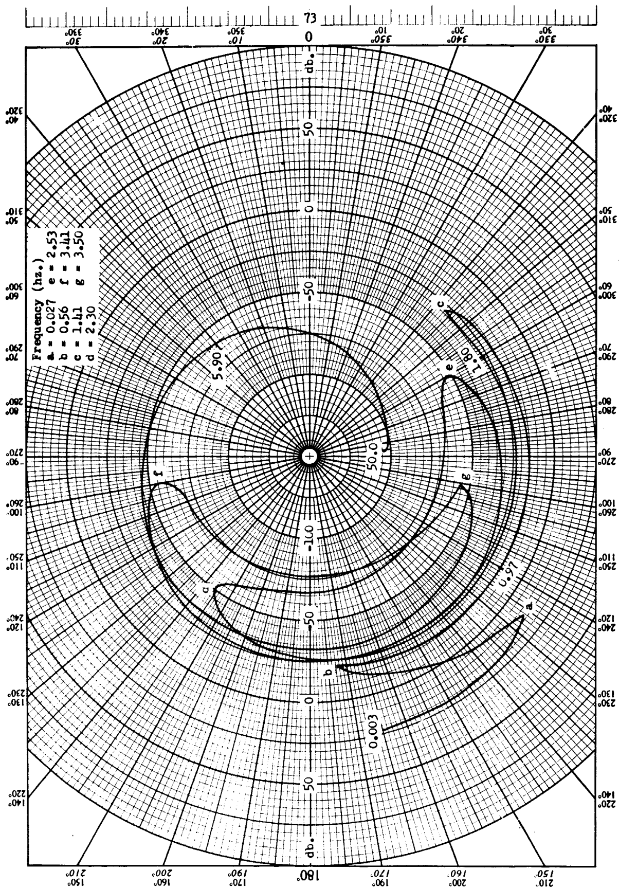
Fig. 30--Nyquist diagram broken in \phi channel of system shown in Fig. 23, T = 0.01
