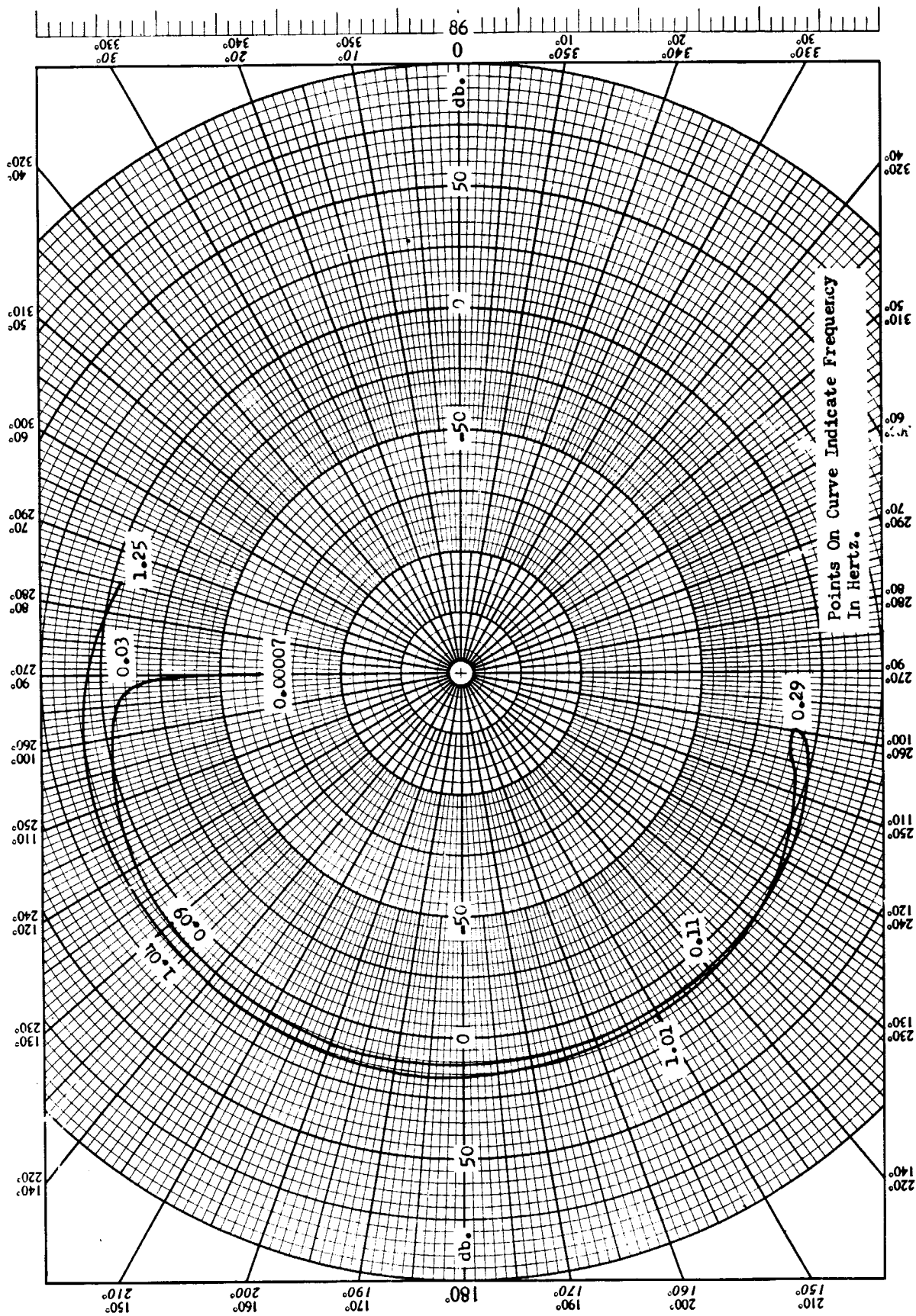
Fig. 43 --Nyquist diagram broken in \phi channel of system shown in Fig. 23, T = 0.4
