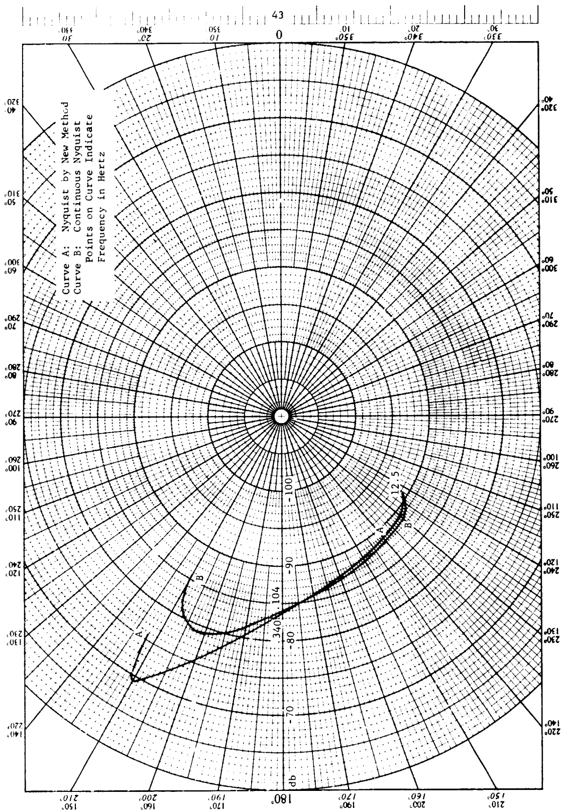
Fig. 18--Nyquist diagrams of system shown in Figure 1 broken in \beta_c channel and described by (41) and (42)
