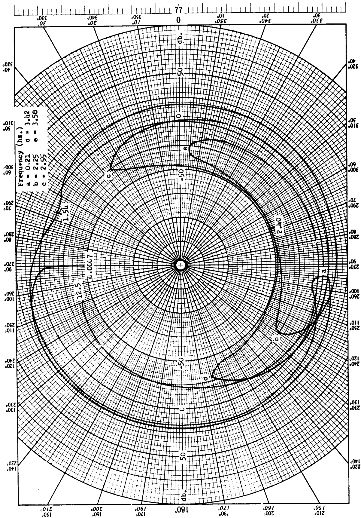
Fig. 34--Nyquist diagram broken in \phi channel of system shown in Fig. 23, T = 0.04
