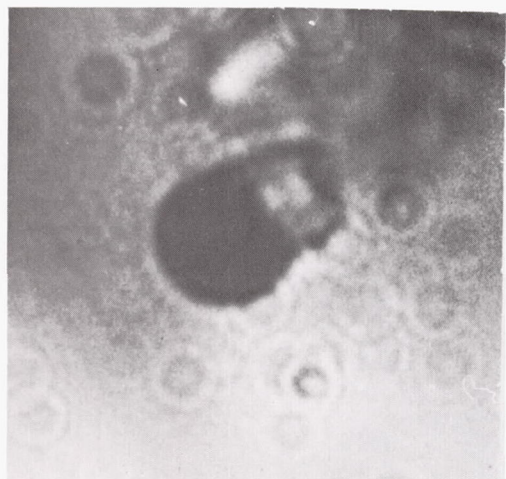
Germination of Spores in a 1 Year Old Culture of 36N \text{H}_2\text{SO}_4 Kept at a Constant 60^\circ .
