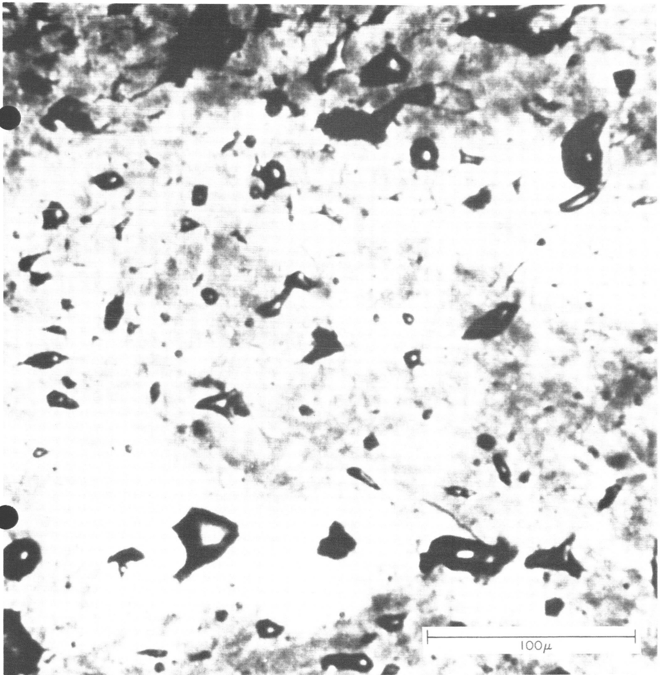
Fig. 32. Angular bubbles observed in a Muong Nong tektite from Kan Luang Dong. Courtesy of V. Barnes. The black marks are voids.
