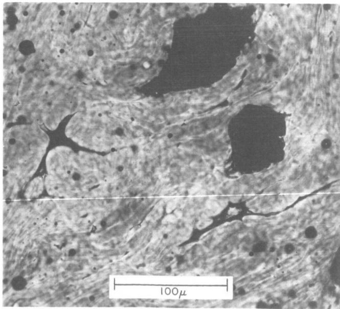
Fig. 33. Microphotograph of a portion of a Muong Nong tektite from Phaeng Dang, showing internal structure. The two large black spots are inclusions. The small, streaky black lines are voids between shard-like glass bodies. The voids do not extend through the section.
