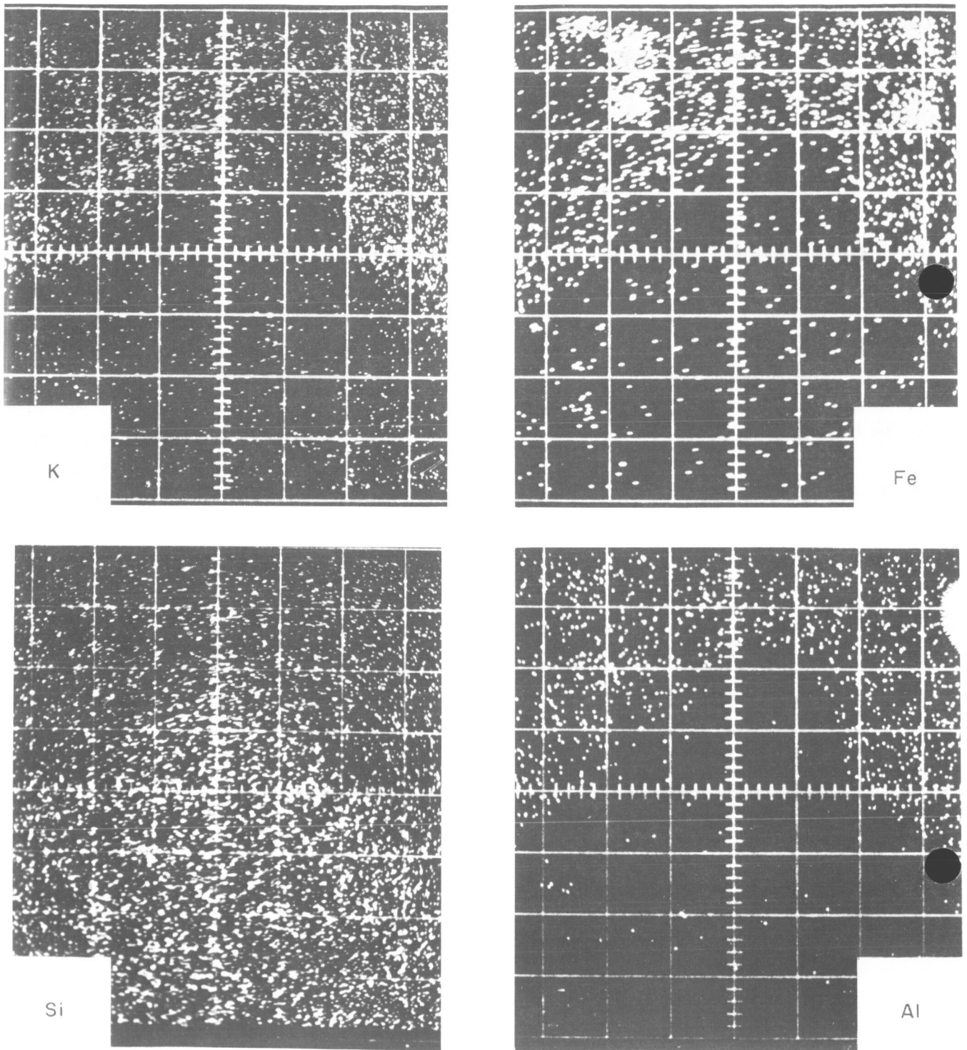
Fig. 38. Microprobe scans for the elements potassium, iron, silicon and aluminum on a sample of Texas siltstone. Note the inhomogeneity as compared with the tektite. Each figure is 90 μ across.
