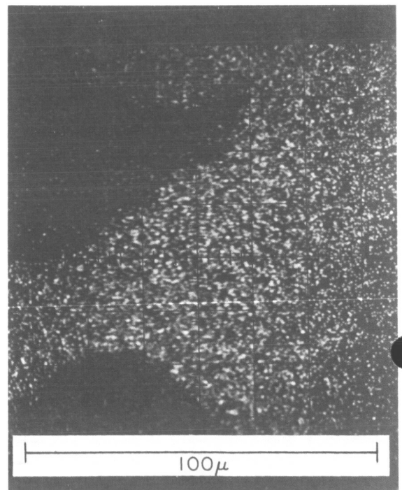
Fig. 34. A portion of the same region as Fig. 33 in the line of the potassium K_{\alpha} line prepared by microprobe scanning using X-ray fluorescence. The image is reversed compared with Fig. 33. Note the homogeneity of the material outside the black inclusions.
