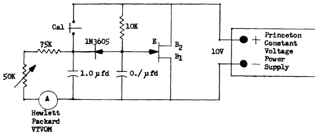
Figure 3. Test Circuit for Measurement of Intrinsic Standoff Ratio.
