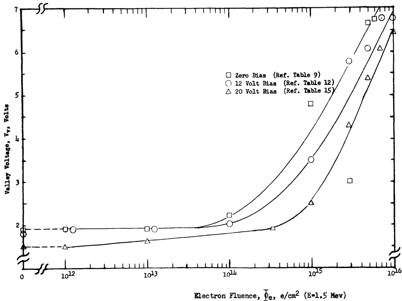
Figure 20. Valley Voltage ( V_v ) versus Electron Fluence for 2N3484.
