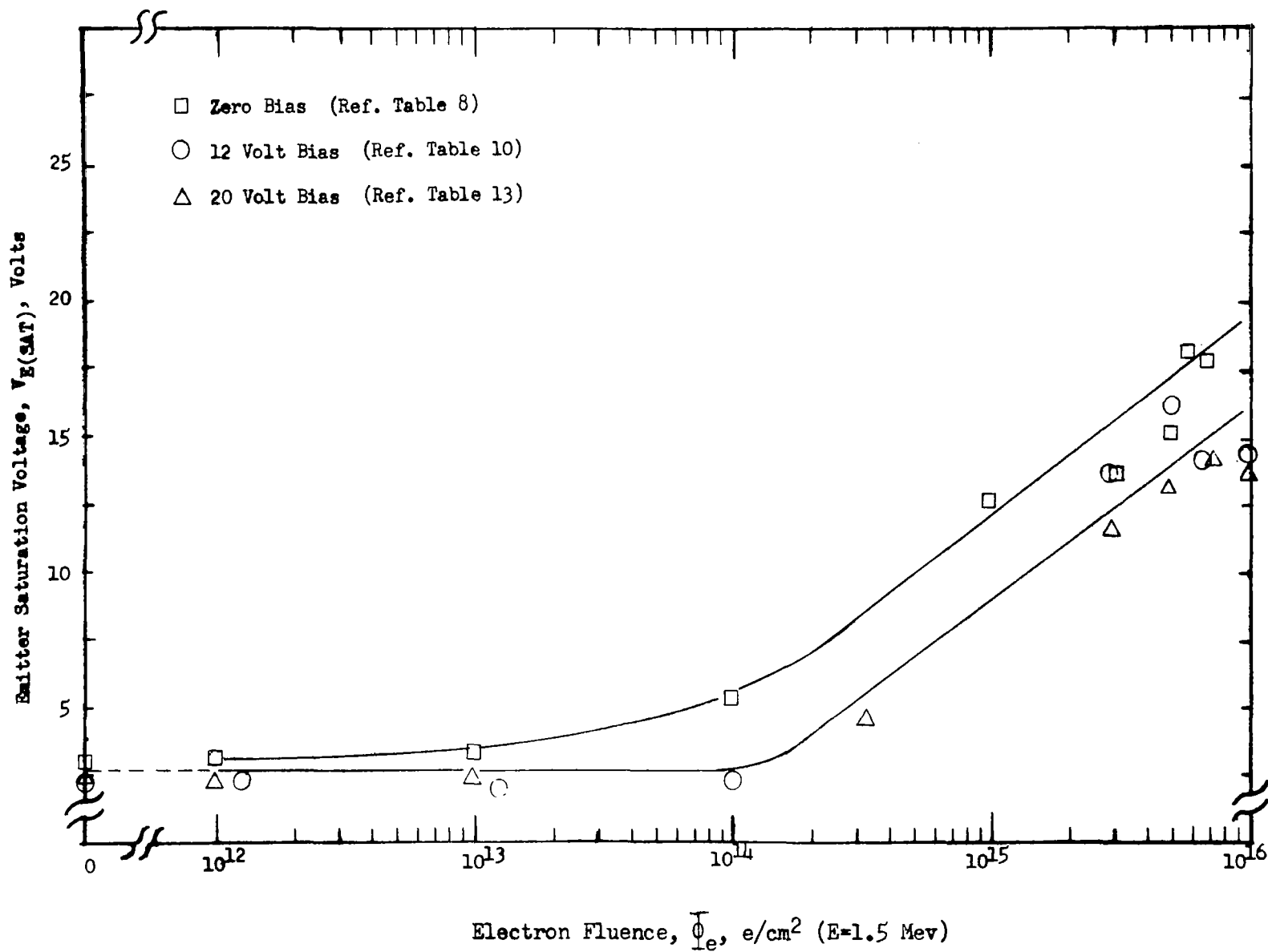
Figure 12. Emitter Saturation Voltage ( V_E(\text{SAT}) ) versus Electron Fluence for 2N1671B.
