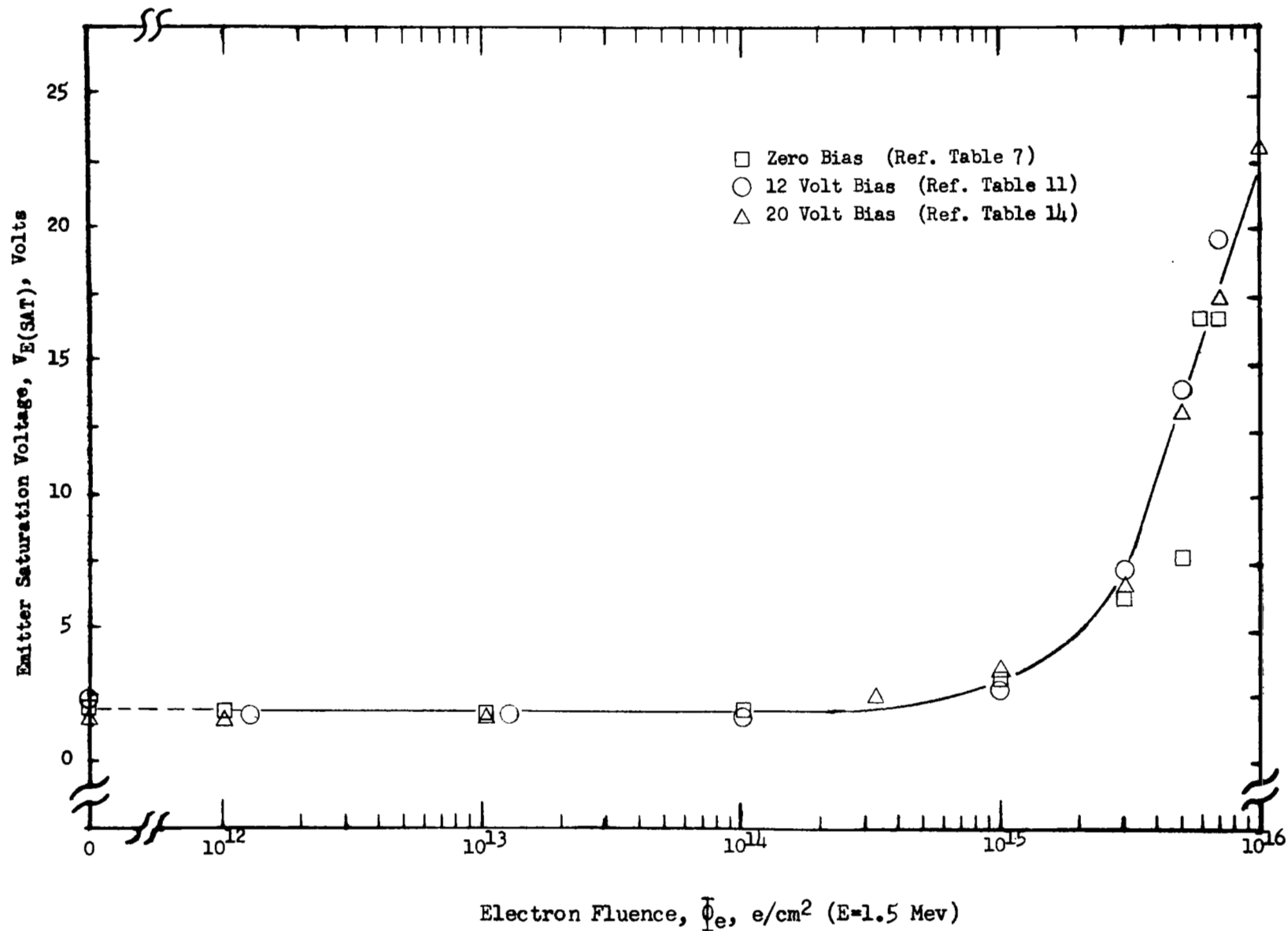
Figure 17. Emitter Saturation Voltage ( V_{E(SAT)} ) versus Electron Fluence for 2N3980.
