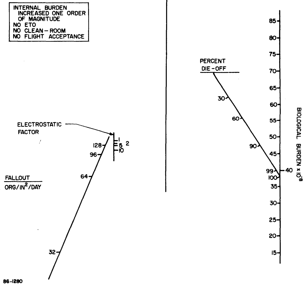
Figure 18 CONTAMINATION SENSITIVITY NOMOGRAM - NO PROCESS CONTROLS AND INTERNAL BURDEN INCREASED
