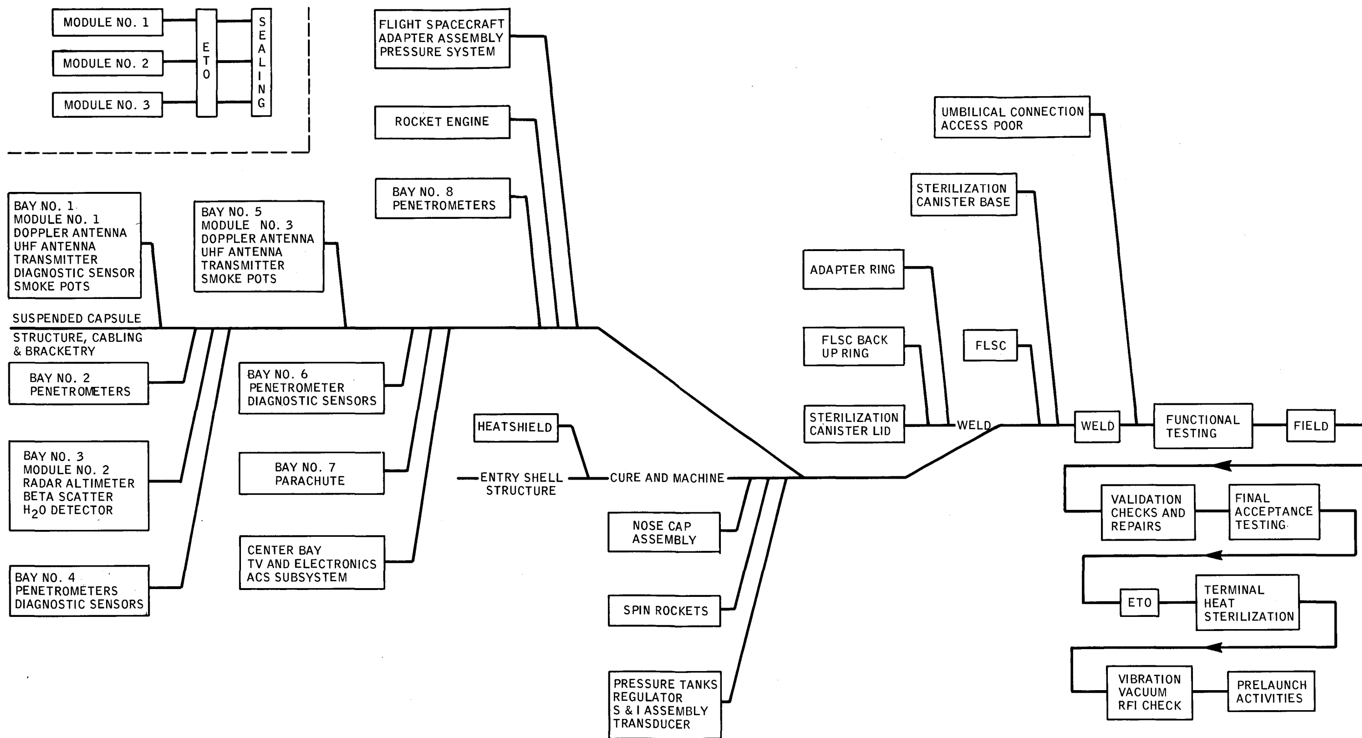
Figure 37 PROBE-ENTRY FROM ORBIT - FACTORY-TO-LAUNCH FLOW SEQUENCE
