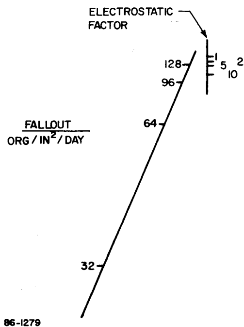
Figure 17 CONTAMINATION SENSITIVITY NOMOGRAM - NO PROCESS CONTROLS AND INTERNAL BURDEN REDUCED
