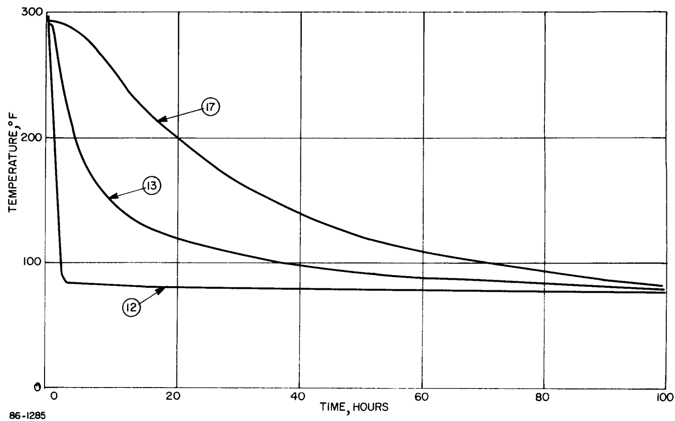
Figure 34 TYPICAL COOLDOWN HISTORY
