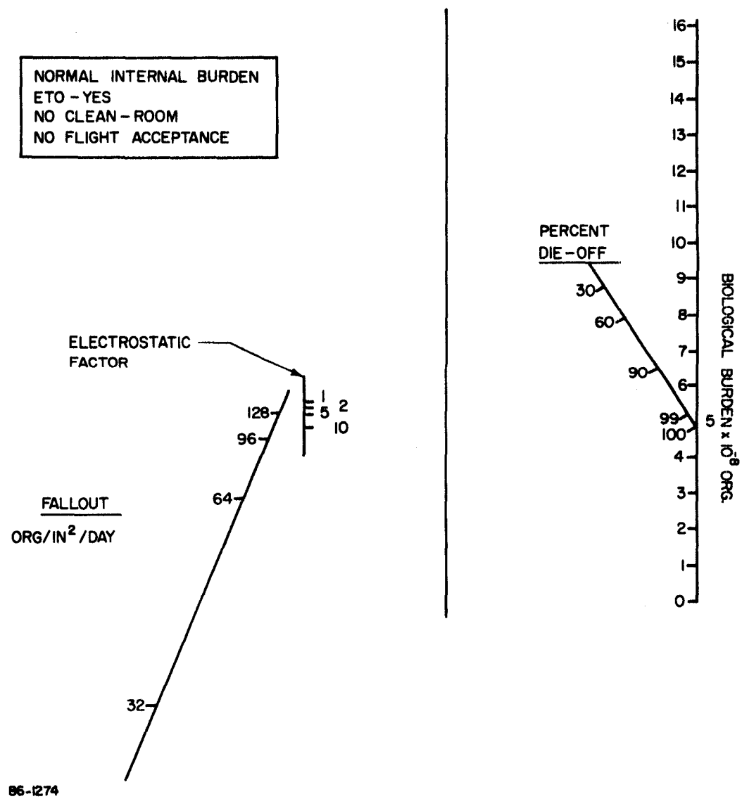
Figure 12 CONTAMINATION SENSITIVITY NOMOGRAM - ETO CONTROL ONLY
