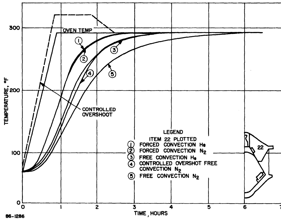
Figure 35 COMPARISON OF COMPONENT RESPONSE FOR VARIOUS HEATING TECHNIQUES
