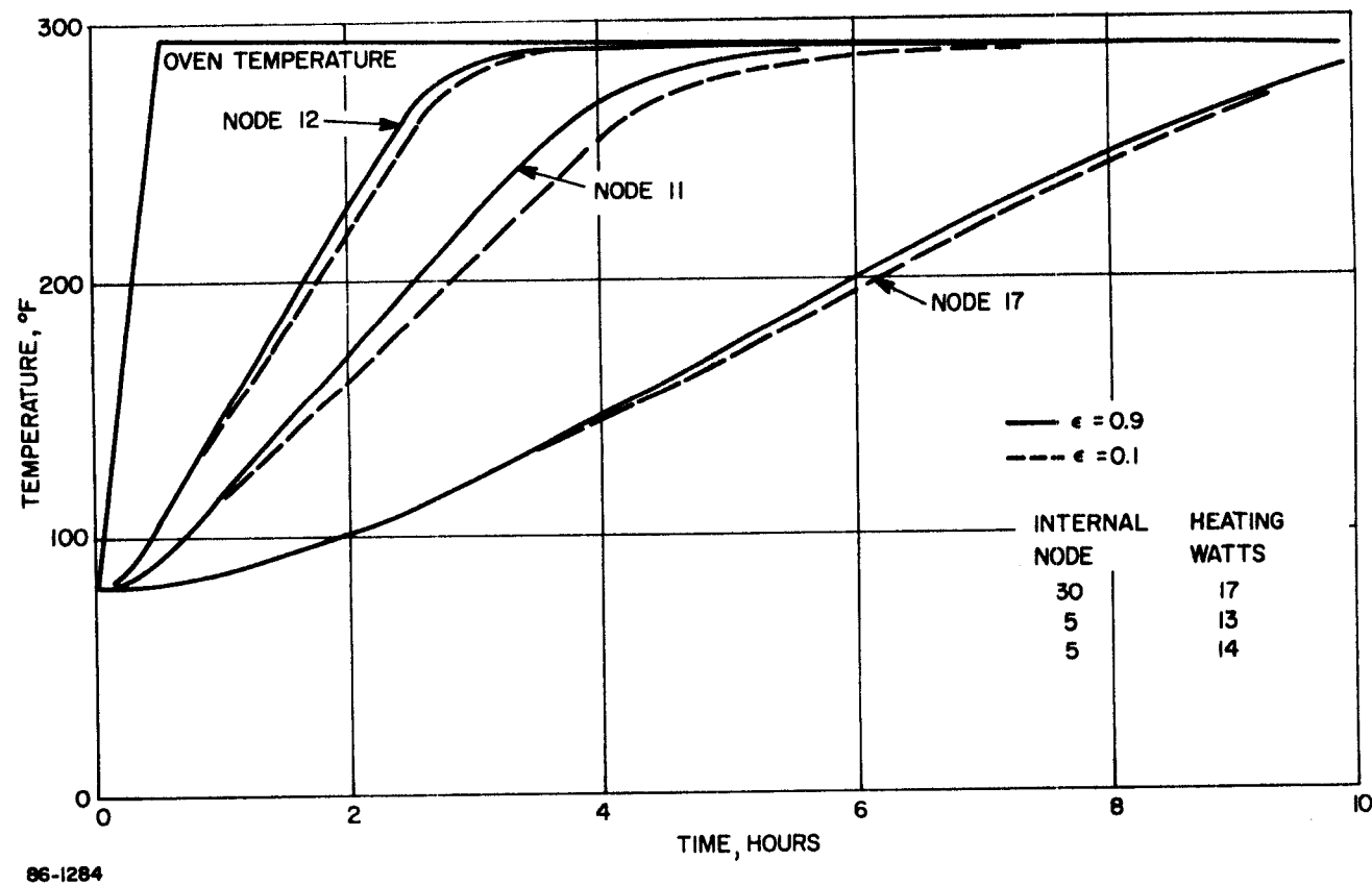
Figure 33 EFFECT OF VARIATION OF EMISSIVITY OF INTERNAL SURFACE ON INTERNAL HEAT TRANSFER
