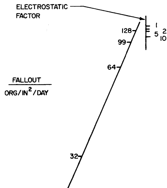
Figure 14 CONTAMINATION SENSITIVITY NOMOGRAM - FA CONTROL ONLY
