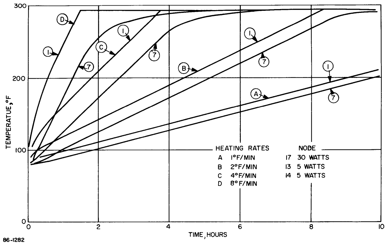
Figure 32 EFFECT OF EXTERNAL HEATING RATES
