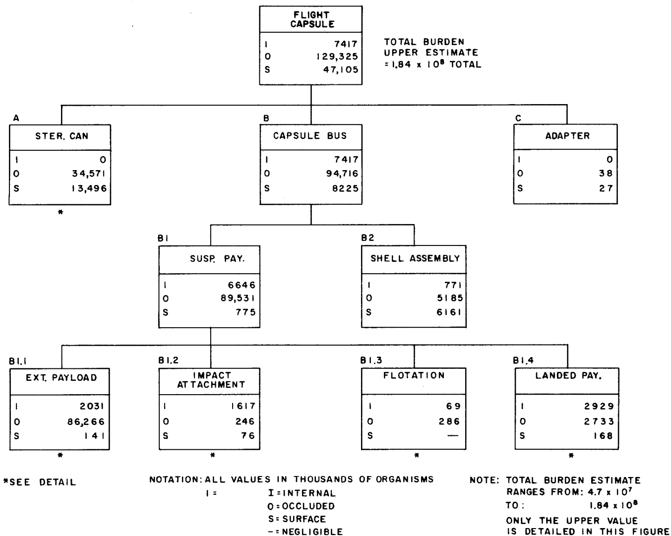
Figure 19 INITIAL FLIGHT CAPSULE BURDEN ESTIMATES
