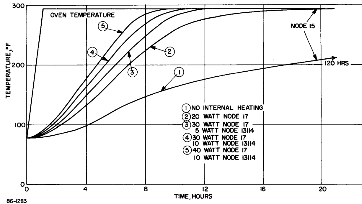
Figure 31 EFFECT OF INTERNAL HEATING ON TIME TO REACH STERILIZATION TEMPERATURE
