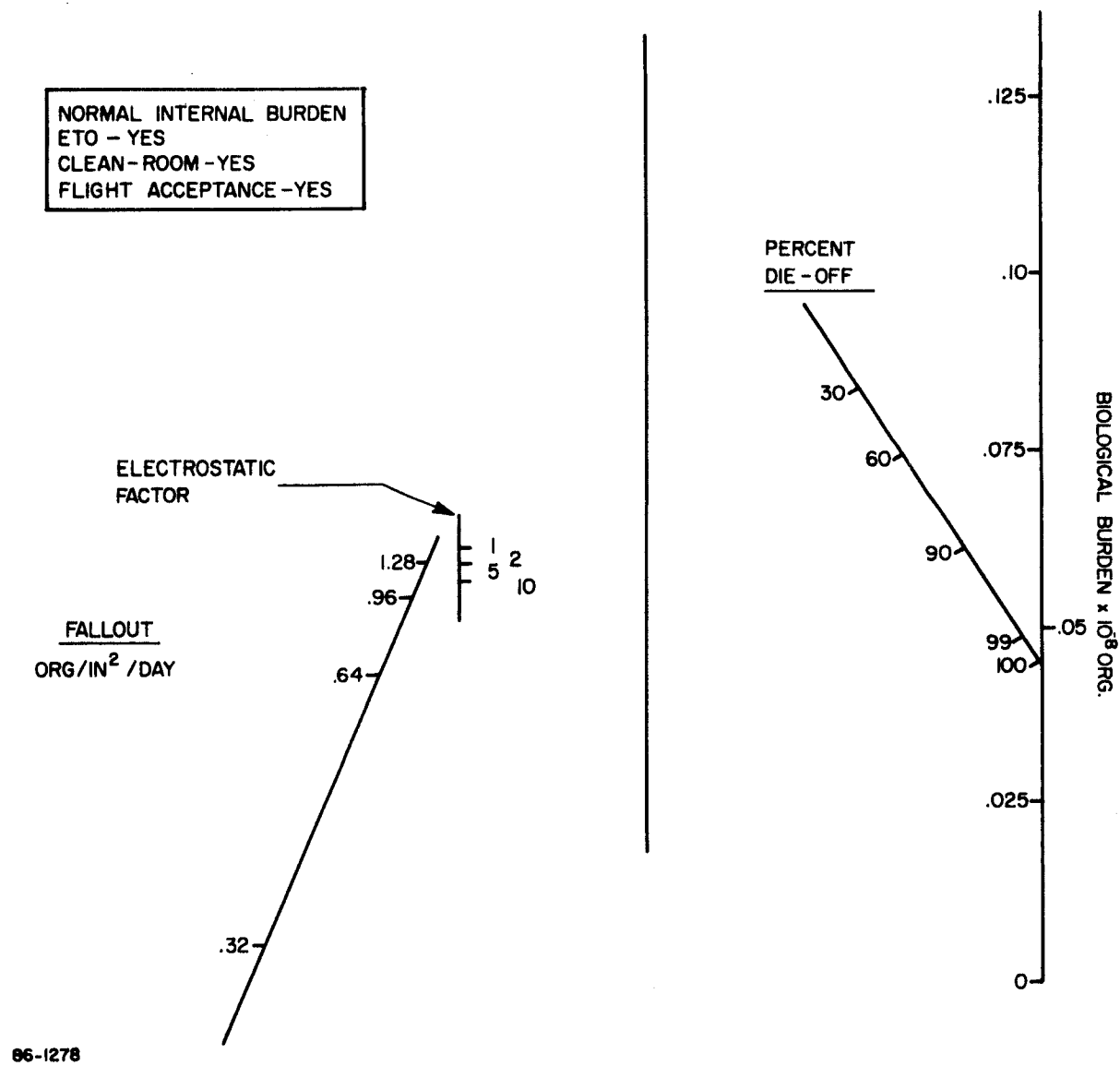
Figure 16 CONTAMINATION SENSITIVITY NOMOGRAM - ALL CONTROLS APPLIED
