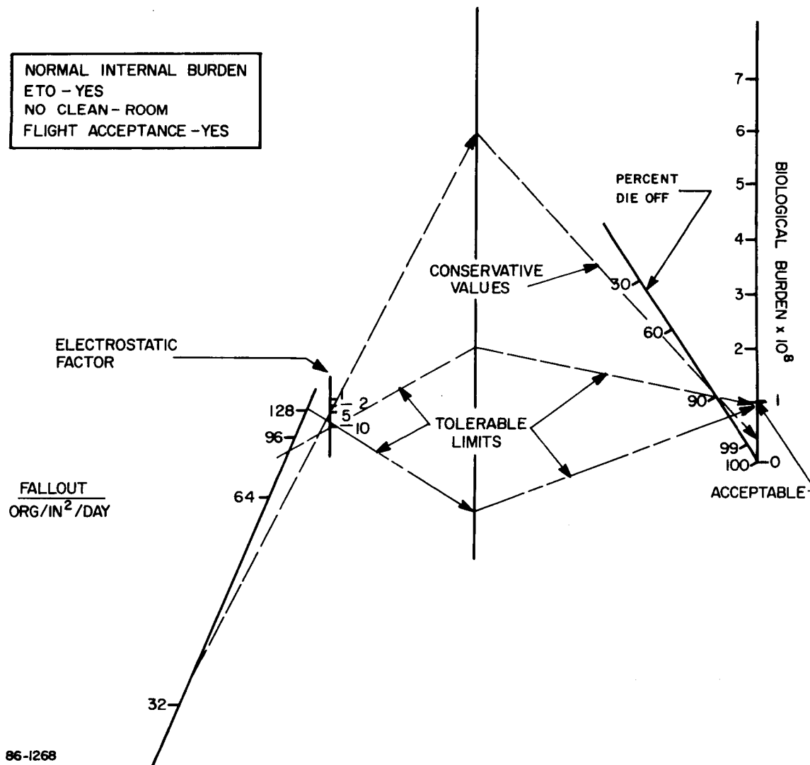
Figure 4 CONTAMINATION SENSITIVITY NOMOGRAM
