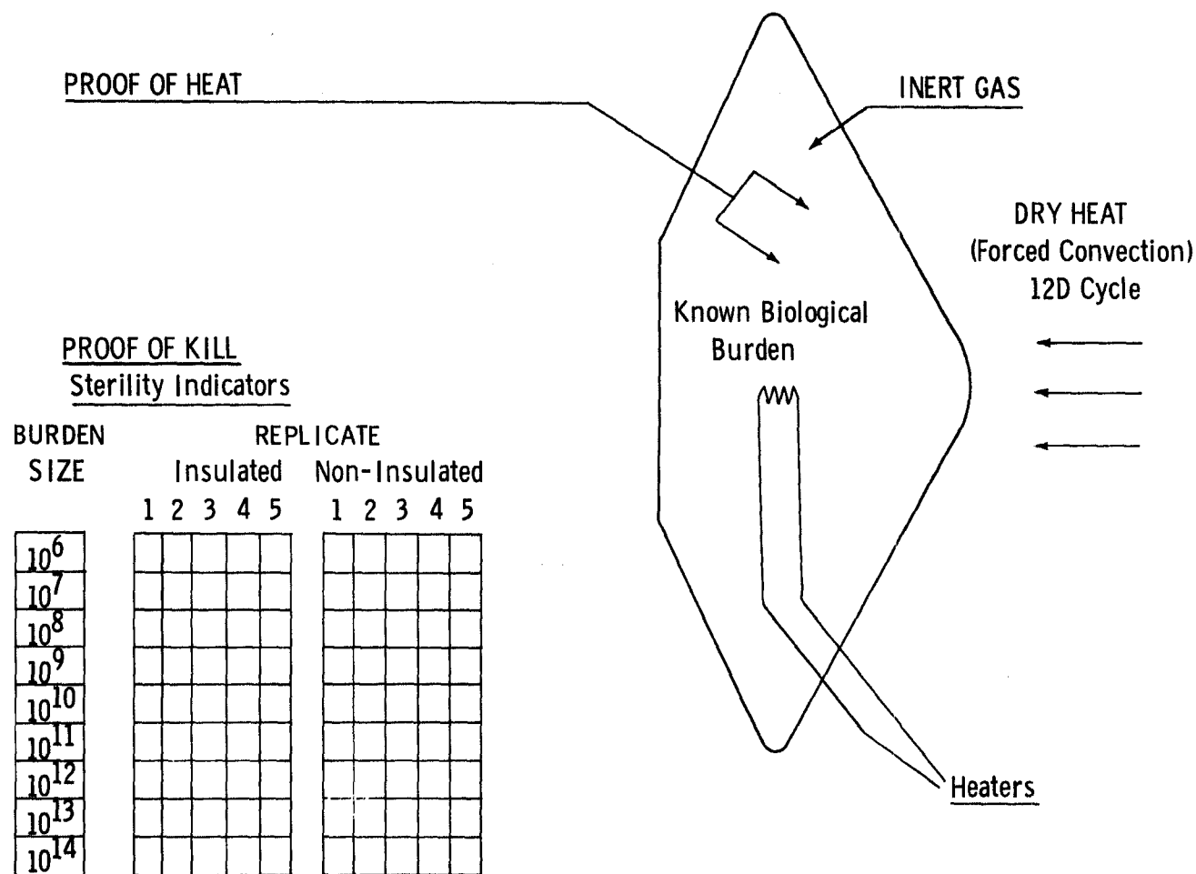
Figure 6 TERMINAL STERILIZATION CONFIGURATION
