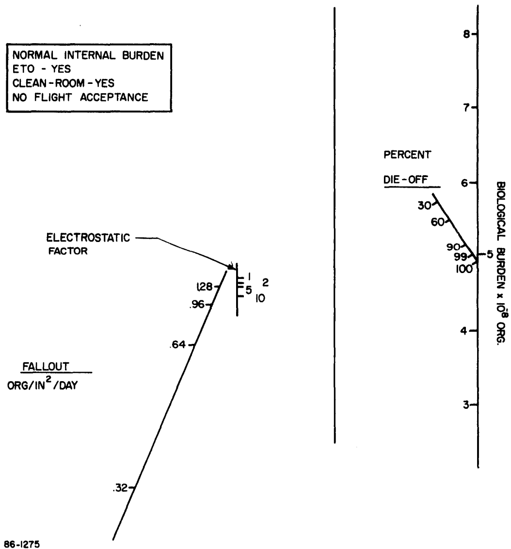
Figure 13 CONTAMINATION SENSITIVITY NOMOGRAM - ETO AND CLEAN-ROOM CONTROLS
