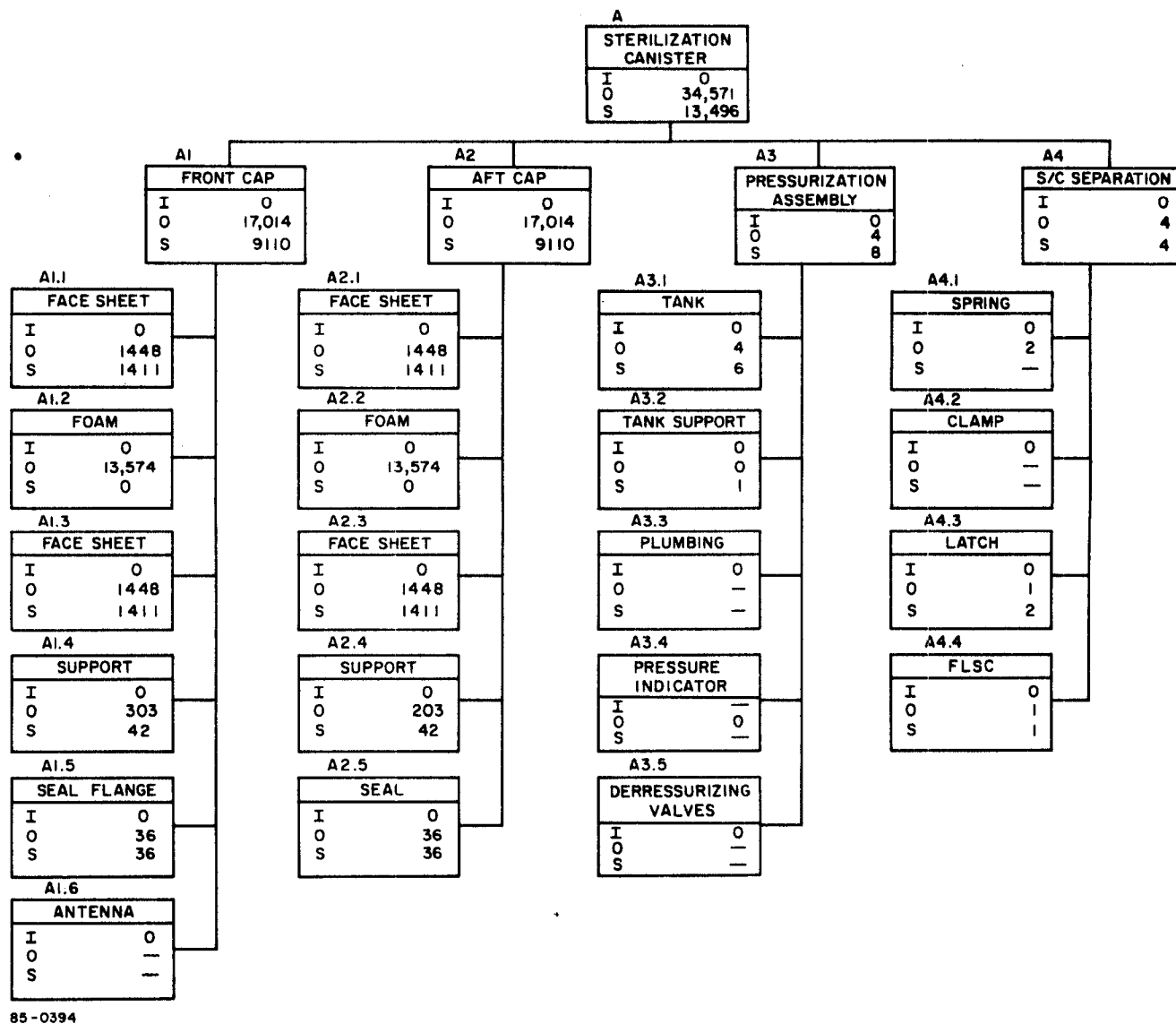
Figure 20 INITIAL FLIGHT CAPSULE BURDEN ESTIMATES- STERILIZATION CANISTER
