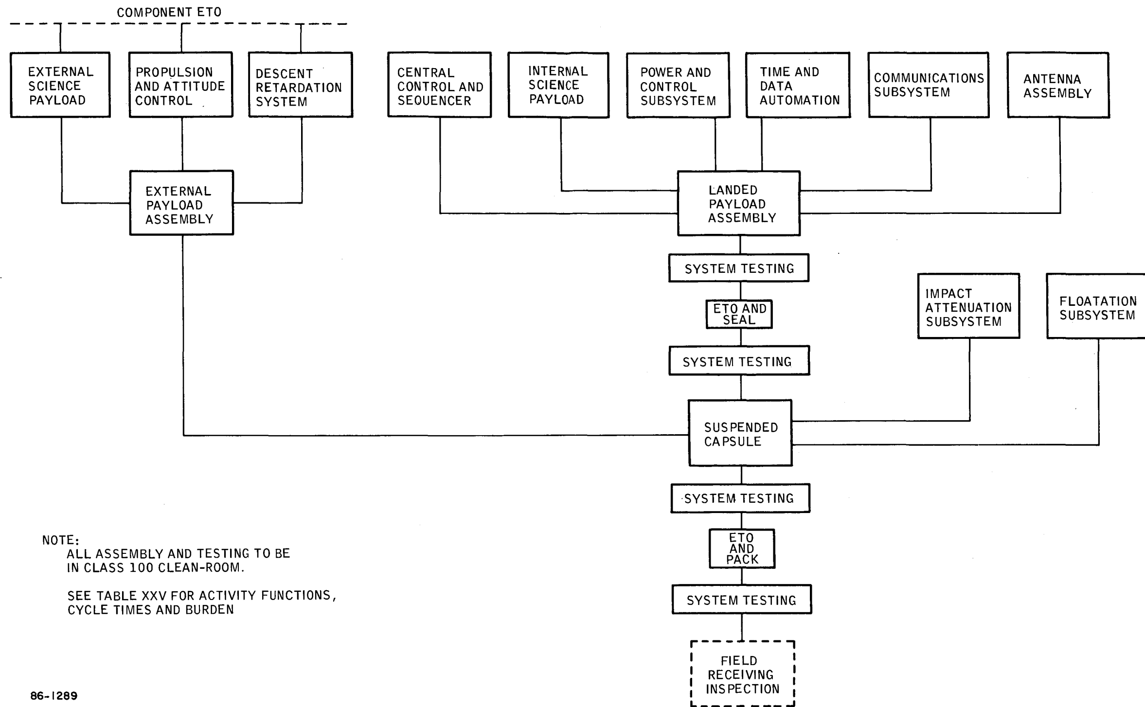
Figure 40 PROBE/LANDER-ENTRY FROM THE APPROACH TRAJECTORY - SUSPENDED CAPSULE ASSEMBLY AND TEST - BLOCK DIAGRAM
