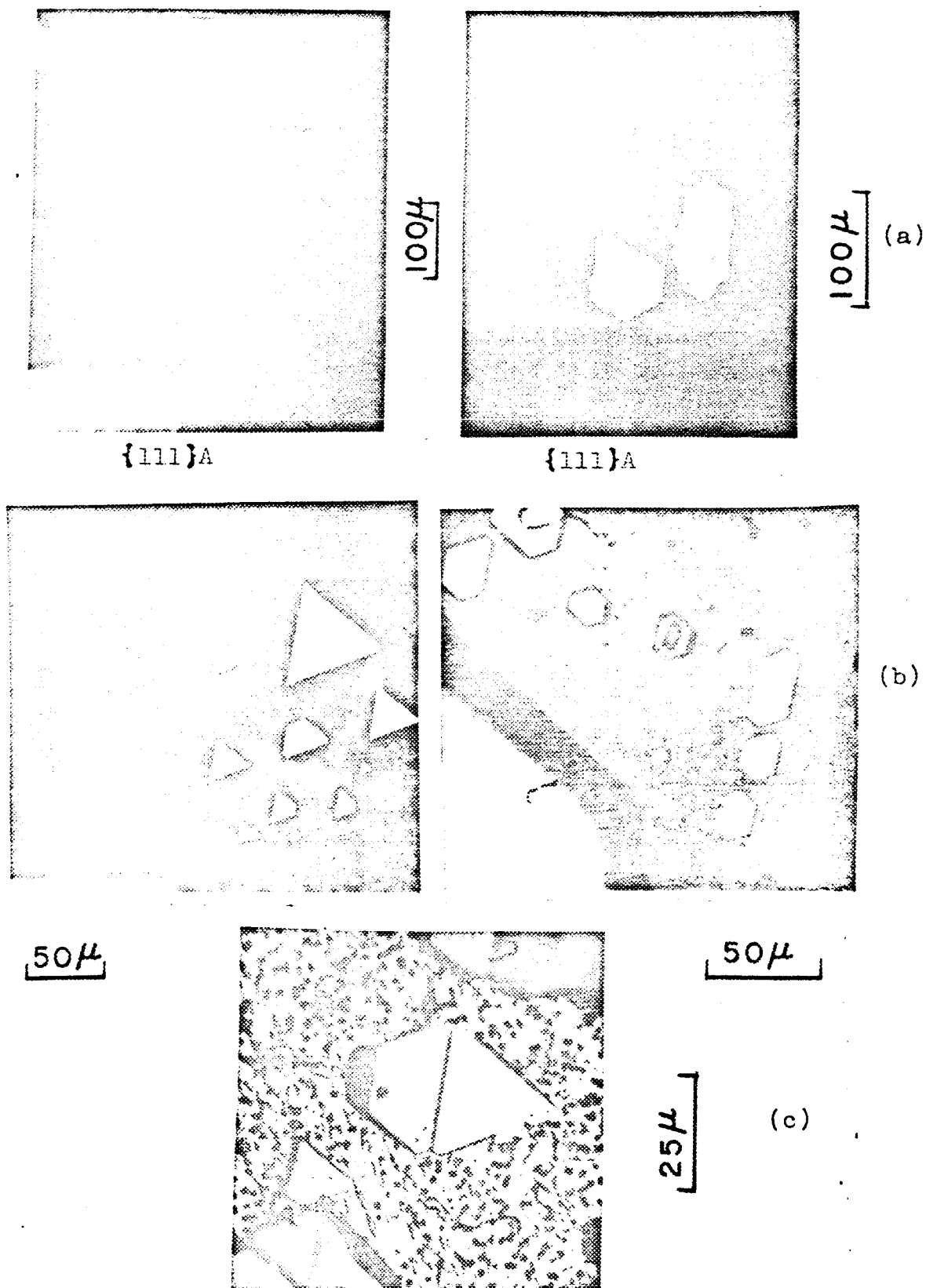
Figure 18. Photomicrographs of the "island" structure on (a) {111}A seed (b) {111}B seed (c) Twinned "islands" on {111}B seed
