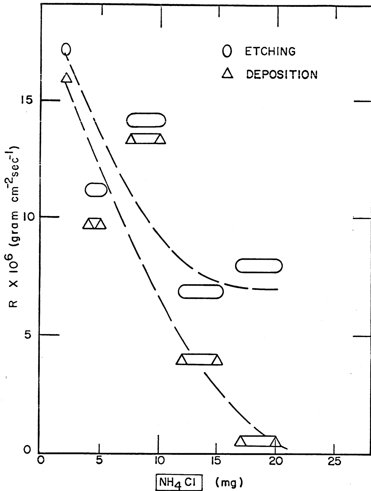
Figure 12. Rates of deposition on the {110} and etching of the {110} source vs. the initial values of \text{NH}_4\text{Cl} at T = 900^\circ\text{K} and \langle \text{is} \rangle = 0 .
