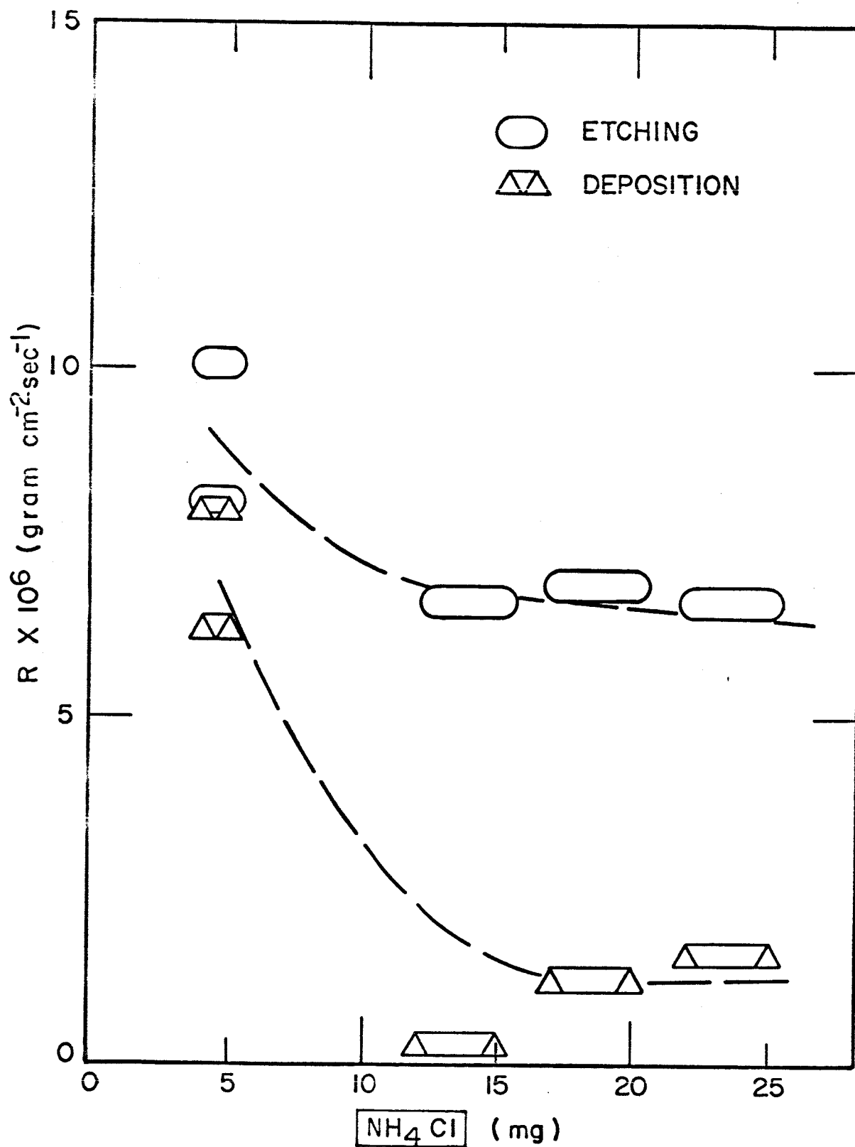
Figure 11. Rates of deposition on the \{111\} surface and etching of the poly-crystalline surface vs. the initial values of \text{NH}_4\text{Cl} at T = 975^\circ\text{K} and \langle \Delta s \rangle = 0 .
