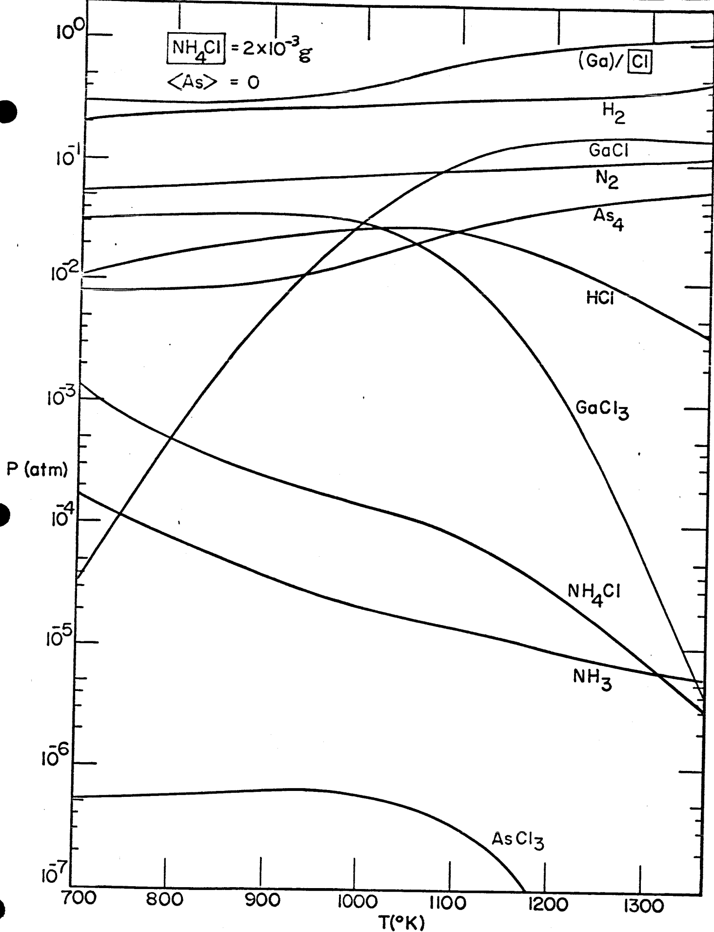
Figure 1. Composition of the gas phase of \text{NH}_4\text{Cl} -Ga-As system vs. temperature with the initial values of \text{NH}_4\text{Cl} = 2 \text{ mg.} and no excess arsenic.
