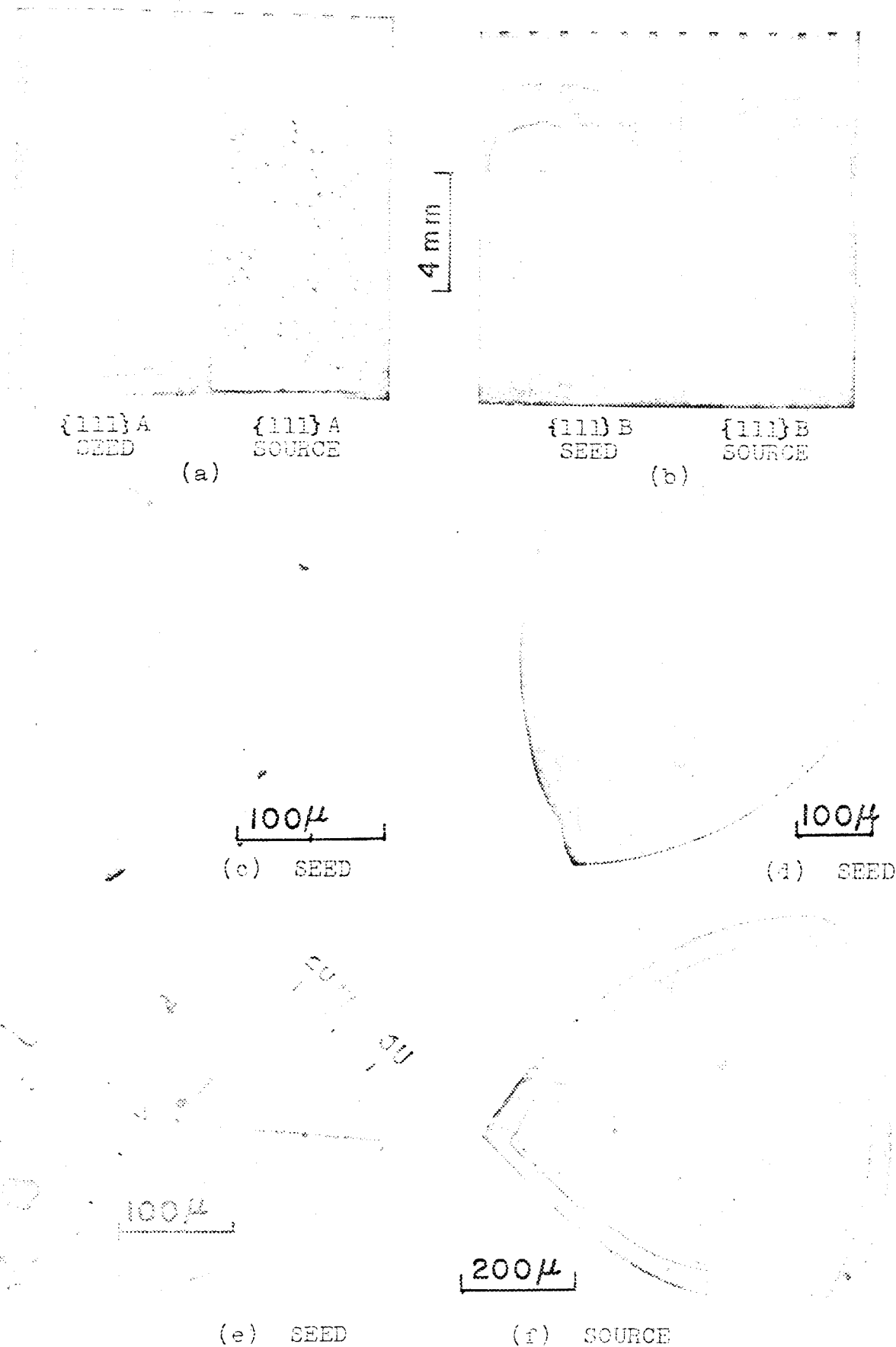
Figure 15. Photomicrographs of the epitaxial overgrowth pattern of the seed and the etched surface pattern of the source. (a) \{111\} A seed and \{111\} A source. (b) \{111\} B seed and \{111\} B source. (c) Tetrahedral dislocation-growth with one apex. (d) and (e) Tetrahedral dislocation-growth with multiple apexes. (f) Tetrahedral etch-pit with multiple apexes.
