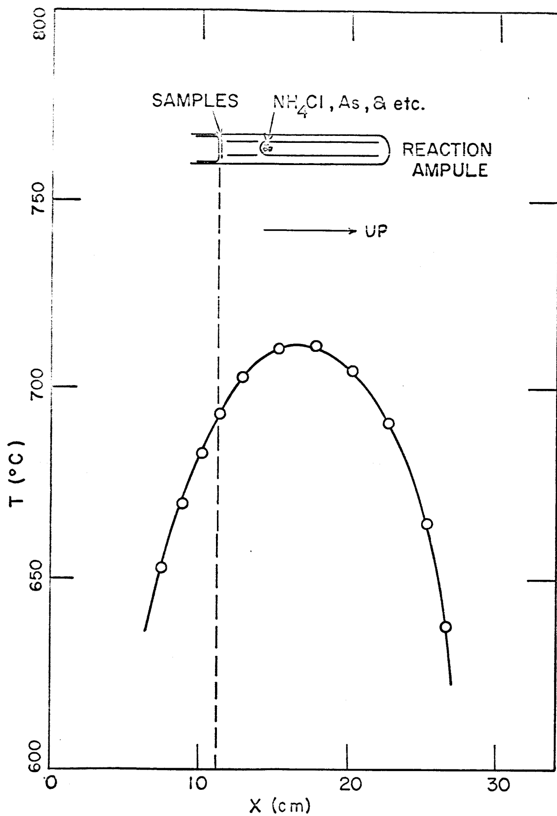
Figure 9. Temperature profile of the reaction ampule, measured without the ampule, at the position of the ampule.
