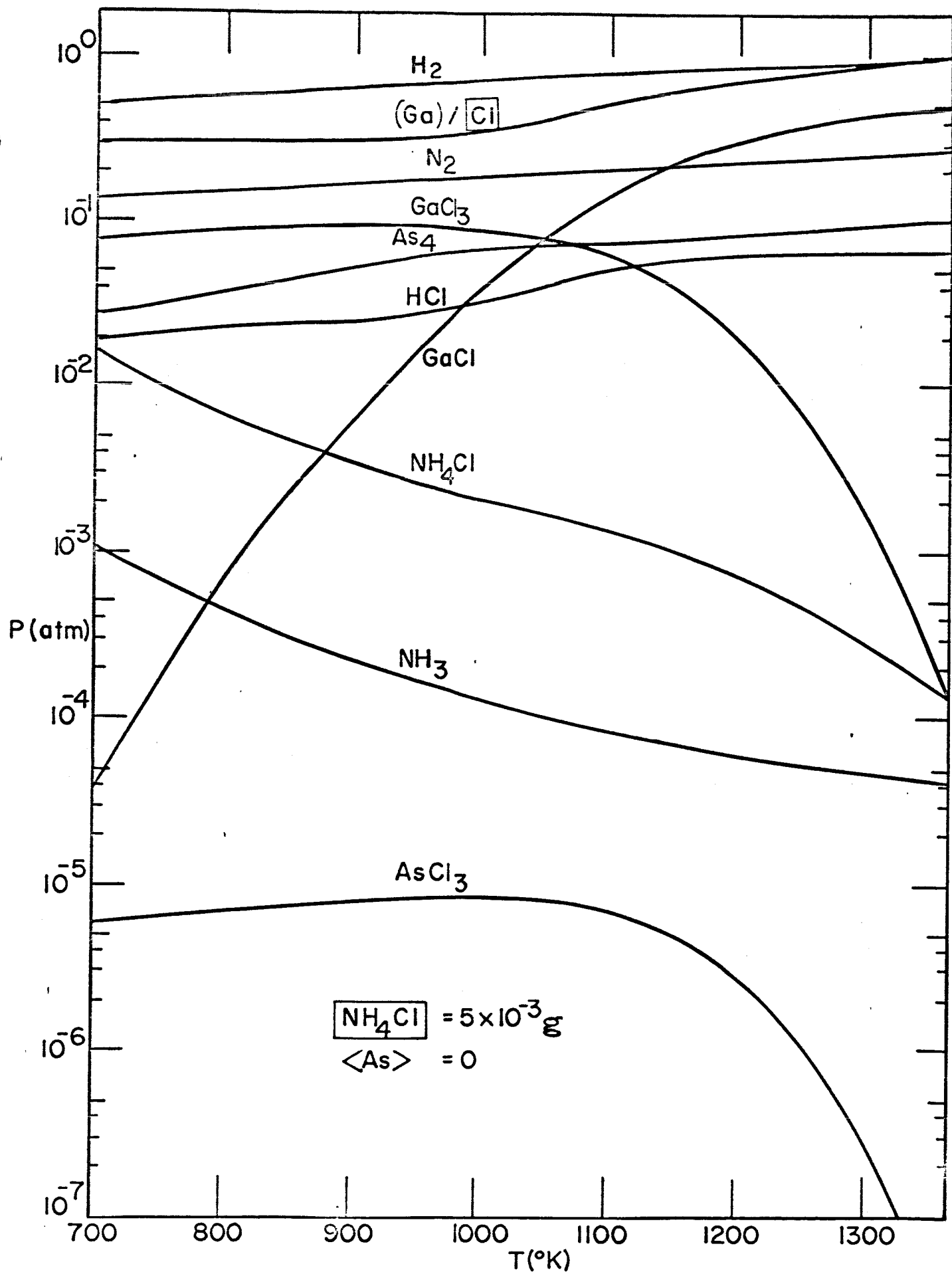
Figure 2. Composition of the gas phase of NH_4Cl -GaAs system vs. temperature with the initial values of NH_4Cl = 5 mg. and no excess arsenic.
