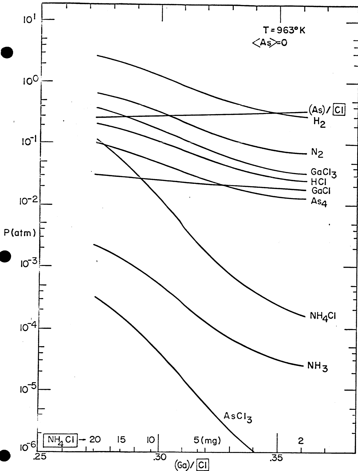
Figure 5. Composition of the gas phase vs. the composition ratio (\text{Ga}) / \text{Cl} and \text{NH}_4\text{Cl} at T = 963^{\circ}\text{K} and no cross section.
