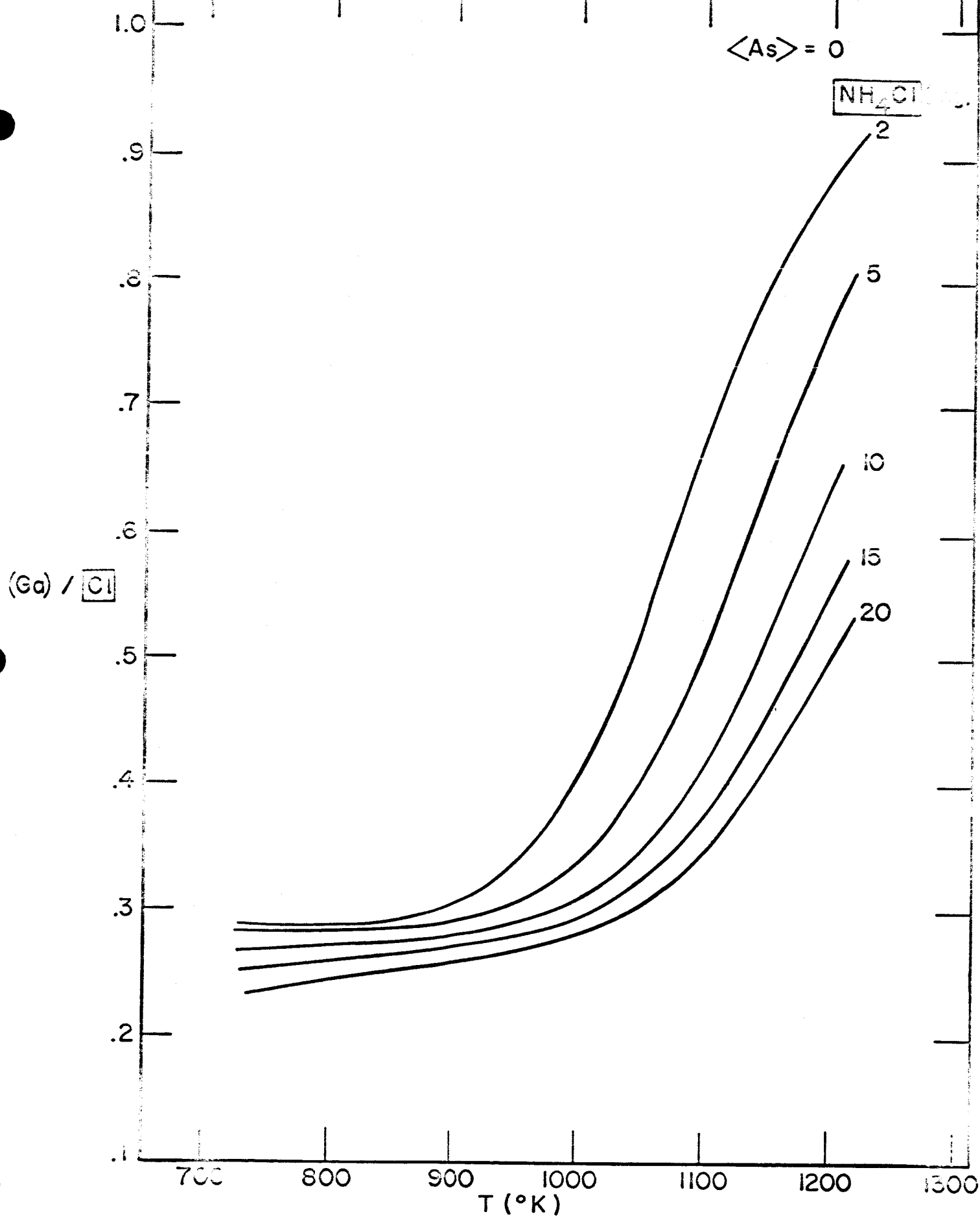
Figure 1. (Ga) / [Cl] vs. T for various NH_4Cl concentrations. \langle As \rangle = 0 .
