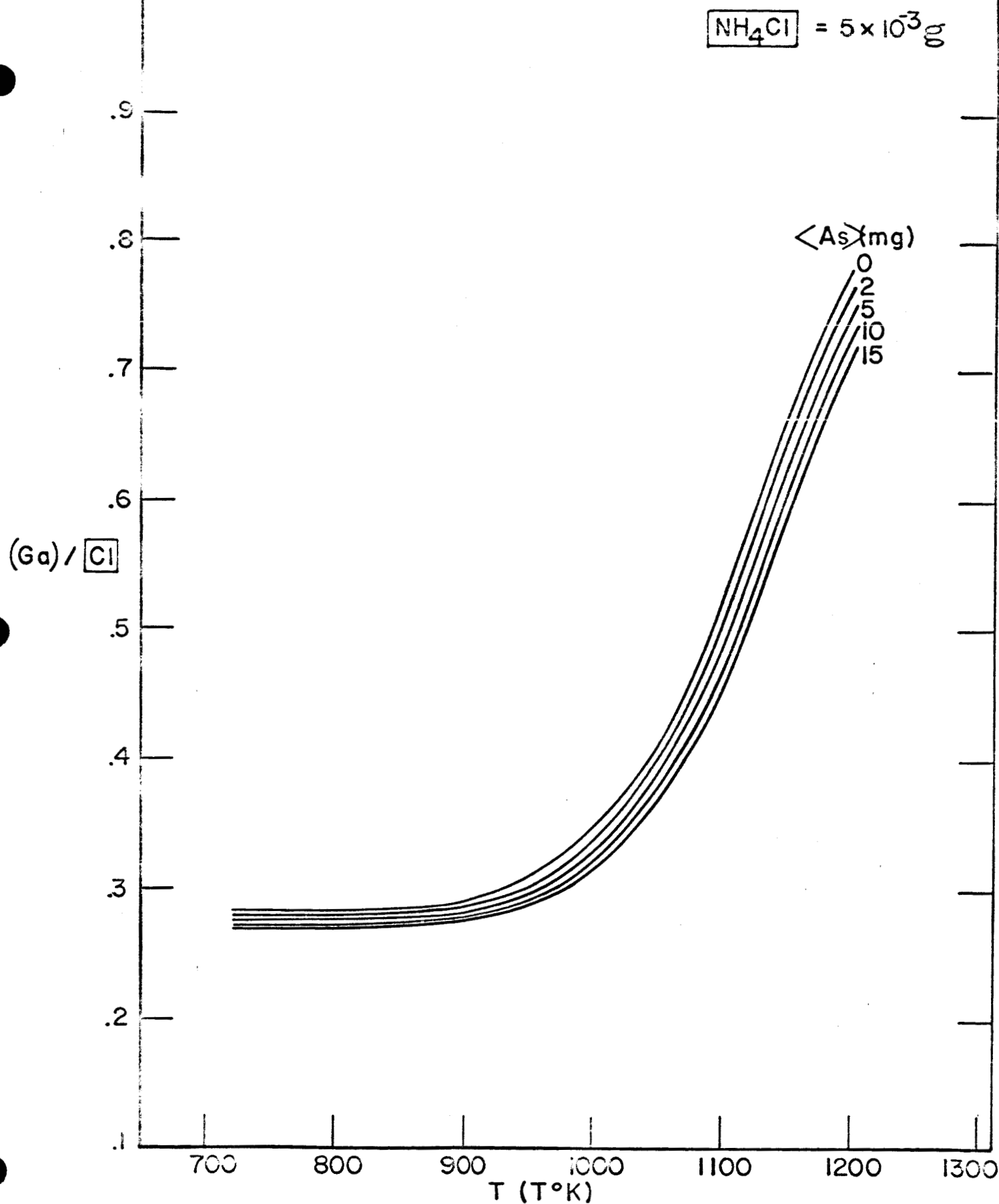
Figure 7. Component (Ga)/(Cl) vs. temperature with various initial values of \langle As \rangle and at NH_4Cl = 5 \times 10^{-3} g .
