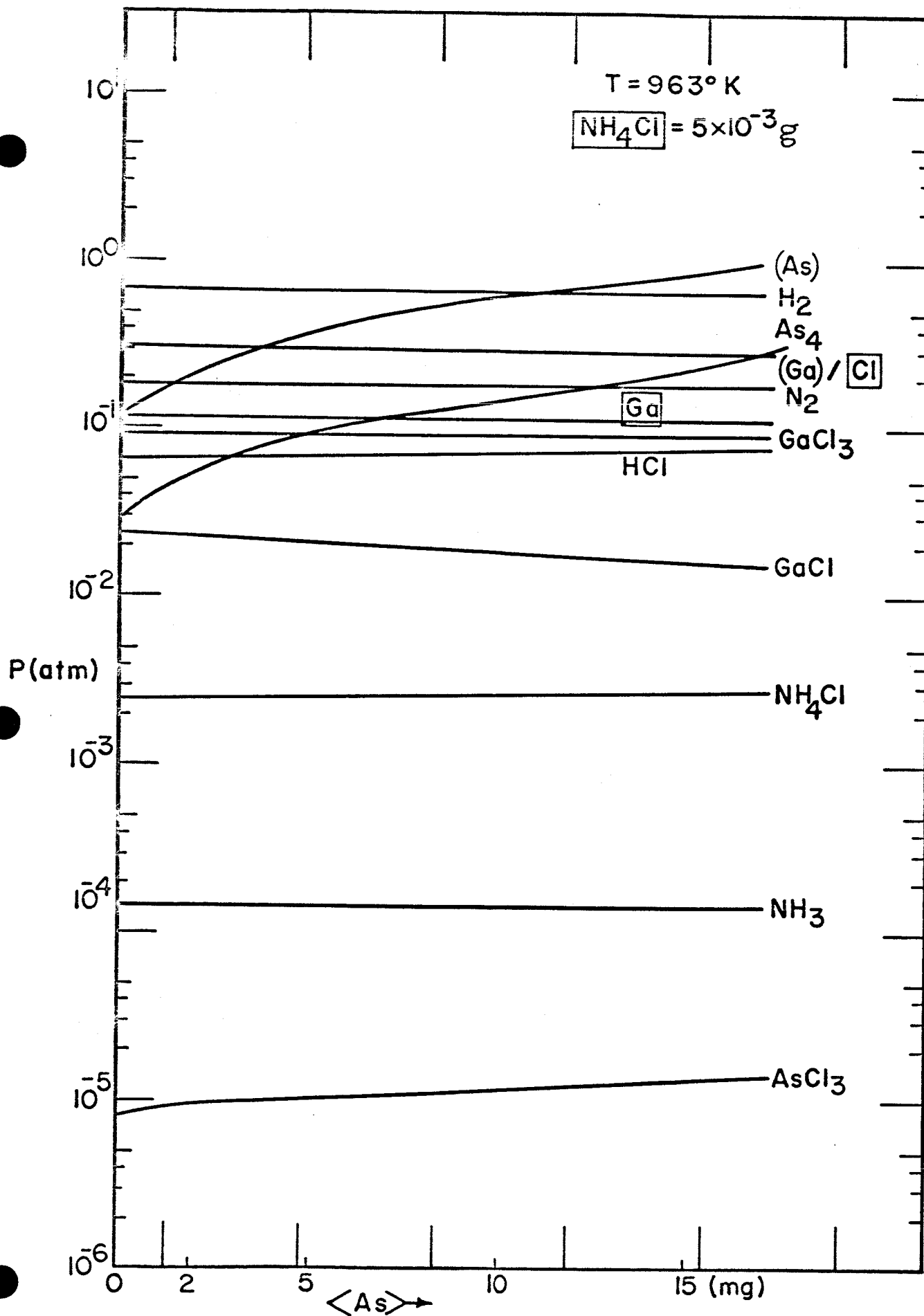
Figure 4. Composition of \text{H}_2 gas vs. \langle \text{As} \rangle at T = 963^{\circ}\text{K} and \text{NH}_4\text{Cl} = 5 \text{ mg} .
