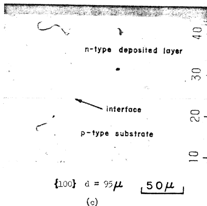
Figure 22. Photomicrographs of the cleaved {110} surface of (a) Zn doped n-type grown layer on the n-type {111}B surface with \text{NH}_4\text{I} . Note Zn diffusion of 5.2\mu beyond interface. (b) Zn doped p-type grown layer on the n-type {100} with \text{NH}_4\text{Cl} . 2\mu Zn diffusion beyond interface. (c) Te doped n-type grown layer on the Zn doped p-type {100} with \text{NH}_4\text{Cl} .
