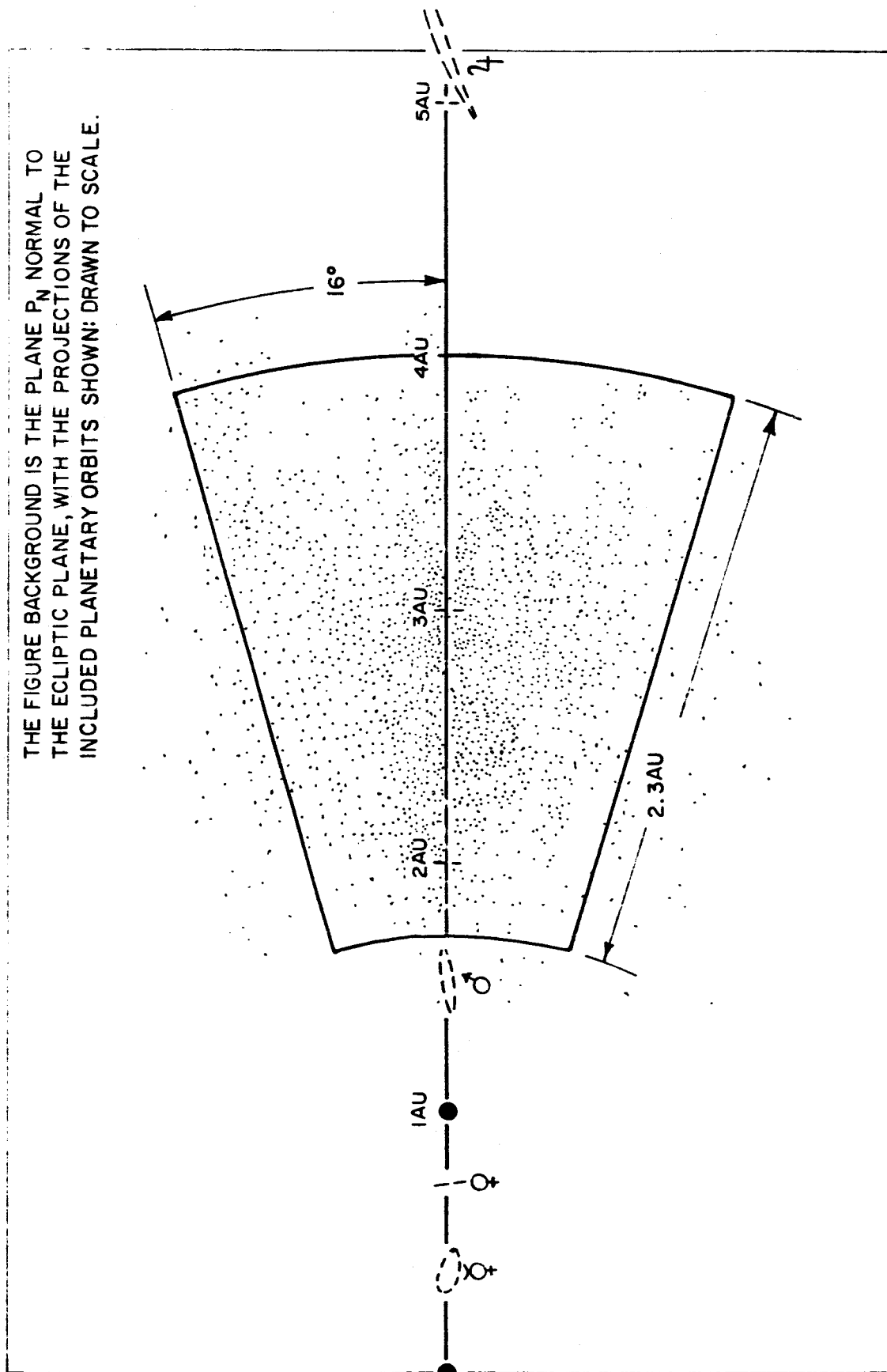
FIGURE 7.1. DISTRIBUTION OF 1500 NUMBERED ASTEROIDS IN \beta AND R ON 3/20/73
