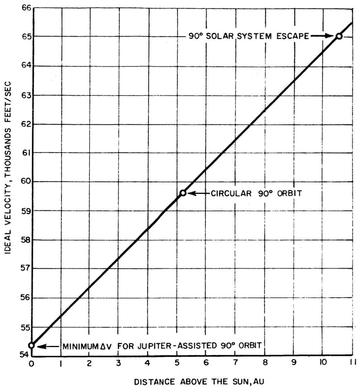
FIGURE 4.2. DISTANCE ABOVE THE SUN FOR JUPITER-ASSISTED 90° ORBITS
