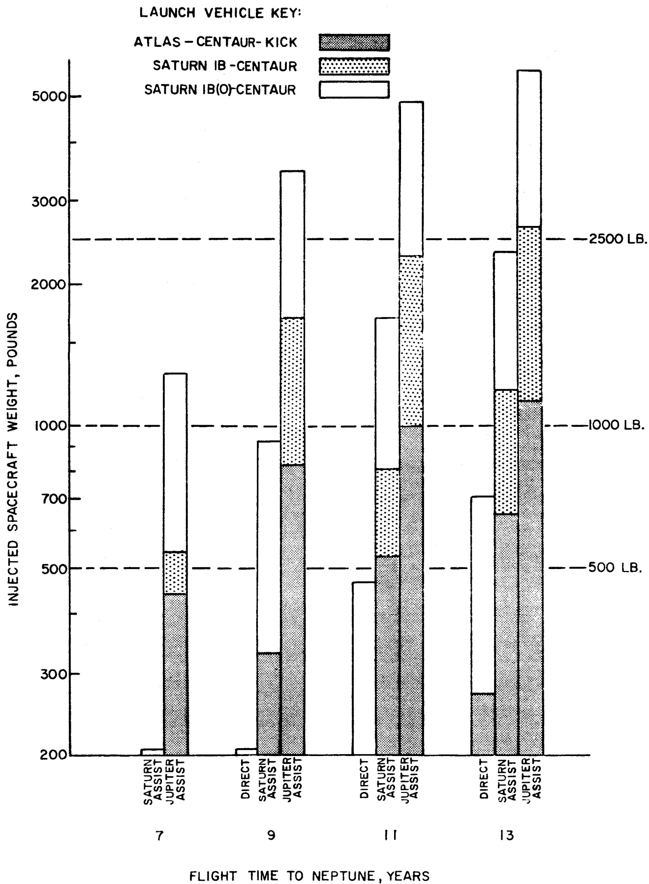
FIGURE 3.3. SPACECRAFT WEIGHT BAR CHART FOR NEPTUNE MISSIONS
