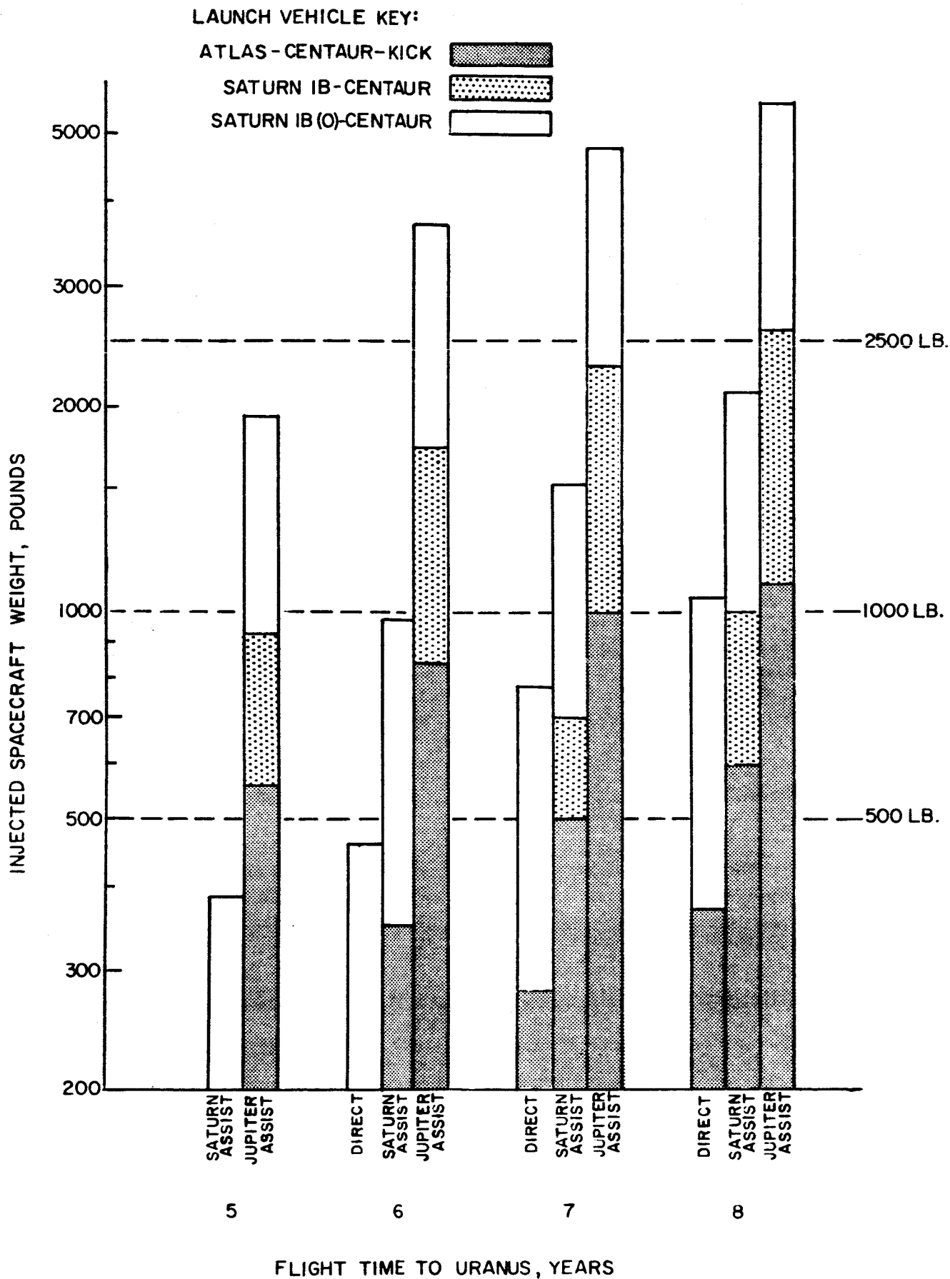
FIGURE 3.2. SPACECRAFT WEIGHT BAR CHART FOR URANUS MISSIONS
