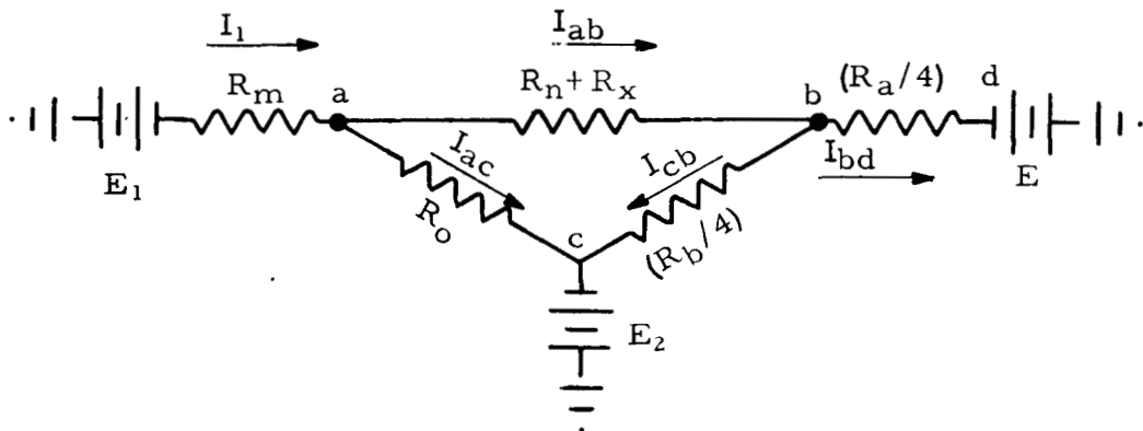
Figure B-8. Circuit of Figure B-7 Modified by \Delta -Y Transformation of Loop a-c-f
