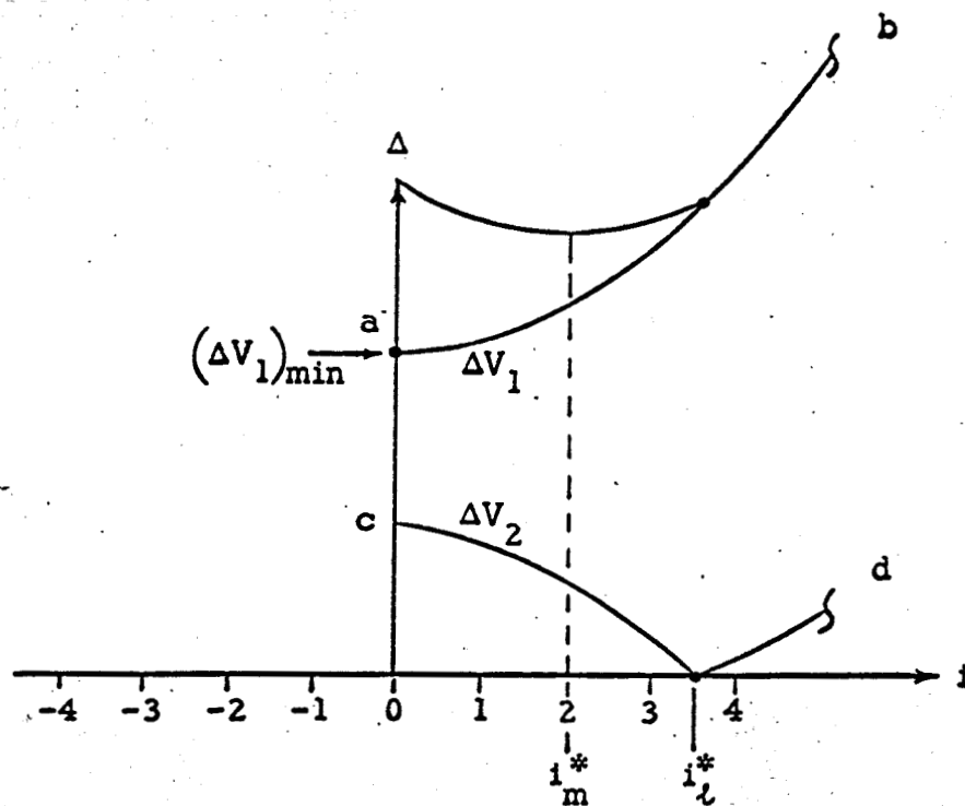
Figure 5 Graphical Representation Velocity Increment Equation
