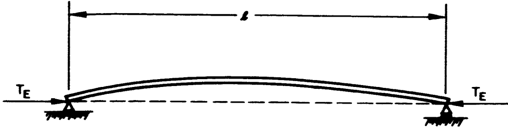
Fig. 2 Pin-Ended Beam under Axial Load
