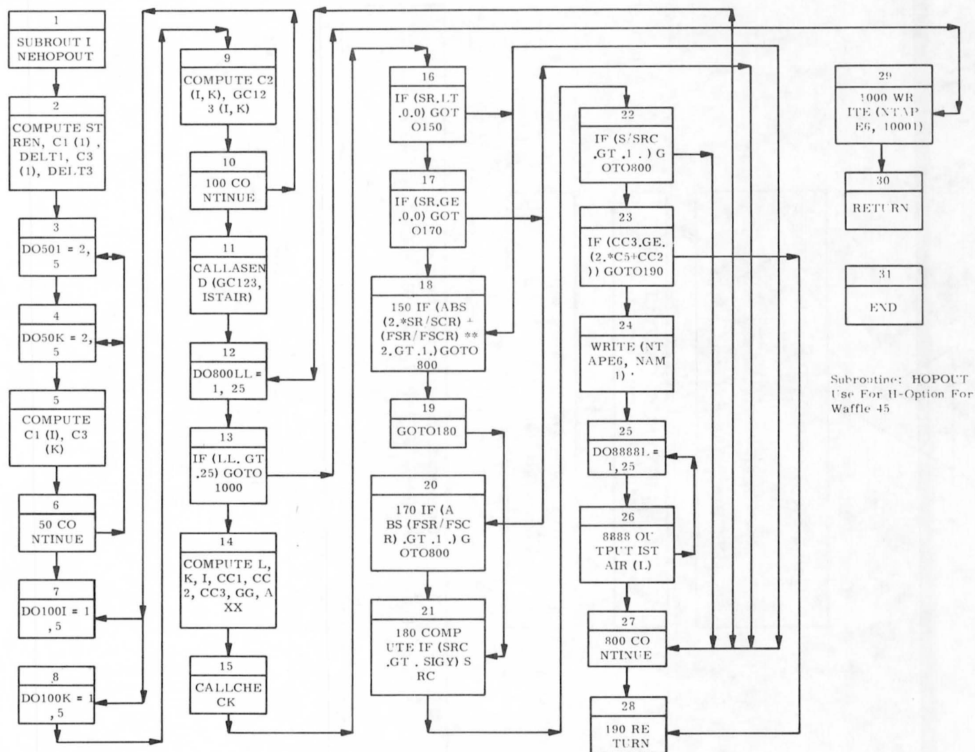
Figure 4-27. HOPOUT Subroutine Flow Chart
