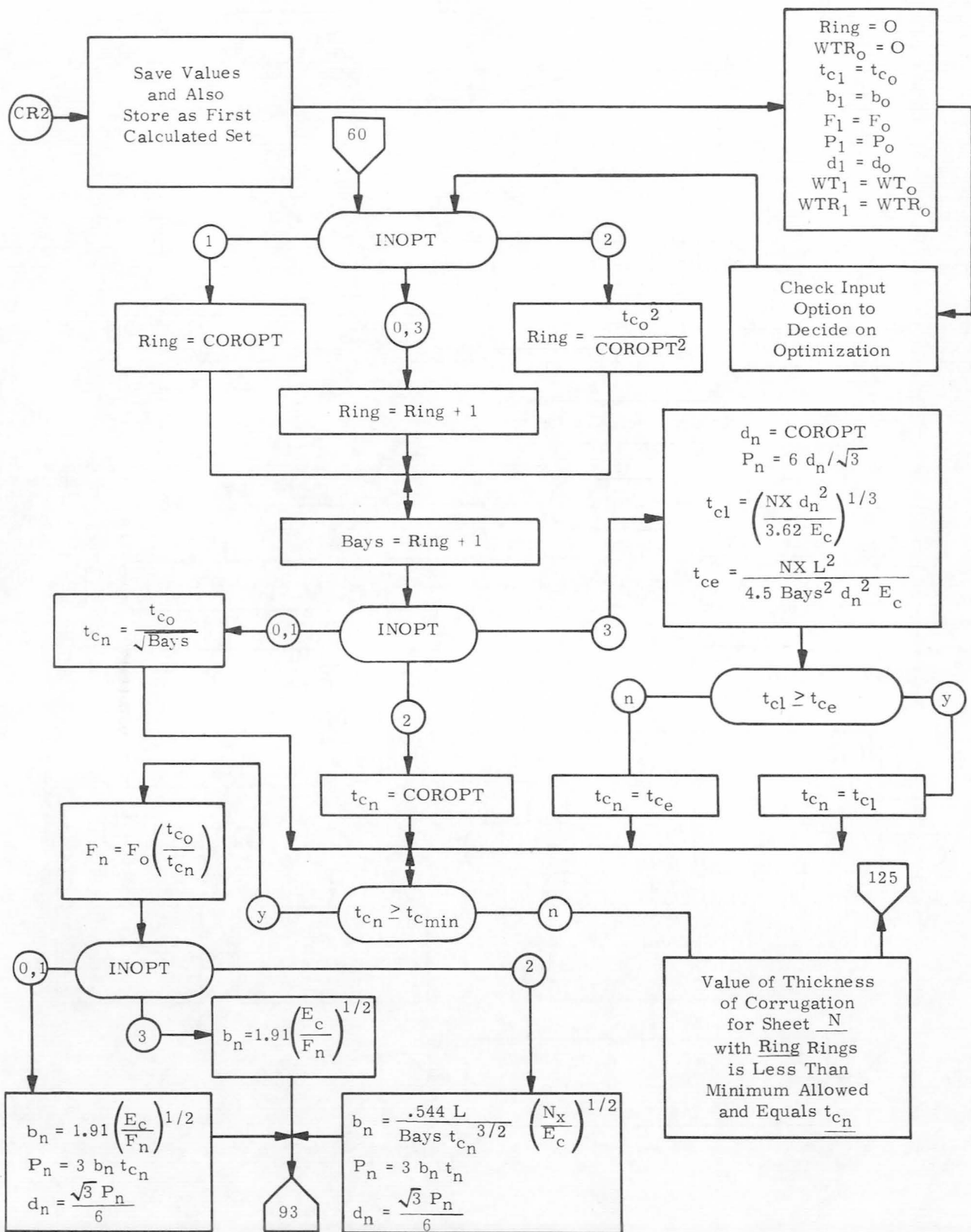
Figure 4-50. CR1MAS Subroutine Flow Chart (Sheet 2 of 4)
