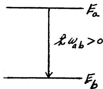
Figure 3 Energy Levels
