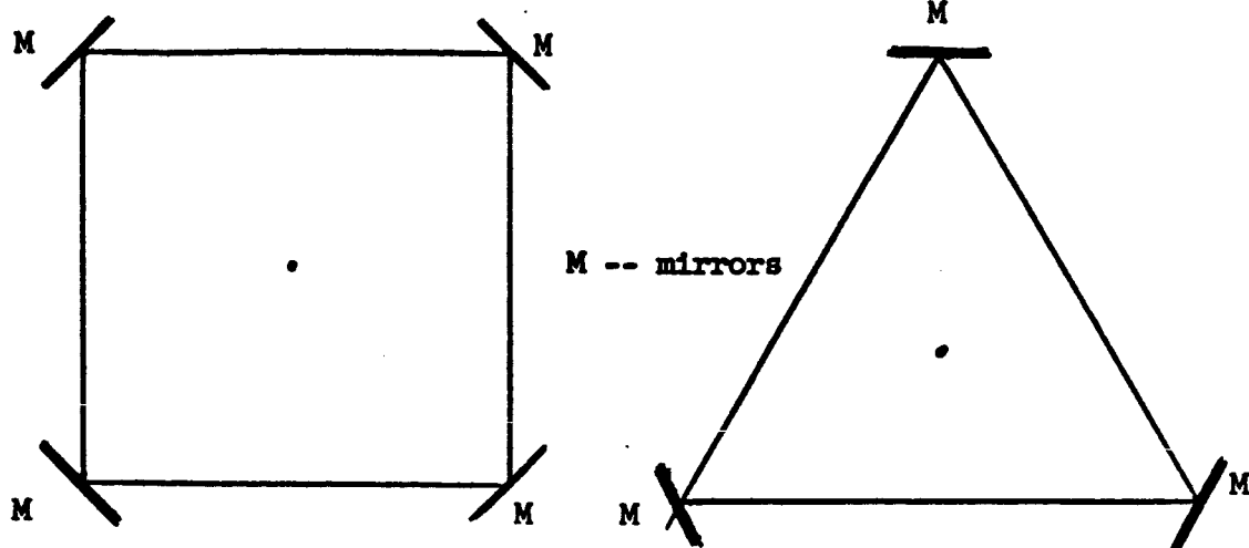
Figure 1 Typical Cavity Designs
