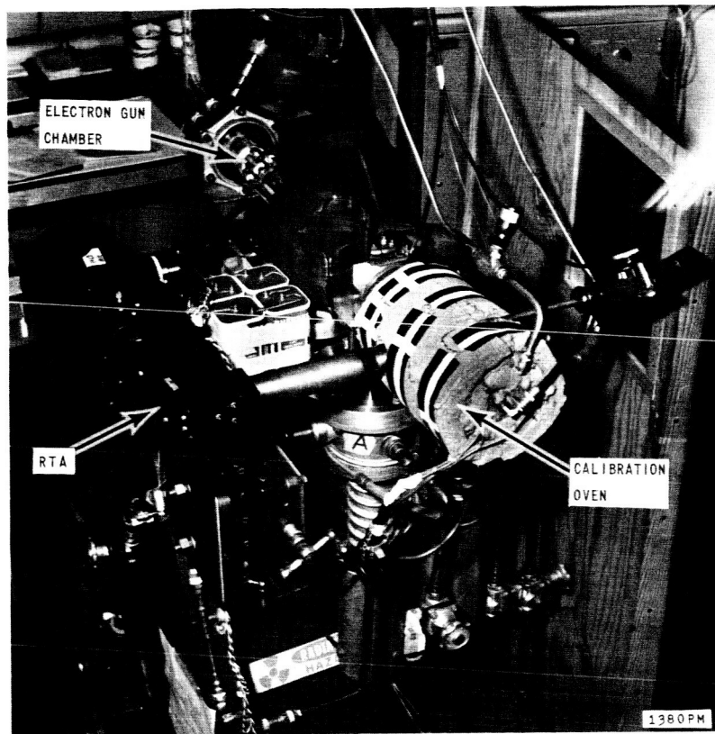
a. CALIBRATION ARRANGEMENT OF THE RTA
