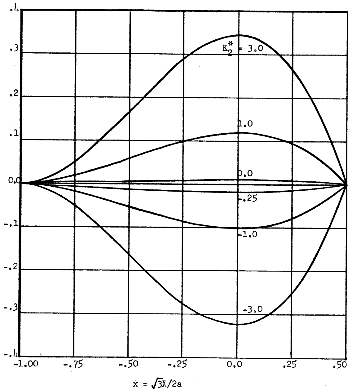
Figure (3) - Dimensionless temperature profiles along y = 0 for steady laminar forced convection
