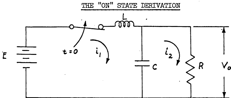
FIGURE 4.36 Equivalent Circuit for "On" State
