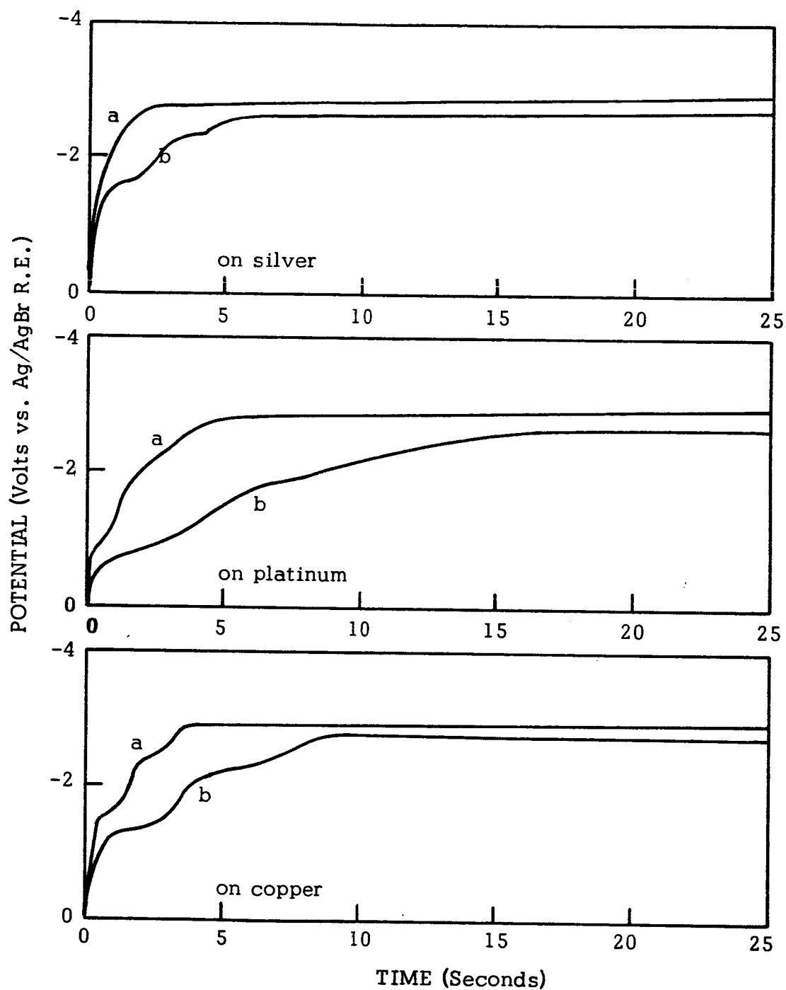
Figure 15: CHRONOPOTENTIOMETRIC SURFACE EFFECTS IN PC/LiBr On substrate indicated, in PC/0.1 M LiBr. a = 2 \text{ mA cm}^{-2} ; b = 0.8 \text{ mA cm}^{-2}
