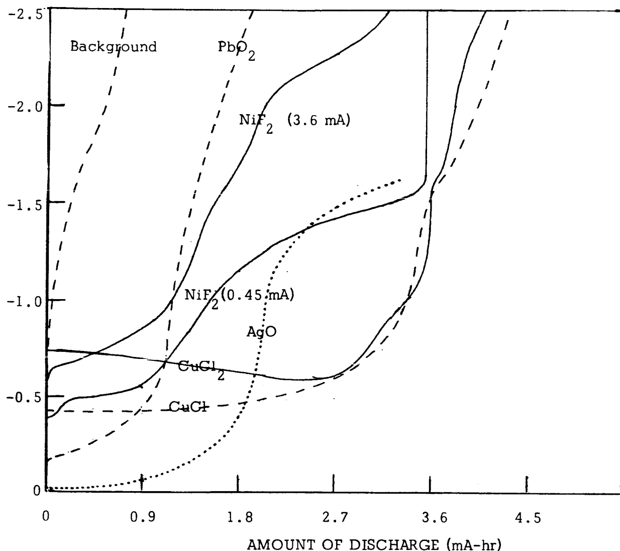
Figure 30: CATHODIC DISCHARGE OF VARIOUS MATERIALS IN PROPYLENE CARBONATE Discharge of 0.85 \text{ cm}^2 electrodes. Mixes were in weight ratio 6:3:1 Ag:Cathode Salt: \text{LiClO}_4 . Theoretical capacities were 7.2 mA-hr. Except where indicated, all discharges were done at 3.6 mA. Potentials are given with respect to a silver disc R.E. against which the potential of a lithium electrode in the same solution is about -3.1 V. Discharges were performed in propylene carbonate, 1 M in \text{LiClO}_4 . Under the conditions prevailing in these experiments, the iR drop for reductions at 3.6 mA is about 0.5 V.
