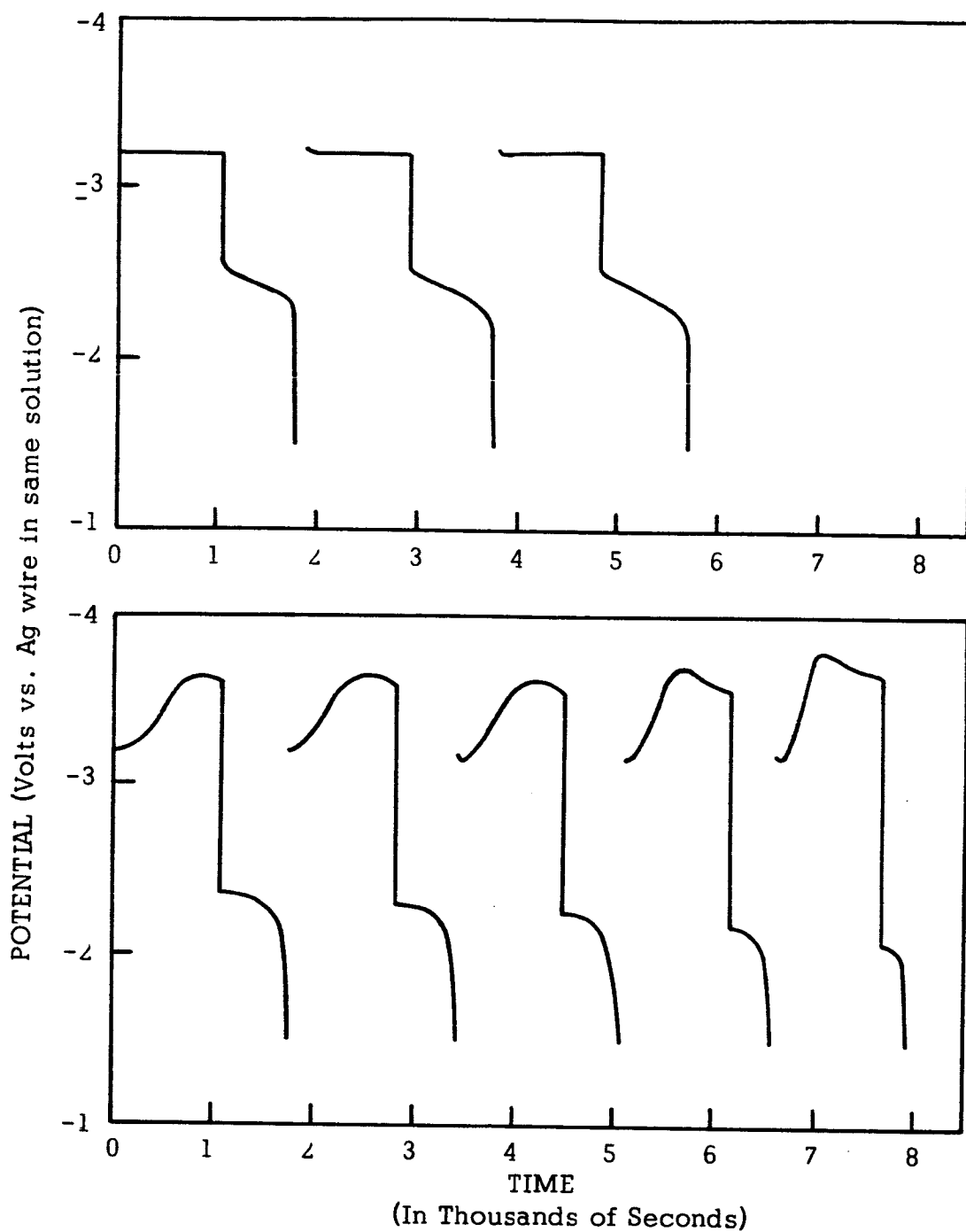
Figure 1: LITHIUM CYCLING IN PC/0.5 M \text{LiAlCl}_4
