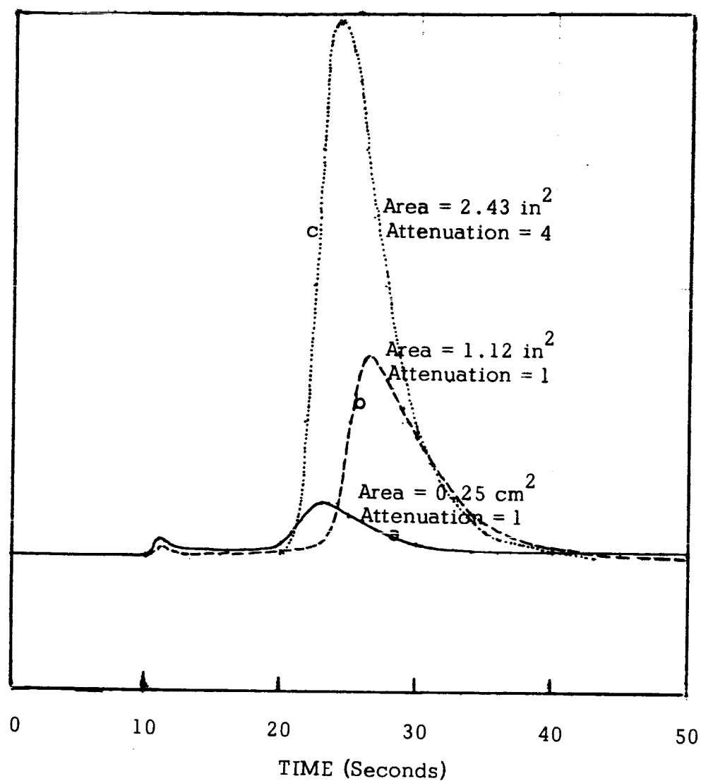
Figure 33 : VAPOR PHASE CHROMATOGRAM OF WATER IN PROPYLENE CARBONATE Performed with 0.8 microliter samples. Column temperature = 200^{\circ} \text{C} .
