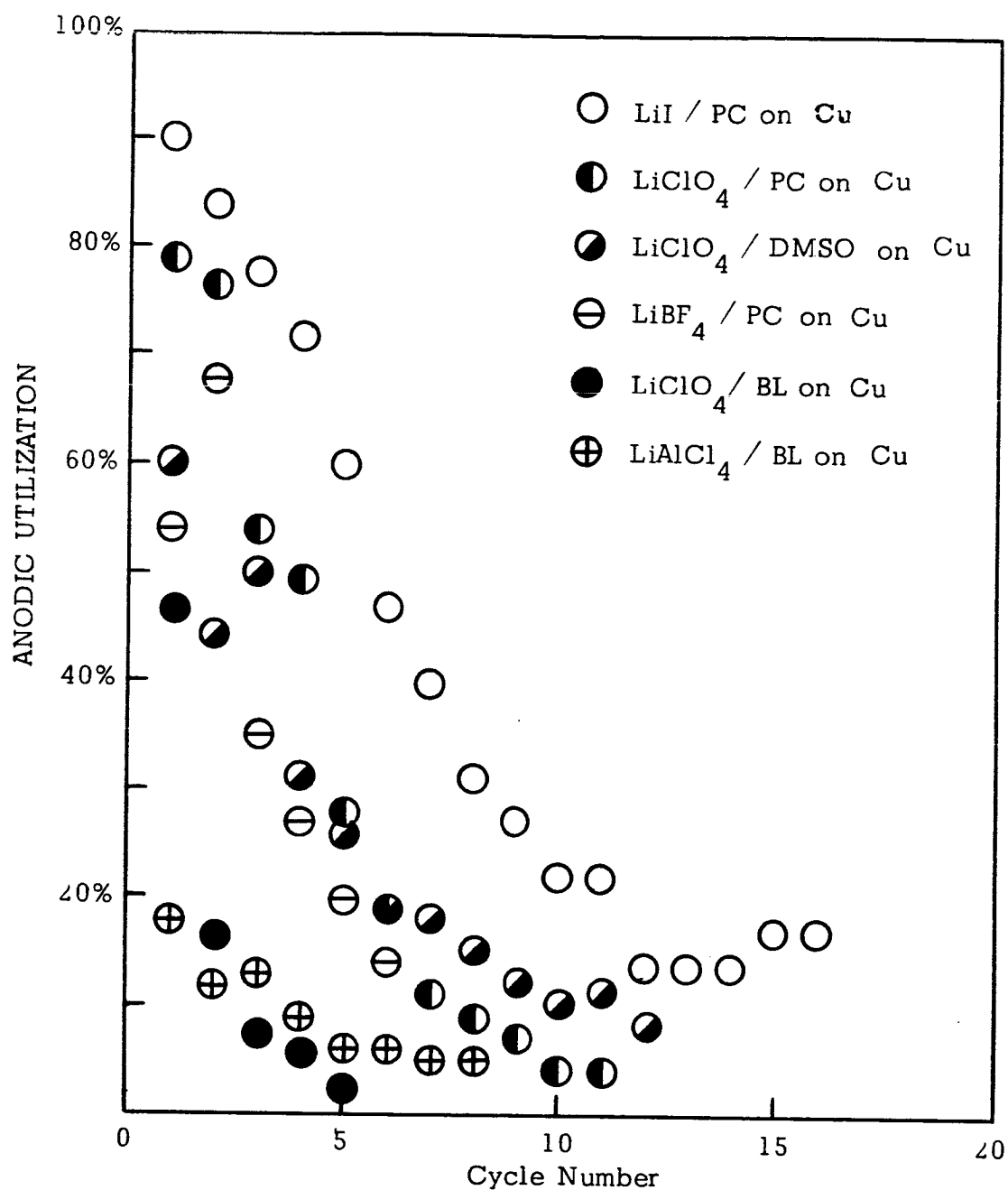
Figure 3: LITHIUM CYCLING
