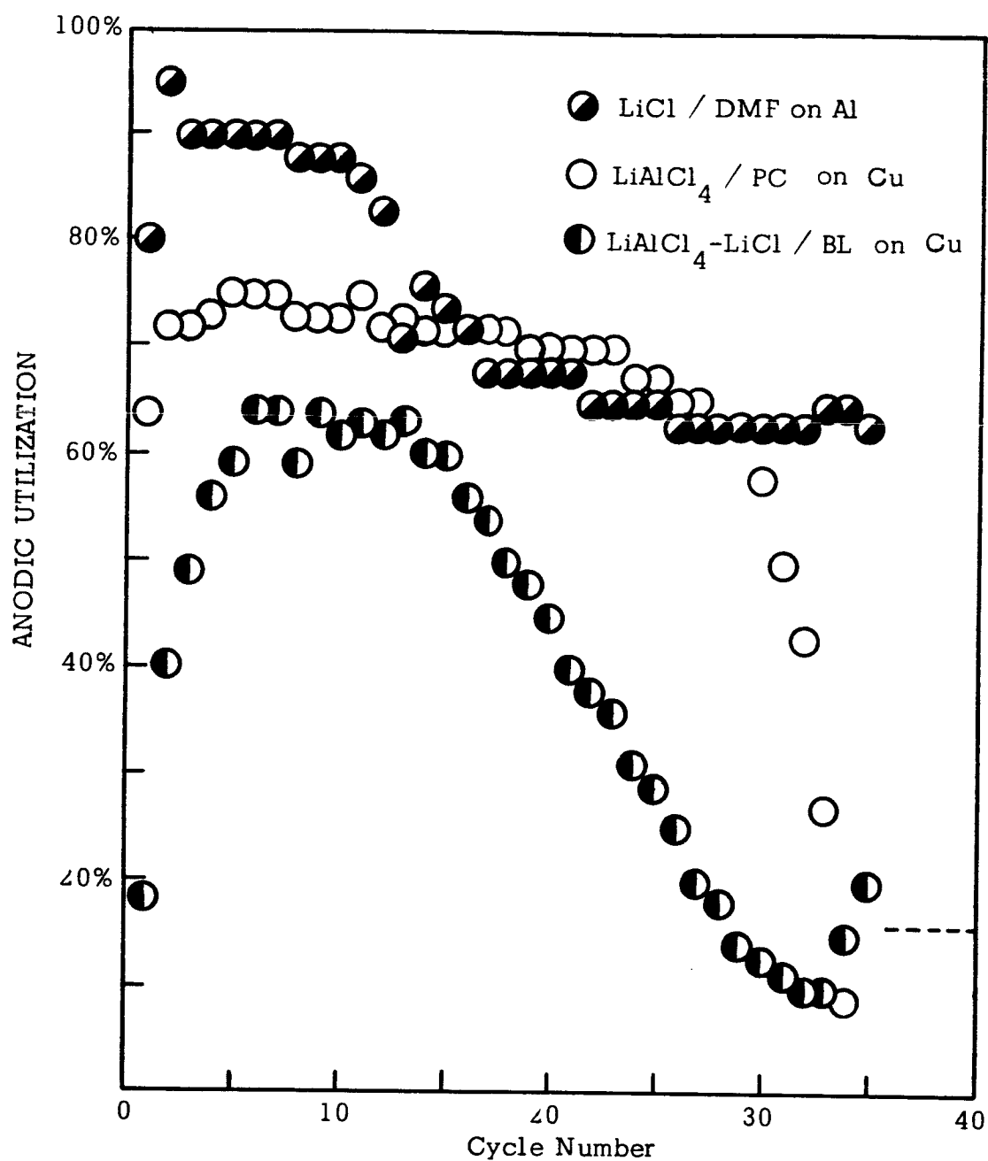
Figure 4: LITHIUM CYCLING
