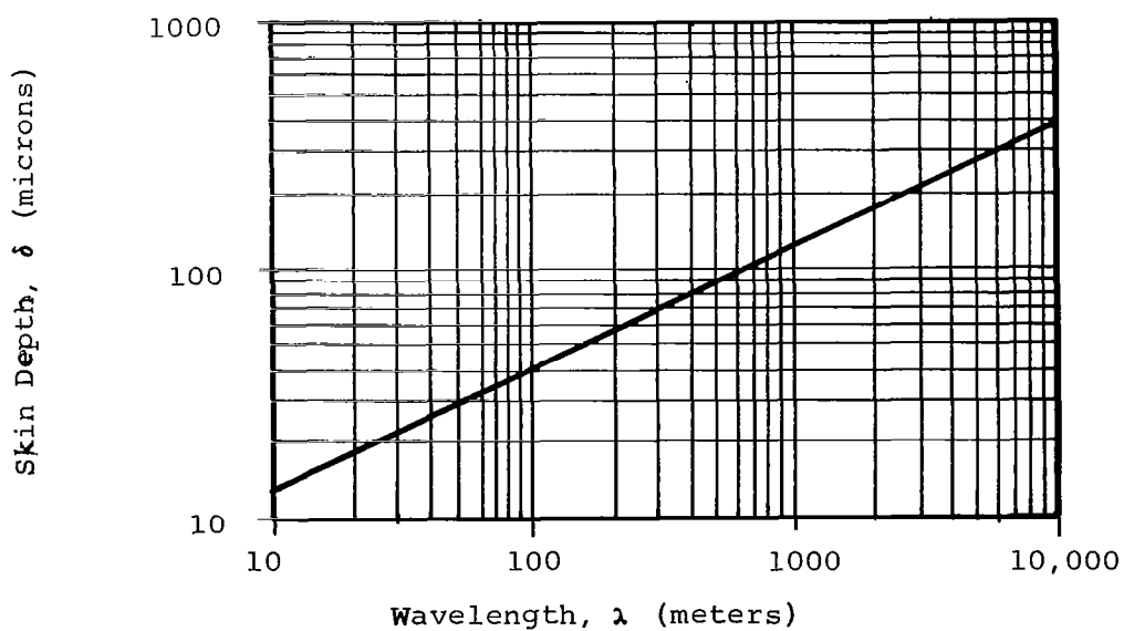
Figure 5. - Skin Depth in Copper.
