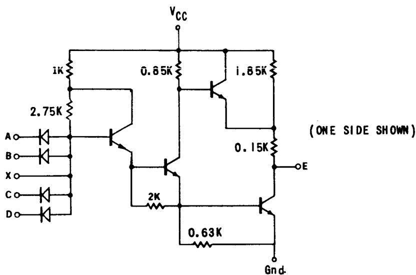
b. FAIRCHILD 932 DUAL NAND BUFFER ELEMENT
