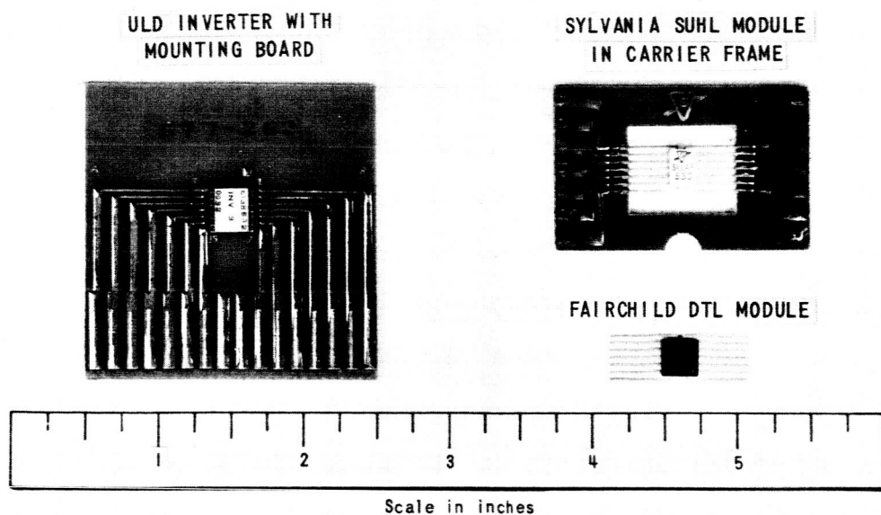
a. ULD, SYLVANIA AND FAIRCHILD MODULES WITH SCALE
