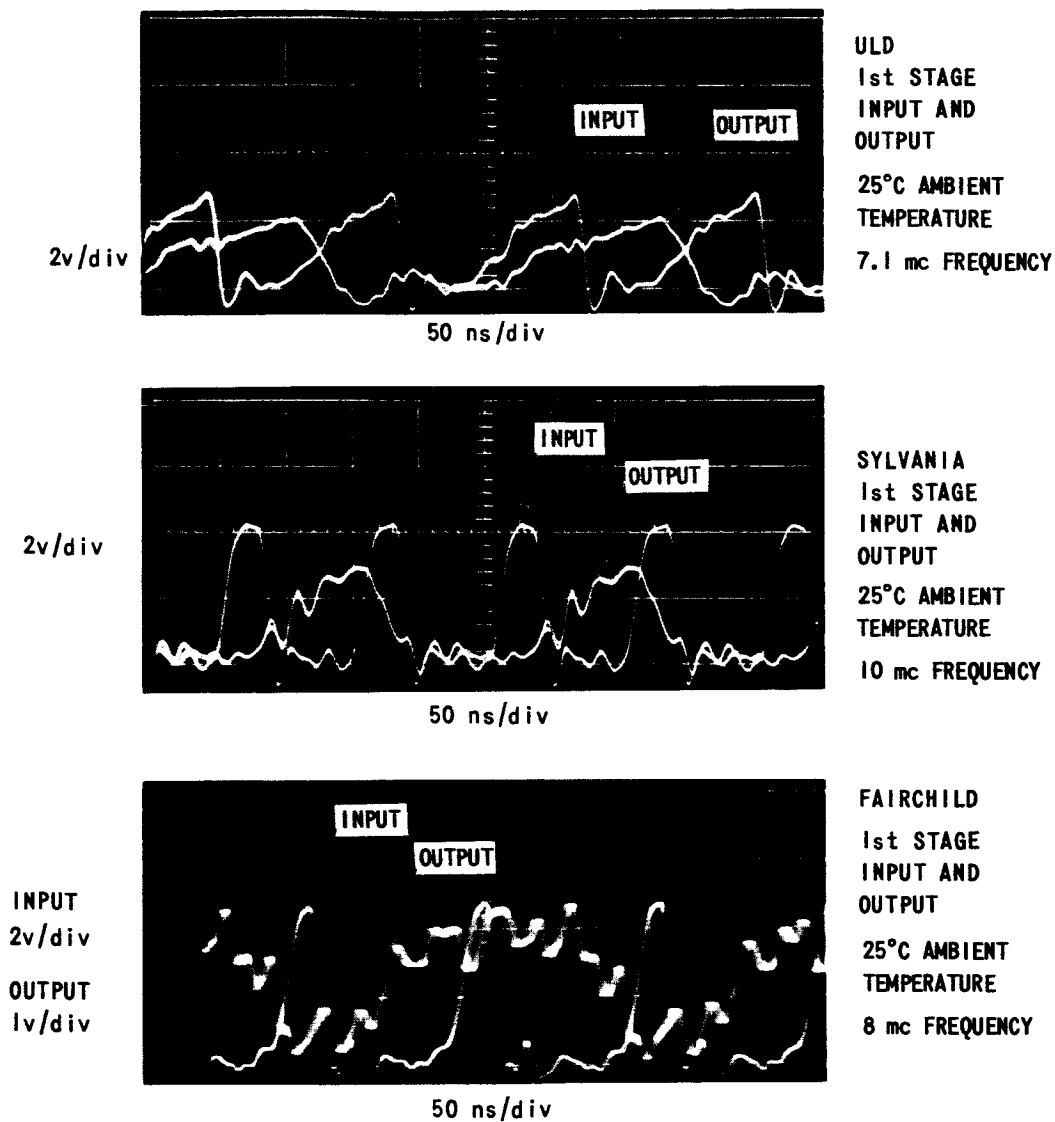
Figure 4.16 INPUT AND OUTPUT WAVEFORMS OF RIPPLE COUNTER FIRST STAGE AT MAXIMUM FREQUENCY WITH STANDARD VOLTAGES
