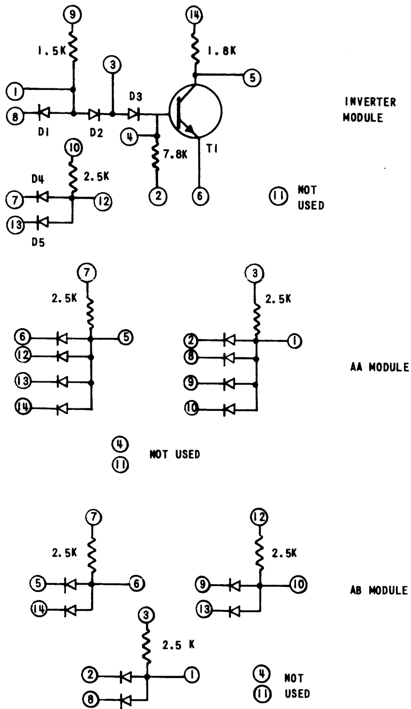
Figure 2.2 CIRCUIT AND PIN CONNECTIONS OF ULD INVERTER, AA AND AB MODULES
