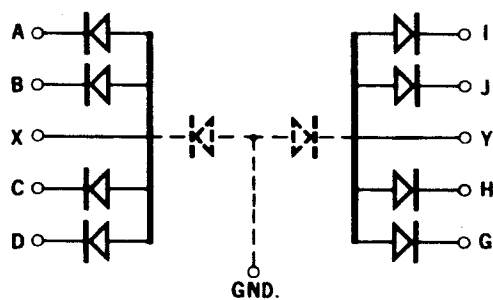
c. FAIRCHILD 933 AND EXPANDER ELEMENT
