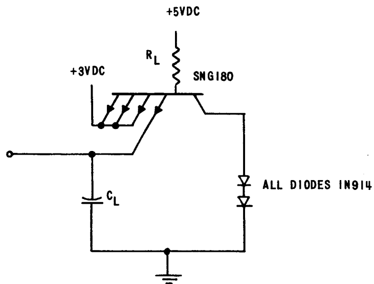
b. SIMULATED LOAD CIRCUIT FOR SYLVANIA TTL CIRCUITS
