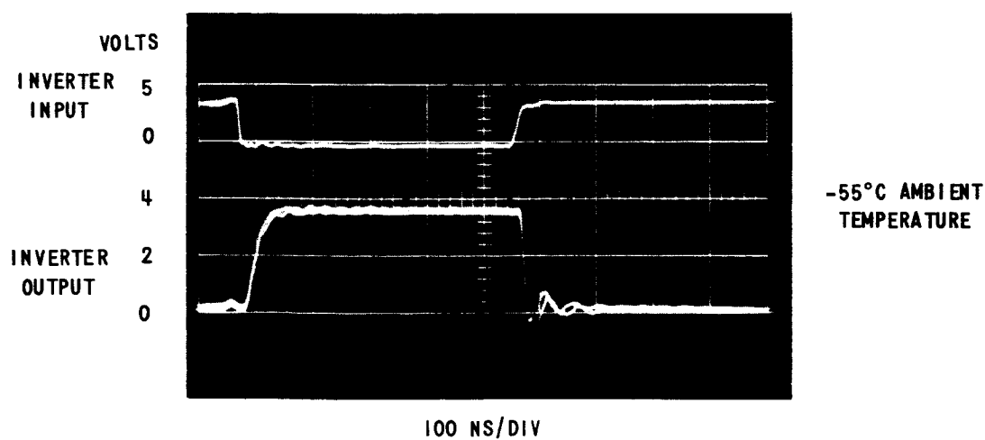
Figure 2.21 DYNAMIC COMPARISON OF SYLVANIA ACTUAL (SNG-14) AND SIMULATED LOADS FOR A FANOUT OF 4
