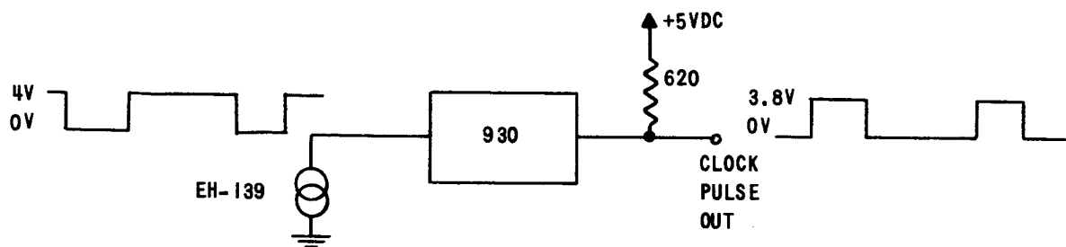
Figure 3.9 FAIRCHILD CLOCK PULSE GENERATOR
