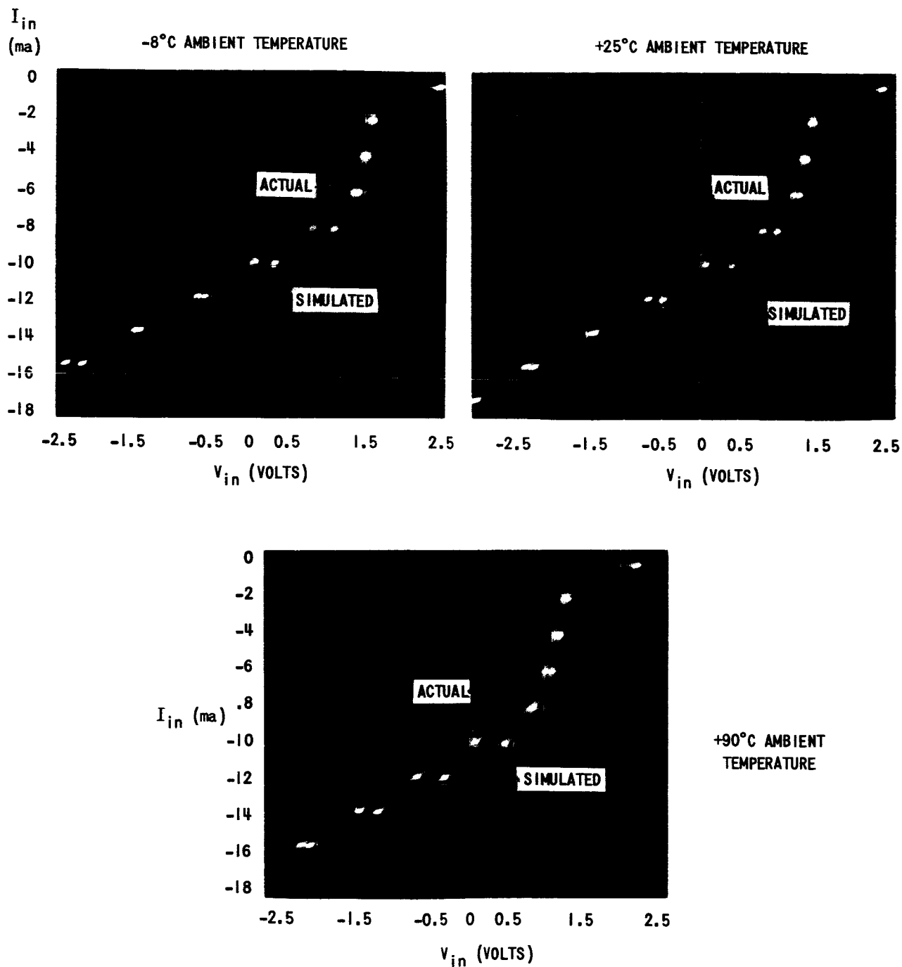
Figure 2.19 STATIC COMPARISON OF ULD ACTUAL AND SIMULATED LOADS FOR A FANOUT OF 3
