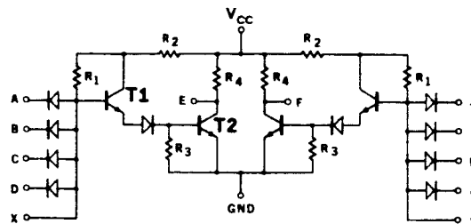
a. FAIRCHILD 930 DUAL NAND GATE
