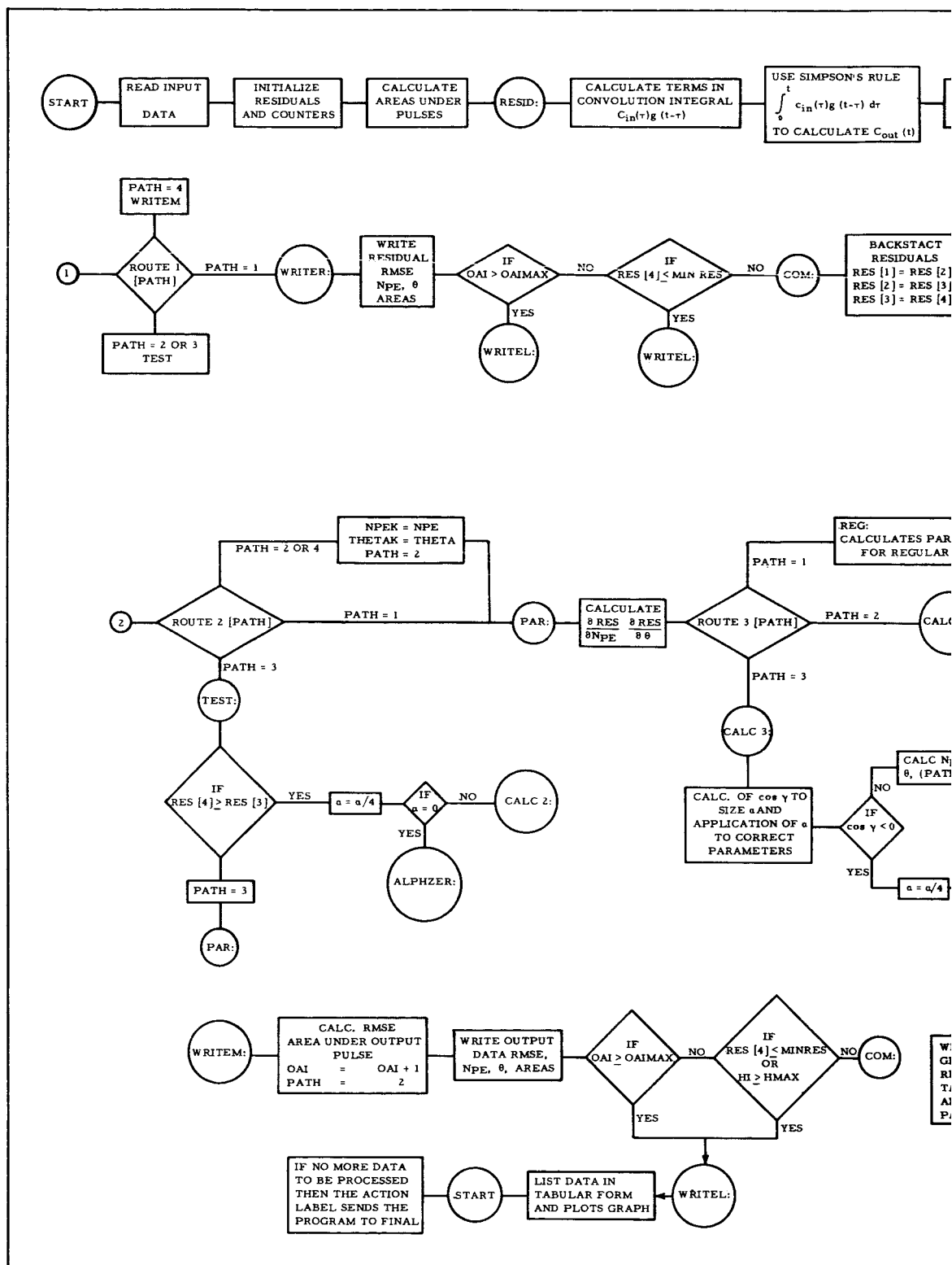
Figure 2. Flow Diagram of Time Domain Analysis Program
