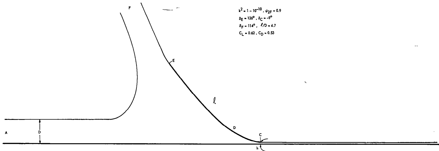
Figure 14. Hydroplaning for Curved Surface Described by Sine-Function ( h/D = 0.11 ).
