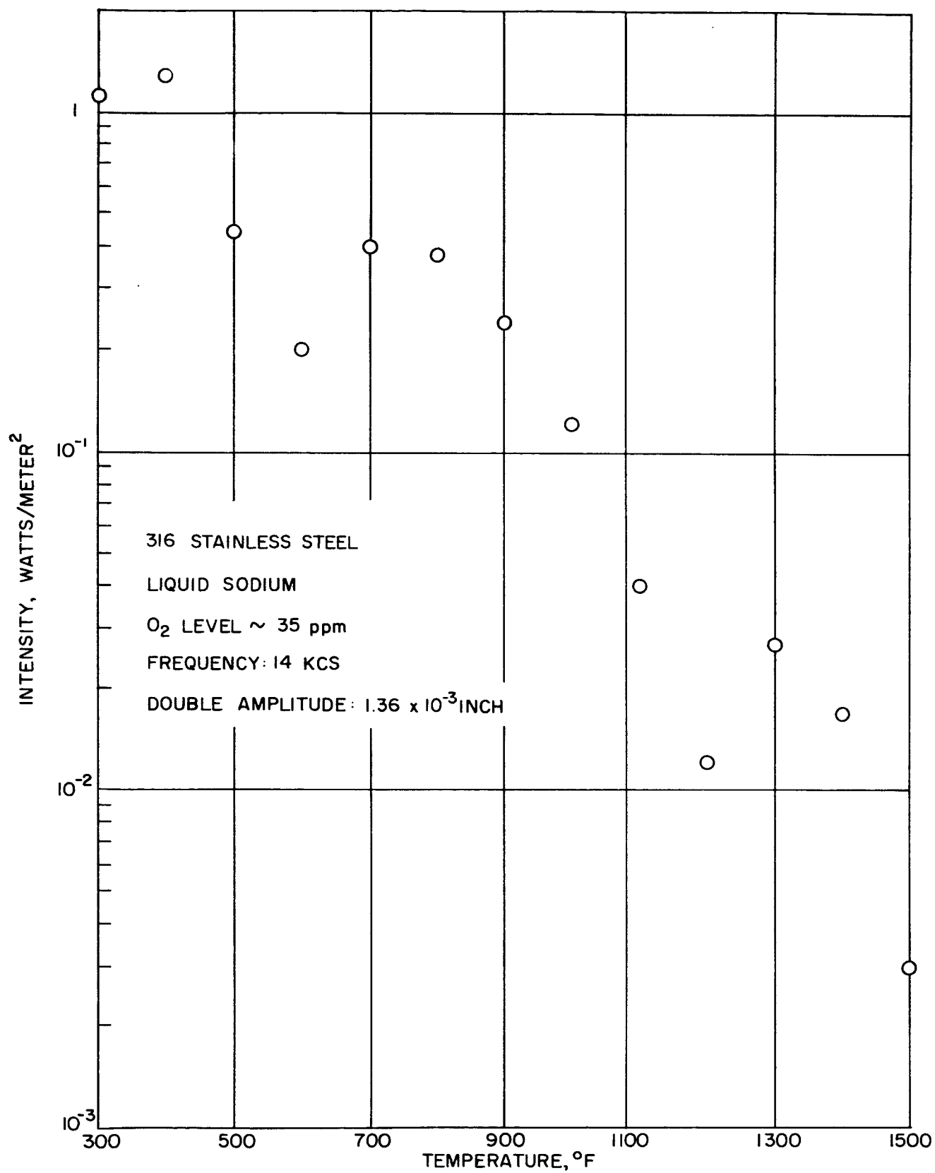
FIGURE 19 - EFFECT OF TEMPERATURE ON THE INTENSITY OF CAVITATION DAMAGE IN LIQUID SODIUM
