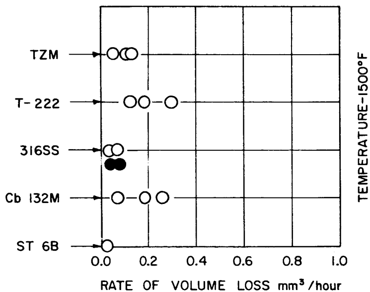
FIGURE 13 - CAVITATION DAMAGE RESISTANCE OF REFRACTORY ALLOYS IN HIGH TEMPERATURE LIQUID SODIUM (1000° AND 1500°F)
