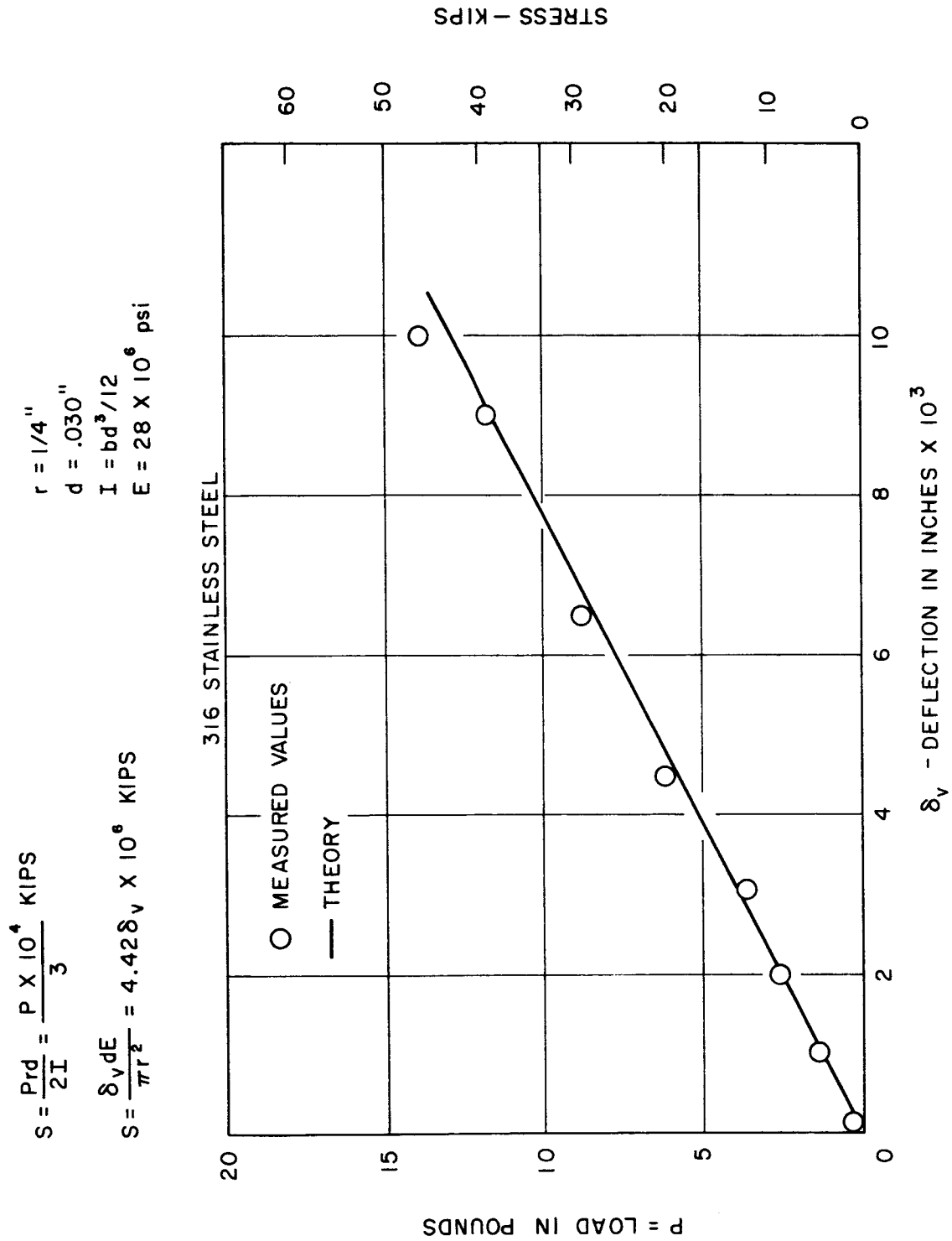
FIGURE 6 - CALIBRATION OF STRESS CORROSION SPECIMEN
