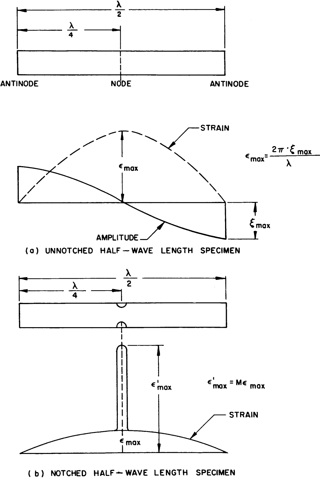
FIGURE 3 - BASIC PRINCIPLE OF HIGH FREQUENCY FATIGUE SPECIMEN DESIGN
