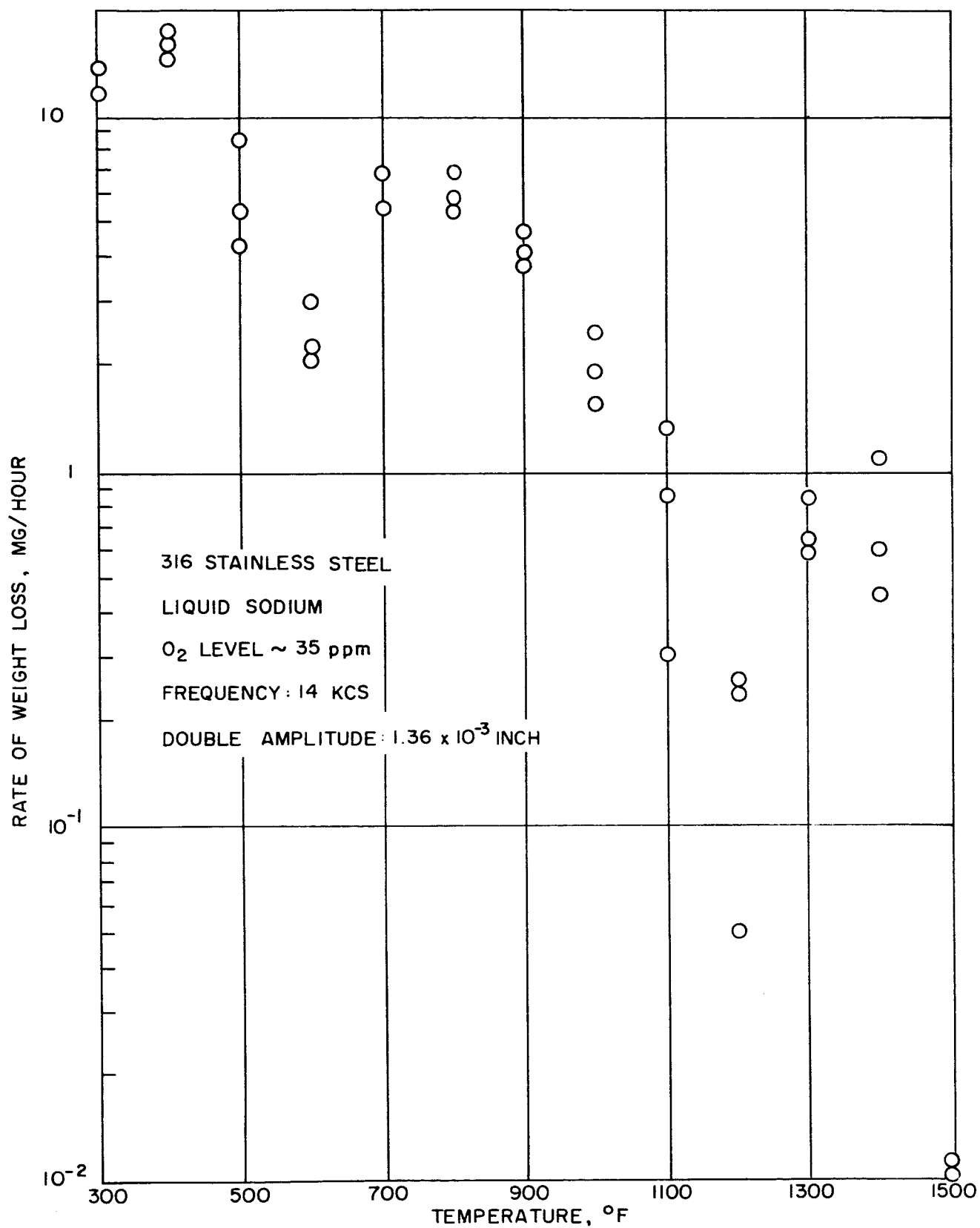
FIGURE 18 - EFFECT OF TEMPERATURE ON THE CAVITATION DAMAGE RATE OF 316 STAINLESS STEEL IN LIQUID SODIUM
