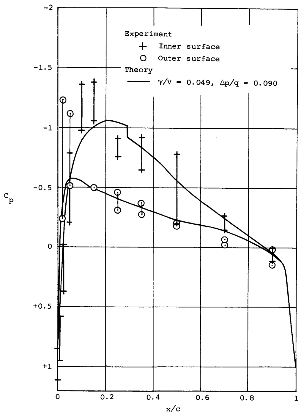
Figure 12.- Pressure distributions for the 7-foot model duct at \alpha = 0^\circ with \beta = 19^\circ, \delta_e = 0^\circ.
