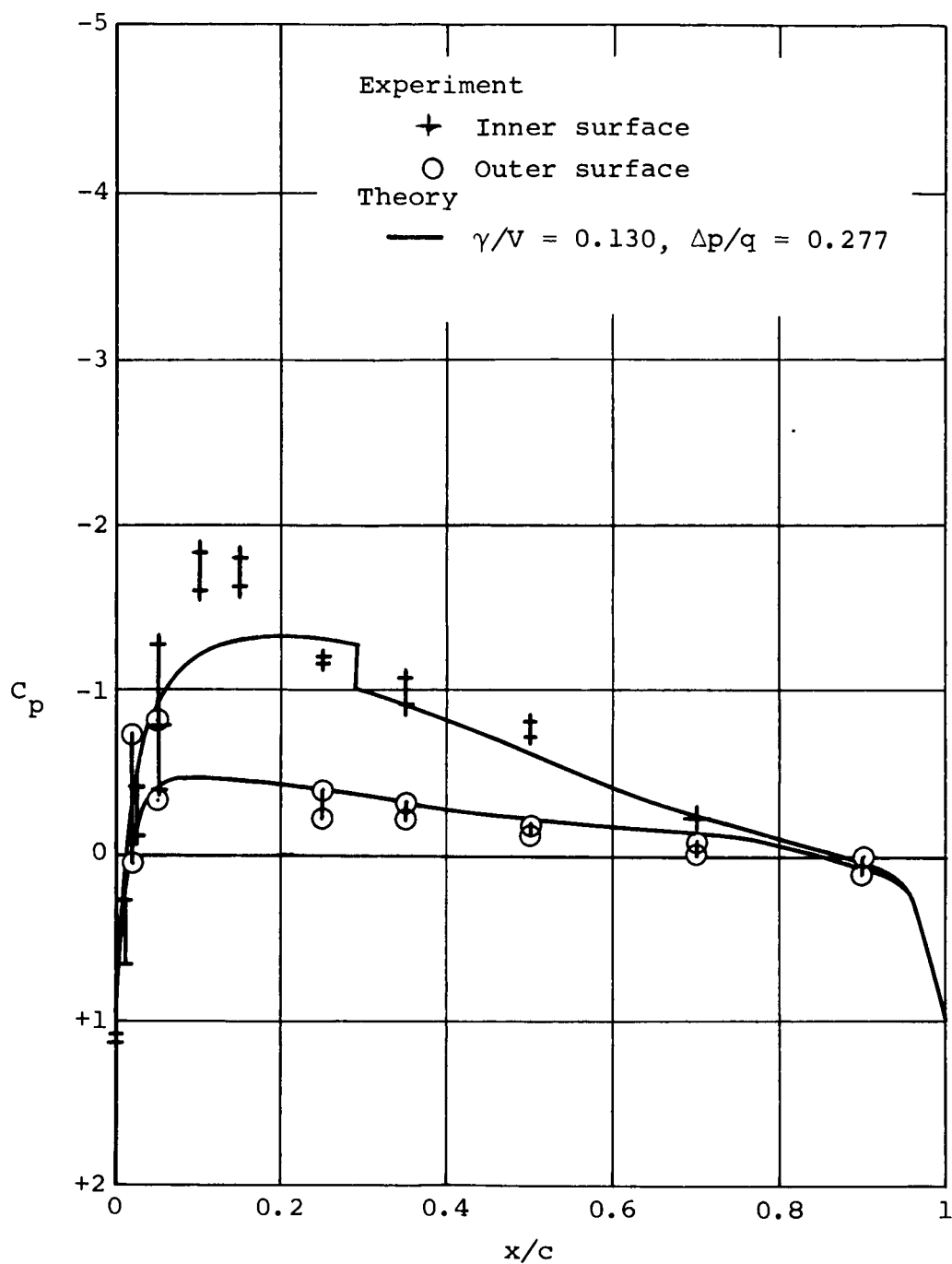
Figure 13.- Pressure distributions for the 7-foot model duct at \alpha = 0^\circ with \beta = 19^\circ , elevon off.
