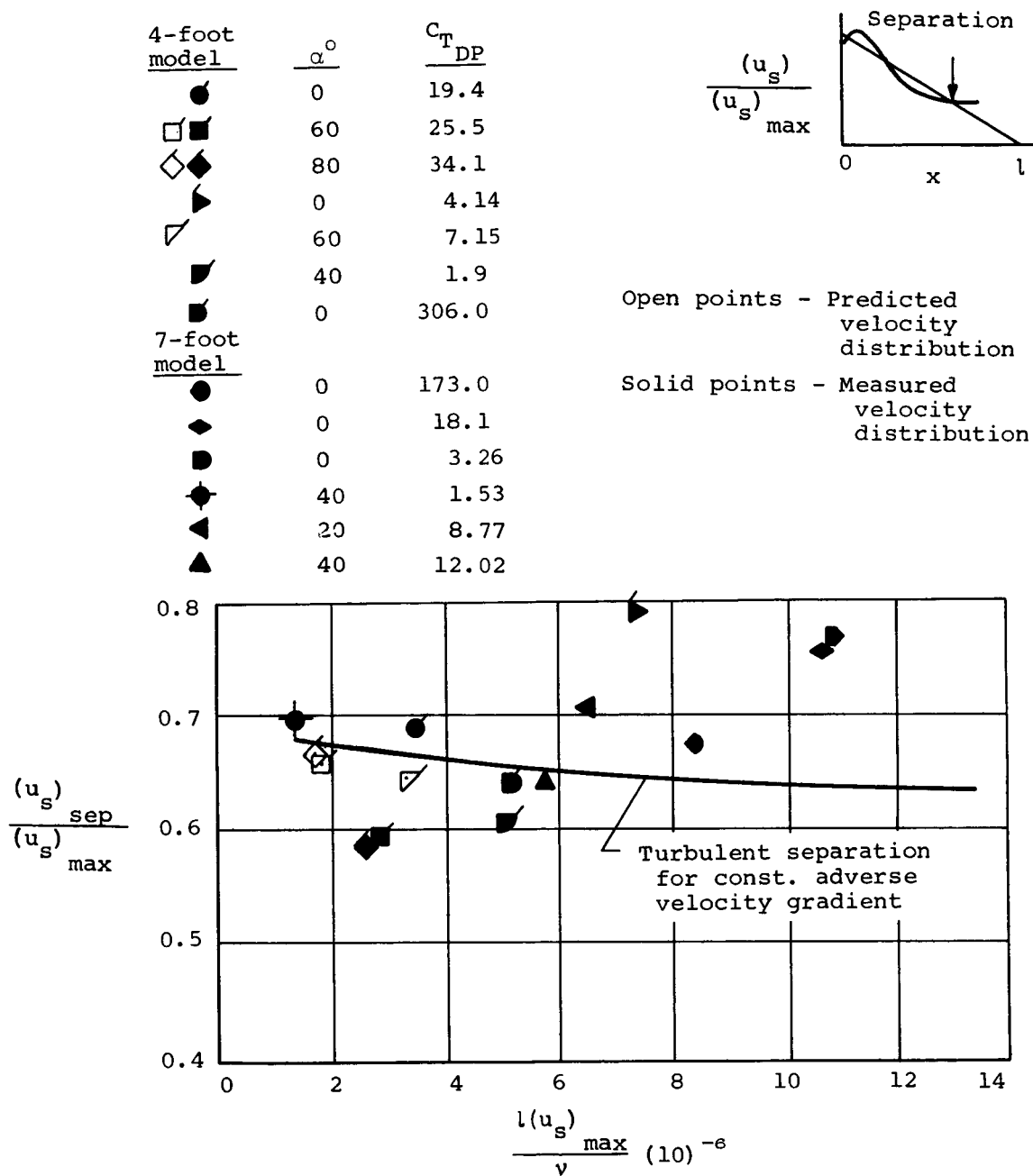
Figure 28.- Summary of computed location of separation for both ducts.
