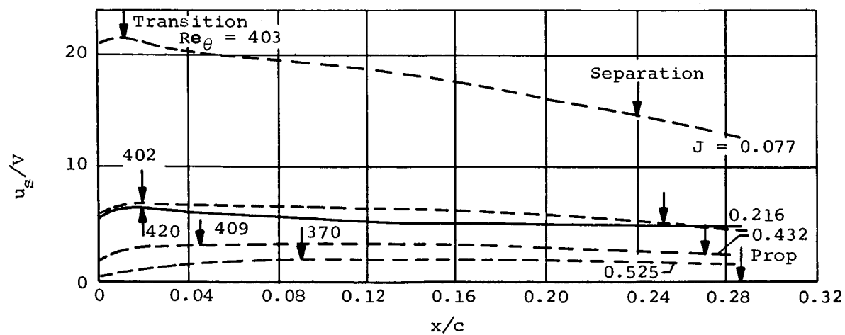
Figure 25.- Computed boundary layers for the 7-foot model duct at \alpha = 0 .
