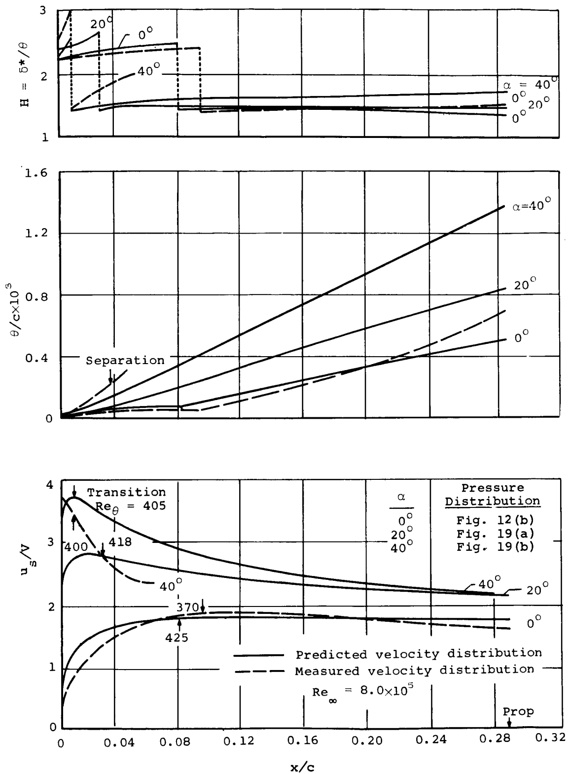
Figure 26.- Computed boundary layers for the 7-foot model duct at \alpha \geq 0 .
