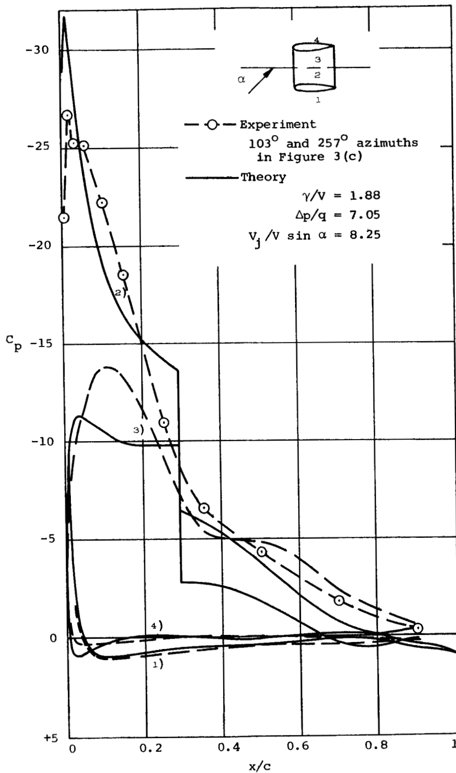
Figure 20.- Pressure distributions for the 7-foot model duct at \alpha > 0 with \beta = 19^\circ , \delta_e = 0 , J \approx 0.20 .
