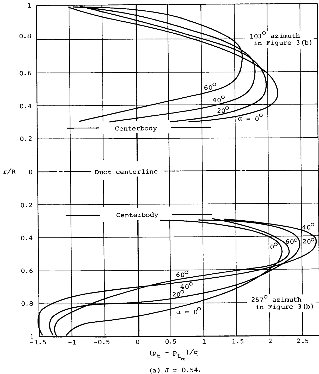
Figure 18.- Total pressure distributions measured across the exit plane of the 4-foot model duct at \alpha > 0 .
